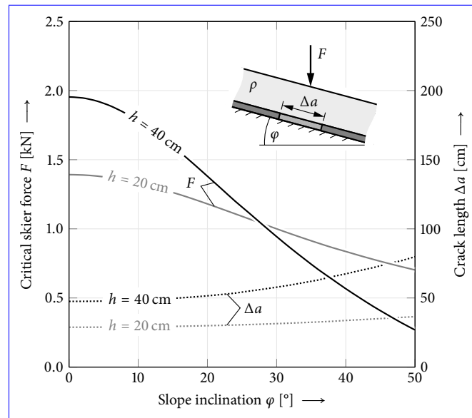
Figure 5. Effect of the slope angle \varphi on the critical additional loading F on a defect-free snowpack (solid line) and on the length of predicted initial finite anticrack \Delta a (dotted line). Steeper slopes cause a significant reduction of the critical skier loading force and a moderate increase of the crack lengths.
