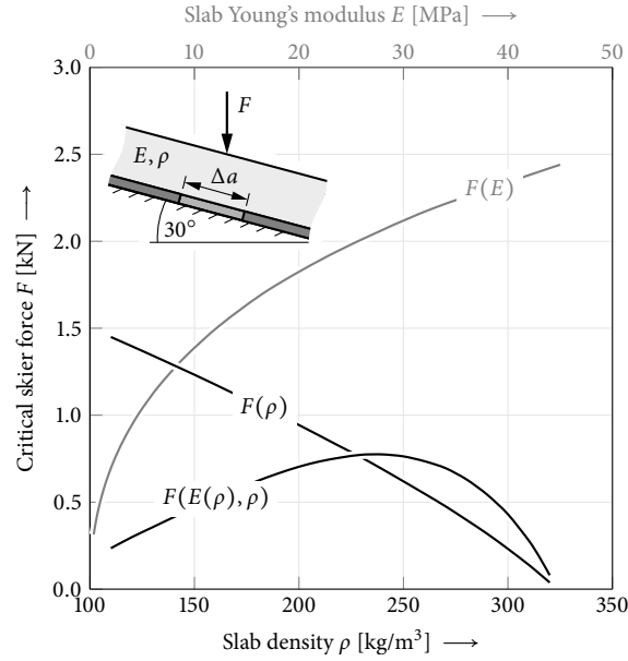
Figure 7. Effect of slab density \rho on critical additional skier loading force F of a defect-free snowpack and the corresponding length of the initiated crack \Delta a . If the slab's Young's modulus is independent of slab density, curve F(\rho) , the increasing slab weight reduces the critical skier loading force . A density-dependent Young's modulus according to Eq. (21), curve F(E(\rho), \rho) , stiffens denser slabs, which initially dominates failure and increases the critical skier load. Above a certain threshold, the weight gain becomes dominant and the critical skier loads force reduces distinctly. The size of the initiated cracks \Delta a increases with slab density.
