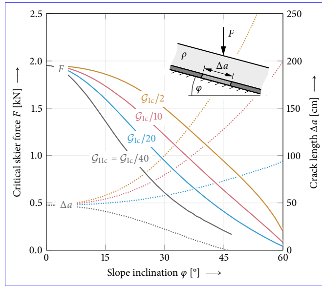
Figure 8. Comparison of mixed-mode energy criteria for a defect-free snowpack loaded by a point-load and the weight of the slab above the weak layer.
