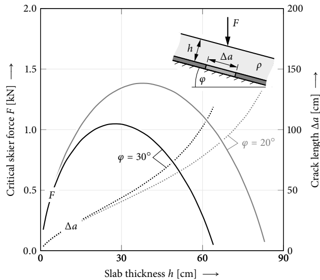
Figure 6. Critical loading of a snowpack without assumed defects and the size of initiated anticrack as a function of slab thickness. Thicker slabs transfer concentrated loads more uniformly less localized into the weak layer allowing for larger point loads. Above a certain thickness, failure is dominated by the slab's own weight reducing admissible additional loads until self-release occurs. The finite anticrack length increases continuously with increasing slab thickness.
