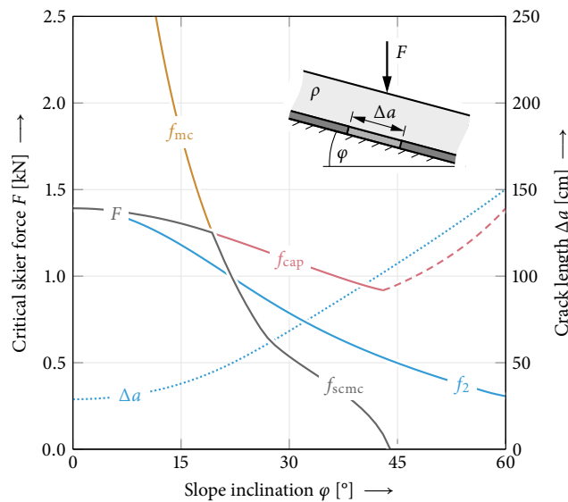
Figure 9. Comparison of mixed-mode stress criteria for a defect-free snowpack with slab thickness h = 20 cm. The quadratic interaction criterion f_2 , the smooth capped Mohr-Coulomb criterion f_{scmc} as well as its constituents f_{mc} and f_{cap} are shown.
