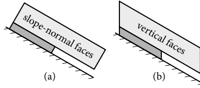
Figure 13. Boundary conditions in PST experiments: (a) slope-normal and (b) vertical upslope and downslope faces.
