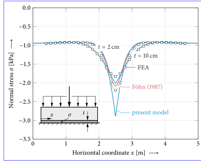
Figure 8. Effect of the weak layer thickness on local weak layer normal stresses. The weak layer thickness changes the size of the skier load affected part of the weak layer and also the peak value of the stress. Thicker, more compliant weak layer-layers distribute the load on a larger area and lead to lower peak stresses. The model-Model results (solid lines) are compared against the reference solution (markers \circ, \square ). Model parameters are chosen as given in Table 1.
