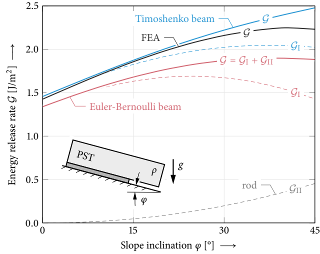
Figure 9. Total, mode I and mode II energy release rates in propagation saw tests of different slope angles \varphi with crack lengths -length a = 30 cm. Comparison of the present model using Timoshenko beam kinematics accounting shear deformation of the slab and the classical Euler-Bernoulli beam model. The latter is recovered in the limit case of infinite shear stiffness of the beam ( \kappa GA \rightarrow \infty ). Model parameters other than E_{\text{weak}} = 0.15 MPa and t = 5 cm are chosen as given in Table 1.
