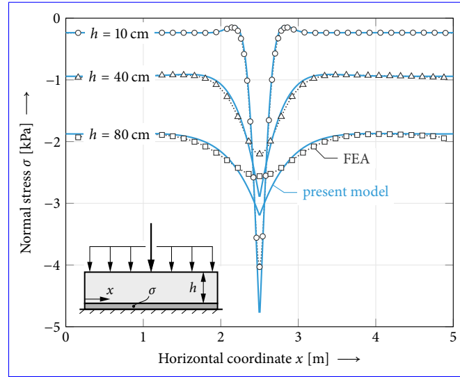
Figure 7. Bridging effect evident in weak layer normal stresses depending on the slab thickness. The peak stresses and the width of the skier loaded snow pack changes with different slab thicknesses. The model results (solid lines) are compared against the reference solution (markers \circ, \triangle, \square ). Model parameters are chosen as given in Table 1.
