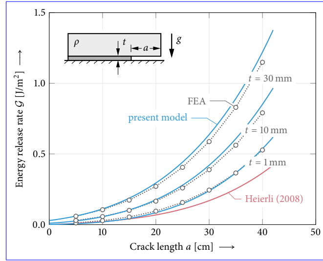
Figure 11. Energy release rate \mathcal{G} in flat terrain propagation saw tests (PST). Comparison of present model (blue lines), Heierli (2008) model (red line) and FEA results (gray circles). Both models agree well with FEA data for short crack lengths and stiff (i.e. thin) weak layers. The model by Heierli (2008) cannot reproduce varying weak layer properties providing and provides a lower bound of the energy release rate corresponding to vanishing weak layer thickness. Except for h = 30 cm and \rho = 200 model parameters are chosen as given in Table 1.
