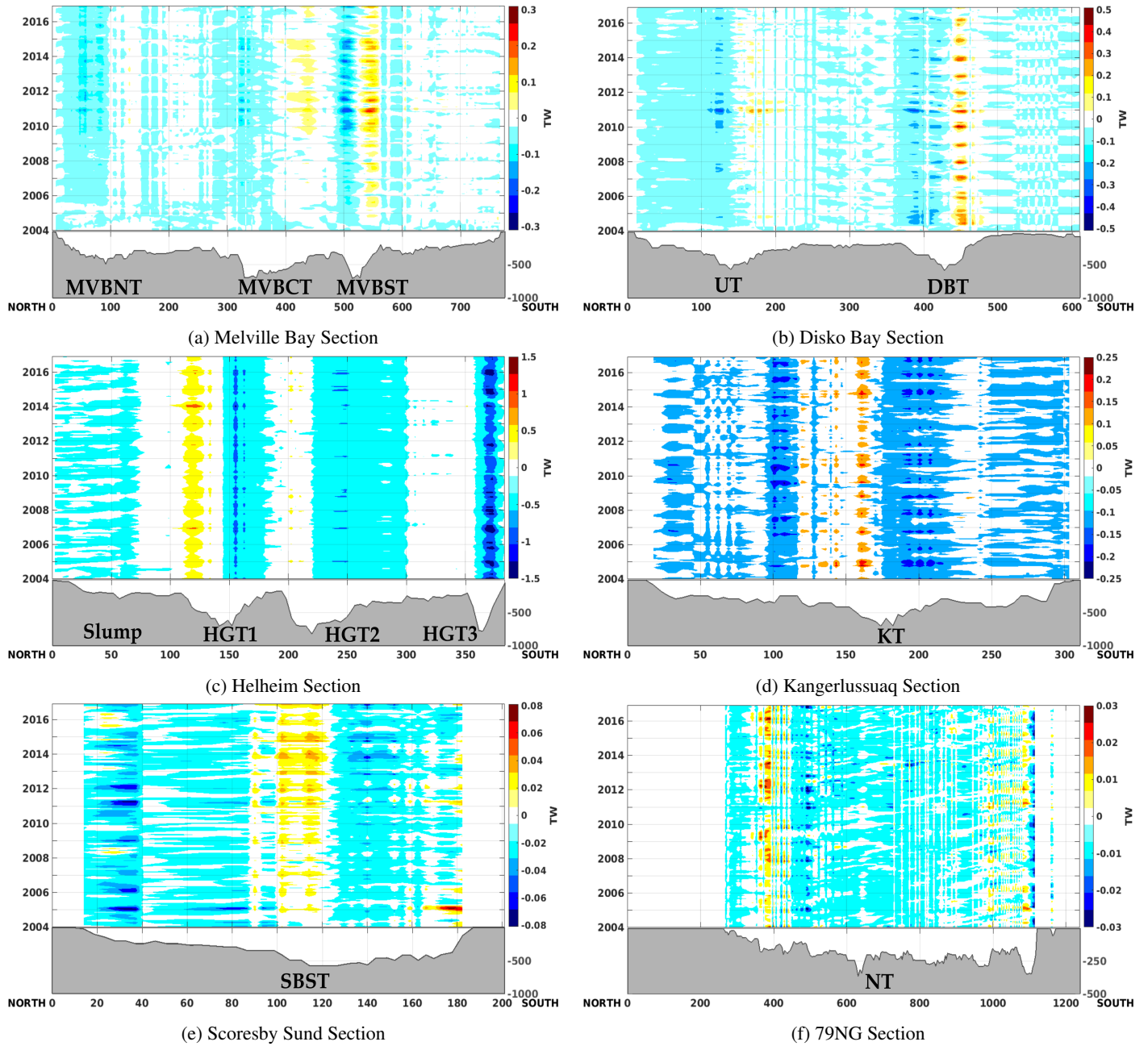
Figure 8. This figure shows the ocean heat exchange (flux) with respect to topography (in grey) within the time series of 2004 to the end of 2016 with the HighRes model output. These hovmoller plots show the monthly average heat flux coming on or off shelf in TW, (into or out of the page respectively), through a section (sections drawn in light purple on the map inset 1). Model bathymetry is in grey and the section runs north to south on the x-axis starting at the left hand side of the figure indicated by the zero kilometre marker. Along the y-axis is the depth for the bathymetry and then time for the 2004 to 2016 period. Colours indicate direction and magnitude of the on or off shelf heat flux (into and out of the page) and colourbar limits change per location .
