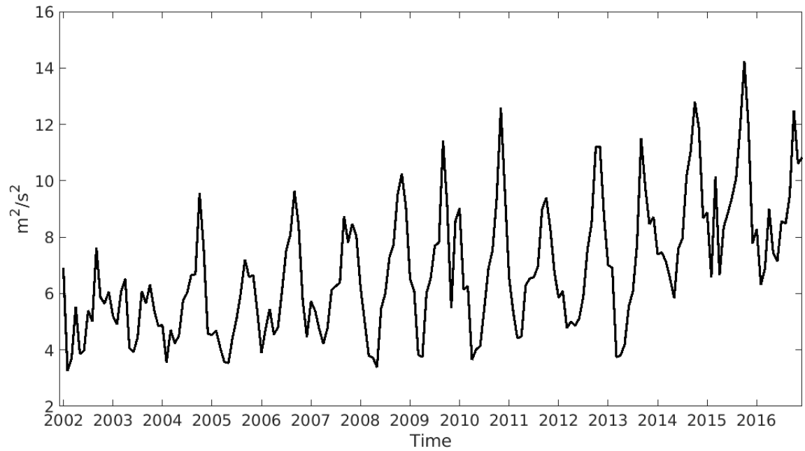
LowResControl (a)
