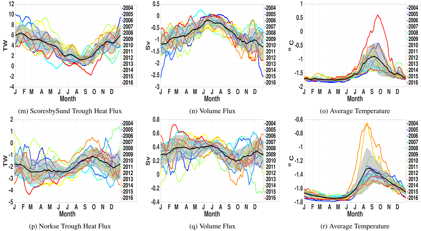
Figure 9. This figure shows the evolution and seasonality averaged through the entire depth of volume flux, heat flux through a trough and average temperature across the section of the trough. The six locations are MVBCT, DBT, HGT2, KT, SBST, and NT (indicated in Fig. 1). The months are on the x-axis and the values of heat flux in TW, on the y-axis. The moving 25 day average heat flux for 2004 to 2016 (calculated using (Eq. 2)) is shown in black with one standard deviation window in grey. The years are indicated by colour, with earlier years starting in blue to later years in red.
