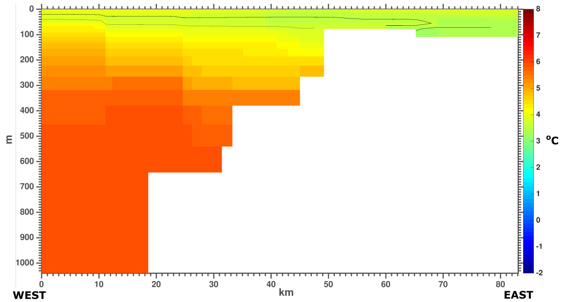
(a) LowResControl
