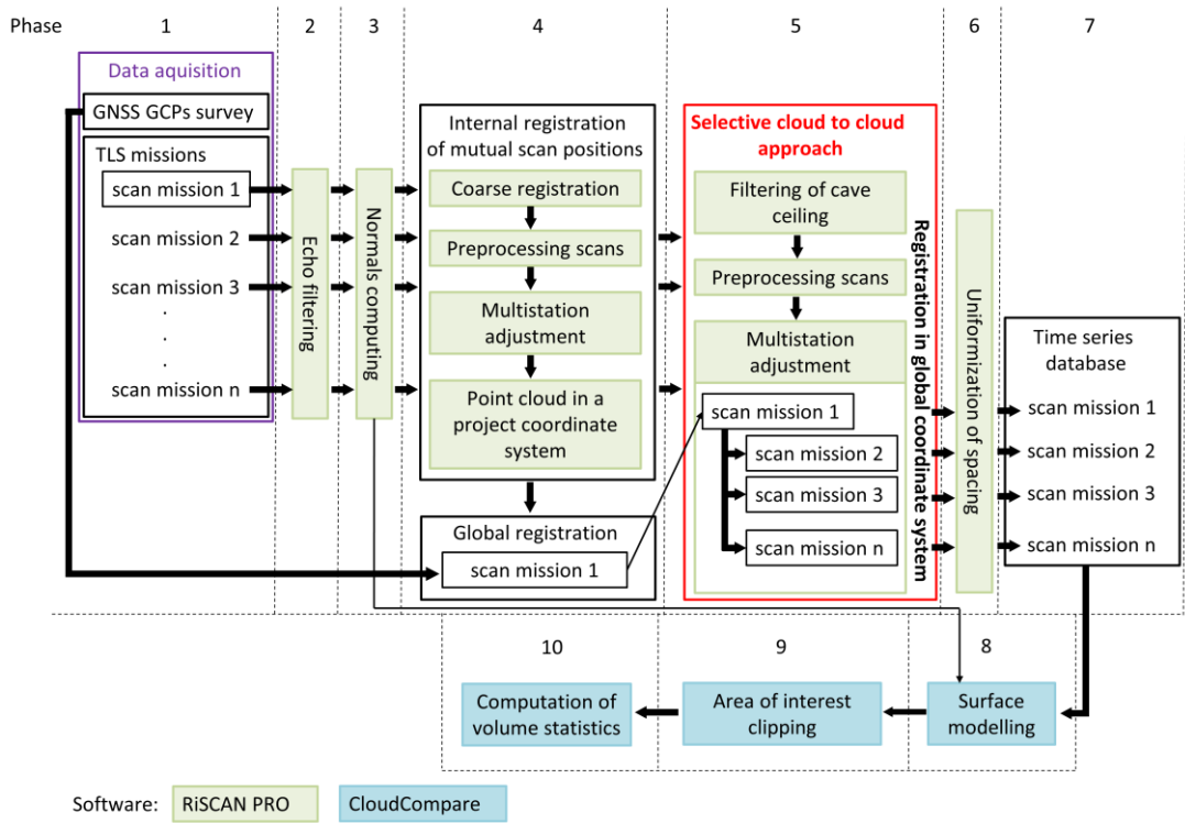
Figure 5: The workflow of generating a time-series database and framework of data processing.
