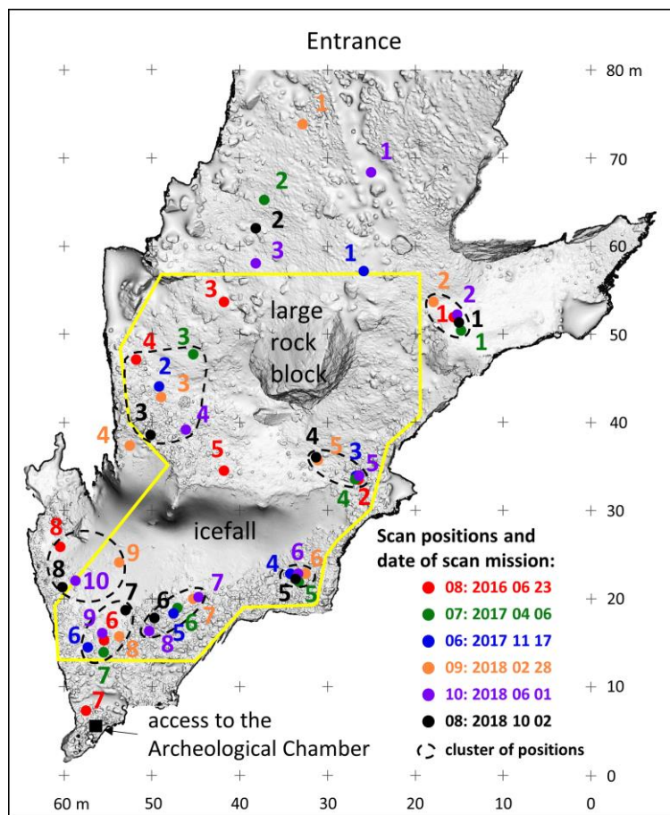
Figure 6: Distribution of scan positions of individual scan missions presented on the plan of the cave derived from TLS mapping. Yellow polygon shows defined AOI for computation of changes in ice accumulation.
