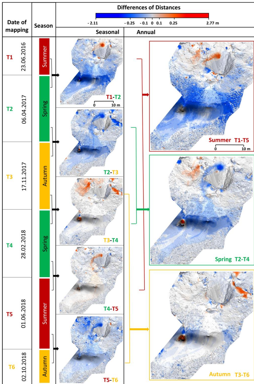
Figure 10: Differences of distances (DoD) between the individual cave floor surface models. The blue color represents decrease and red color indicates increase of the surface elevation.
