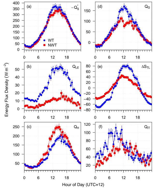
Figure 5. Comparison of diurnal variations of inverted net radiation -Q_S^* (a), latent evaporative heat flux Q_{LE} (b), sensible heat flux Q_H (c), ground heat flux Q_G (d), energy storage change in the thawed layer \Delta S_{TL} (e) and soil heat flux at ice table depth Q_{IT} (f) between WT (water track) and NWT (non-water track), averaged over the entire measuring period of 26 days. Energy fluxes for (a) and negative energy fluxes for (d) are directed towards the ground surface, energy fluxes for (b)-(d) and (f) and positive energy fluxes for (d) point away from the ground surface. Positive energy fluxes for (e) are directed from the ground surface or the ice table into the thawed layer and negative fluxes move out of the thawed layer towards the ground surface or the ice table. Error bars depict standard errors of the mean.
