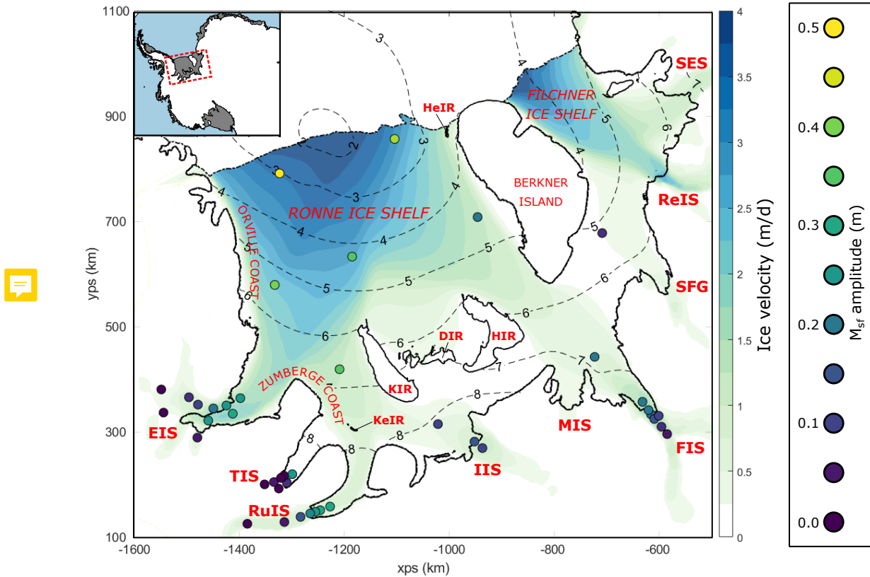
Figure 1. Map showing the Filchner-Ronne Ice Shelf and adjoining ice streams. Circular markers show locations of GPS sites and are coloured according to M_{sf} amplitude. The background colourmap shows ice speed, grounding lines are indicated by solid black lines, dashed contour lines show tidal range (in meters) and solid gray contour lines show ice surface elevation. Acronyms for glaciological features marked on the map are as follows: Evans Ice Stream (EIS), Talutis Ice Stream (TIS), Rutherford Ice Stream (RuIS), Institute Ice Stream (IIS), Moller Ice Stream (MIS), Foundation Ice Stream (FIS), Support Force Glacier (SFG), Recovery Ice Stream (ReIS), Slessor Ice Stream (SES), Hemmen Ice Rise (HeIR), Korff Ice Rise (KIR), Kershaw Ice Rumples (KeIR), Doake Ice Rumples (DIR) and Henry Ice Rise (HIR).
