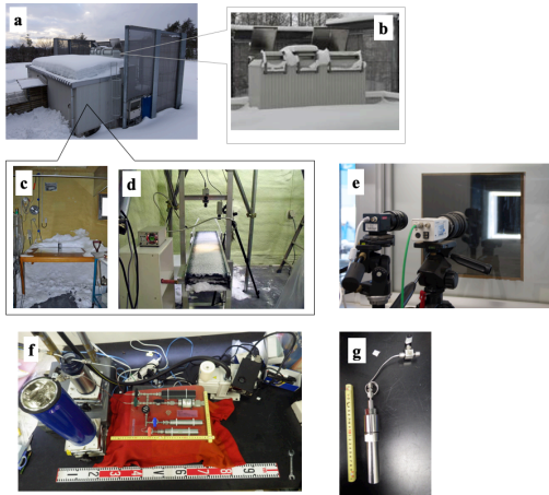
Fig.1. Falling Snow Observatory (FSO) and the device developed for the methane adsorption method at the SIRC
