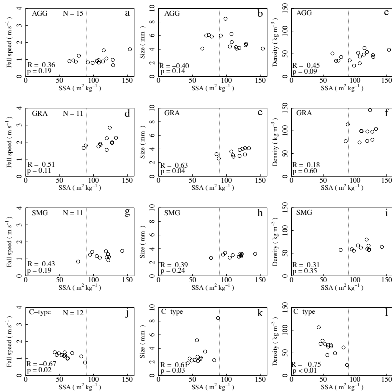
Fig. 12. Relationship between SSA of freshly fallen snow and detailed characteristics of falling snow produced by the CMF. a, b, c: data of aggregate group events in M-type (AGG) d, e, f: data of graupel type events in M-type (GRA) g, h, i: data of small particle type events in M-type (SMG) j, k, l: data in C-type (C-type) N: sample number, R: correlation coefficient, and p: p values Dotted lines indicate SSA value of 90 m 2 kg -1
