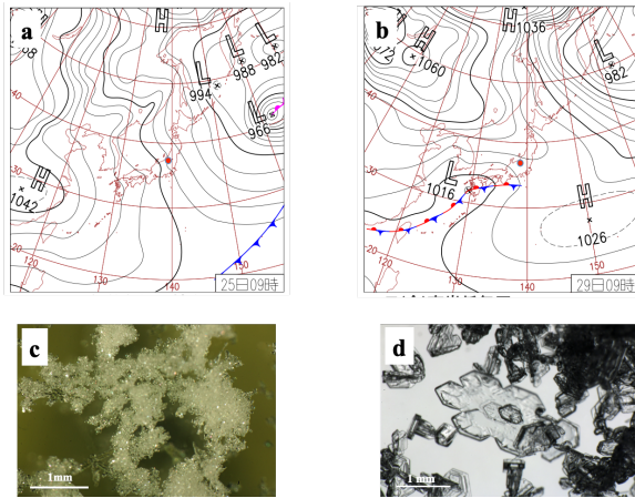
Fig. 5. Synoptic atmospheric pressure condition of falling snow events in Nagaoka. Red circles indicate the location of Nagaoka.
