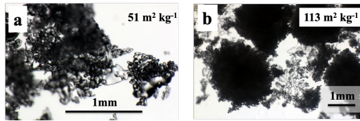
Fig. 4. Microphotographs of samples taken under melt events
