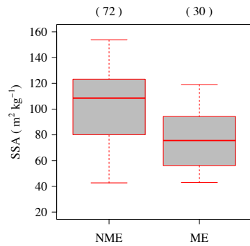
Fig. 3. Wet-bulb temperature ( T_w )-melting-based classification of SSA data classification
