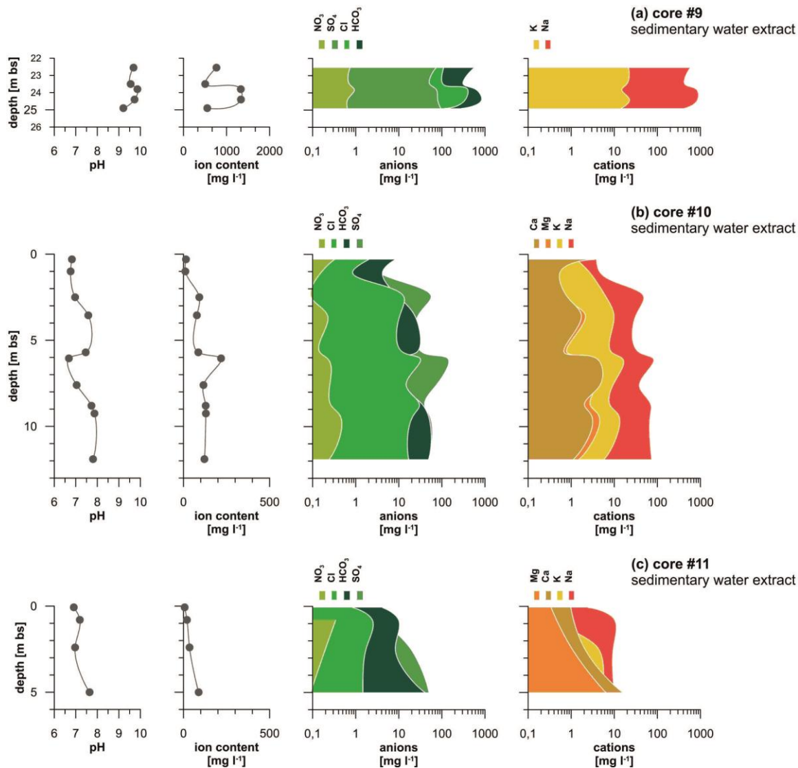
Figure 4: Hydrochemical composition of water extracts from the sedimentary cores #9, #10 and #11. Data are given in Table 3. Note different axis scale for ion content in (a) reaching up to 1335mg l -1 .
