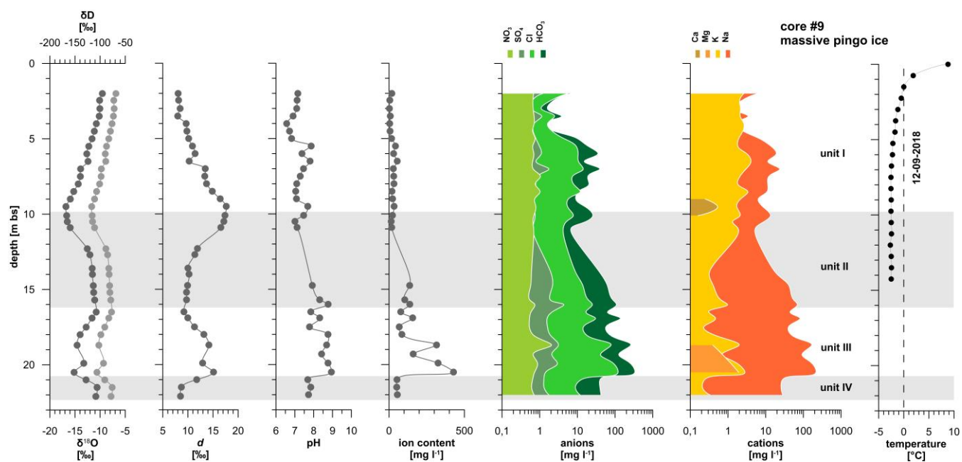
5 Figure 2: Isotopic and hydrochemical composition of the massive ice of Filipingo obtained from core #9 as well as thermometric data from the borehole on 12 September 2018. Light grey symbols in the first plot refer to the upper x-axis ( \delta D ). Data are given in Table 1 and Table 2.
