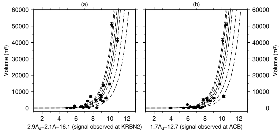
Figure E1. Best performing GLMs for KRBN2 and ACB. Symbols show calibration data from lidar measurements with error bars. Solid curve represents the fitted model. Dashed lines show deviations of \pm 20\% , 50\% and 70\% for a given volume. A_d is the logarithm of envelope amplitude integrated over calving signal duration and A the logarithm of maximum envelope amplitude.
