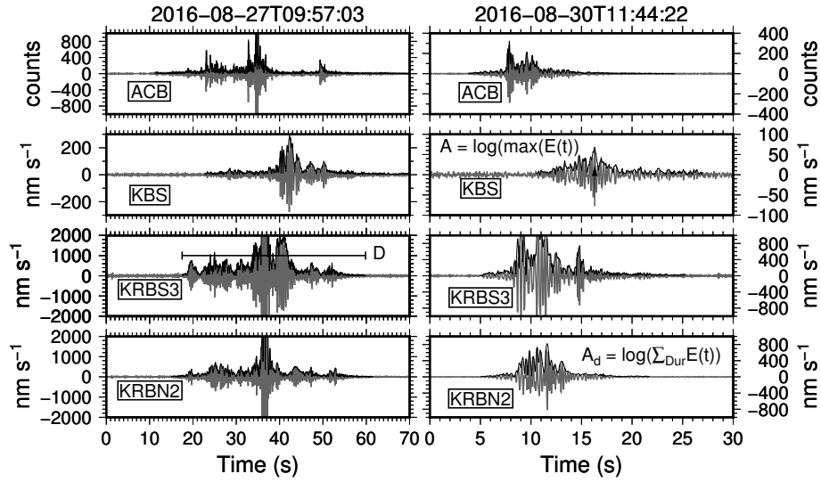
Figure 2. Examples of hydroacoustic (ACB) and seismic (KBS, KRBN2, KRBS3) signals of two calving events. Waveforms bandpass-filtered between 2 and 12 Hz are shown in gray. Black curves are signal envelopes ( E(t) ) used to compute the event features: signal duration ( D ), logarithm of envelope amplitude integrated over event duration ( A_d ), and logarithm of maximum envelope amplitude ( A ). Note, that for hydroacoustic data the raw digitizer output is processed (counts).
