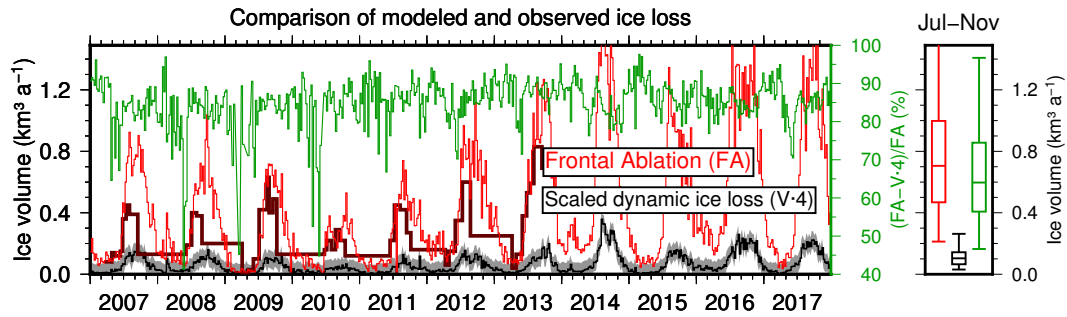
Figure 7. Comparison of frontal ablation rates at Kronebreen directly measured with satellite remote sensing between 2007 and 2013 (dark red) and modeled in Köhler et al. (2016) from seismic KBS data with weekly resolution (red). Scaled dynamic ice loss rates modeled in this study from KBS record and taking into account an average dynamic ice loss detection rate of 25% at KBS are shown in black with gray area indicating uncertainty (two times standard deviation estimated in 2016 calibration period, Table 1). Green curve is percentage of total frontal ablation not explained by modeled dynamic ice loss. Right panels-panel shows box plot-plots for calving season (2%, 25%, 98%, and 75% quantiles) using difference (FA-4·V) instead of percentage.
