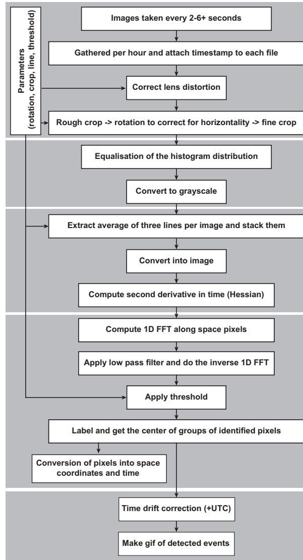
Figure B1. Workflow for detecting calving events in the time-lapse image data.
