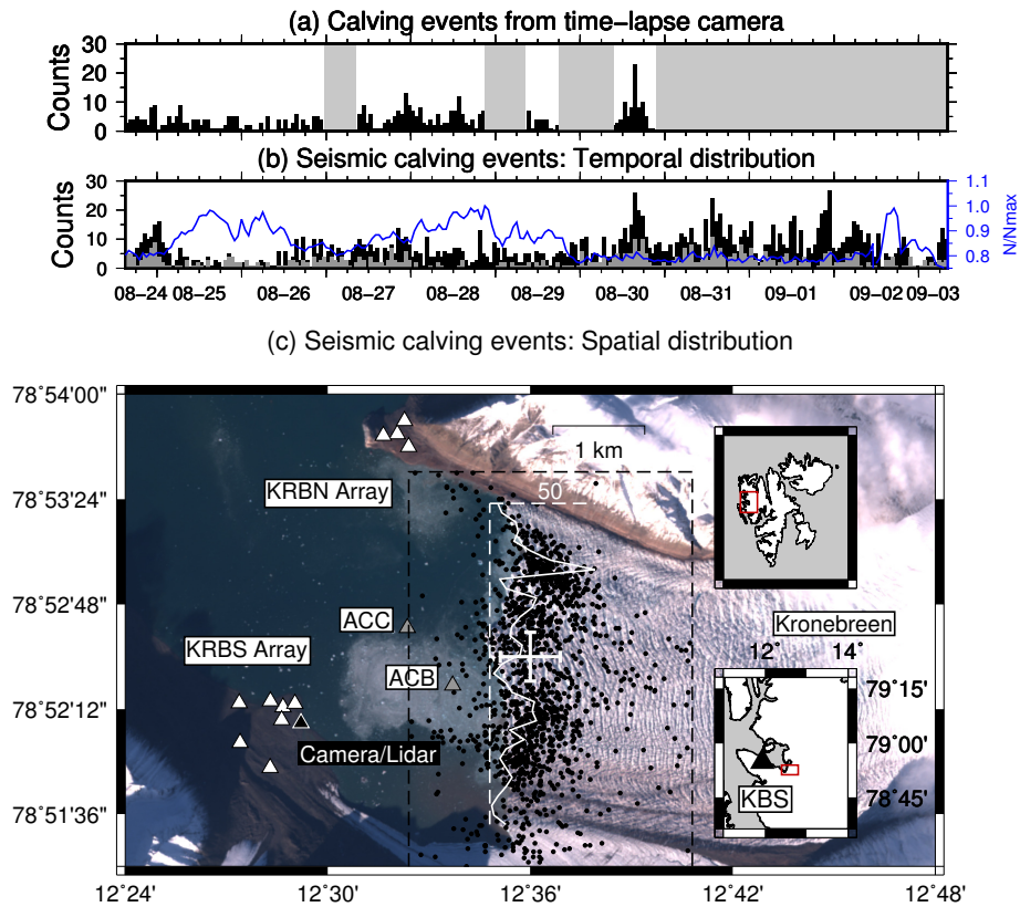
Figure 1. Calving event time series and location. (a) Hourly counts of calving events automatically detected on time-lapse camera images. Grey-Gray areas indicate image gaps. (b) Hourly counts of seismic detections simultaneously at KRBN and KRBS (black) and at KBS (gray). Blue line shows relative variations in seismic background noise level (N) with respect to maximum level (Nmax) in recording period. (c) Triangles show locations of time-lapse camera (black), Lidar scanner (black), seismic (white), and hydroacoustic (gray) instruments at the calving front of Kronebreen. Black points are seismic calving event locations. White error bars show an estimate of the typical location uncertainty. White curve is histogram of time-lapse camera event counts projected on a line (dashed) parallel to the terminus. Dashed box is used to classify located seismic signals as calving events. Insets to the right show Arctic archipelago of Svalbard (upper) and a closeup map of Kongsfjorden area (lower) with location of permanent broadband seismometer KBS in Ny-Ålesund.
