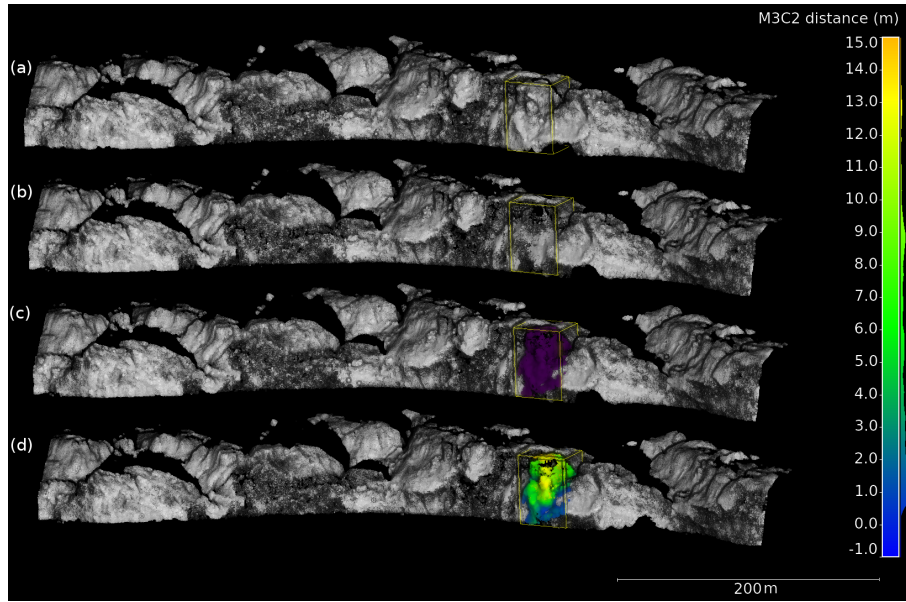
Figure A1. Lidar DSM differencing for a calving event on 2016-08-27T09:57:03 (a) point cloud before the event, (b) point cloud after the event, (c) area of the calving event, (d) calving event depth computed with M3C2 plugin (Lague et al., 2013). A histogram of computed depths is located to the right of the color bar and the calculated calving event volume V is 7046.6 \pm 632.3 \text{ m}^3 . The region of interest is marked with a yellow bounding box and the lidar reflection intensity is shown in grayscale on each point cloud (a-d).
