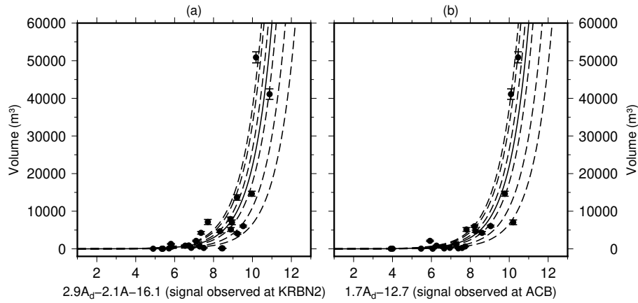
Figure E1. Best performing GLMs for KRB2 and ACB. Symbols show calibration data from lidar measurements with error bars . Solid line-curve is fitted model. Dashed line show deviations of \pm 20\% , 50\% and 70\% for a given volume. A d is logarithm of envelope amplitude integrated over calving signal duration and A logarithm of maximum envelope amplitude.
