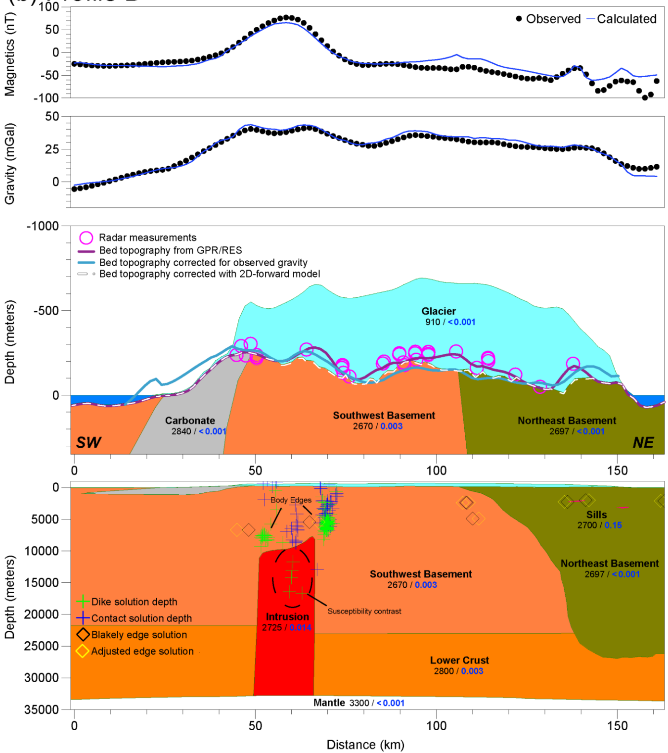
Figure 5: Profile A (a) and profile B (b), near-surface view of the basement (top) and depth to mantle (bottom) with Werner deconvolution indicators of the intrusions and the basements interface. A gravity response (purple) is calculated for a homogeneous bedrock using GPR/RES bed topography. The misfit with the observed gravity suggests the bedrock is heterogeneous and the bed topography from the radar needs refining. The gravity corrected bed topography provides improvement but fails to recognize the heterogeneity of the bed. The 2D-forward model improves the accuracy of the bed topography by using a density more representative of the lithology. Each polygon representing a geological body is characterized with a density ( \text{kg m}^{-3} ; black) and a susceptibility (SI units; blue).
