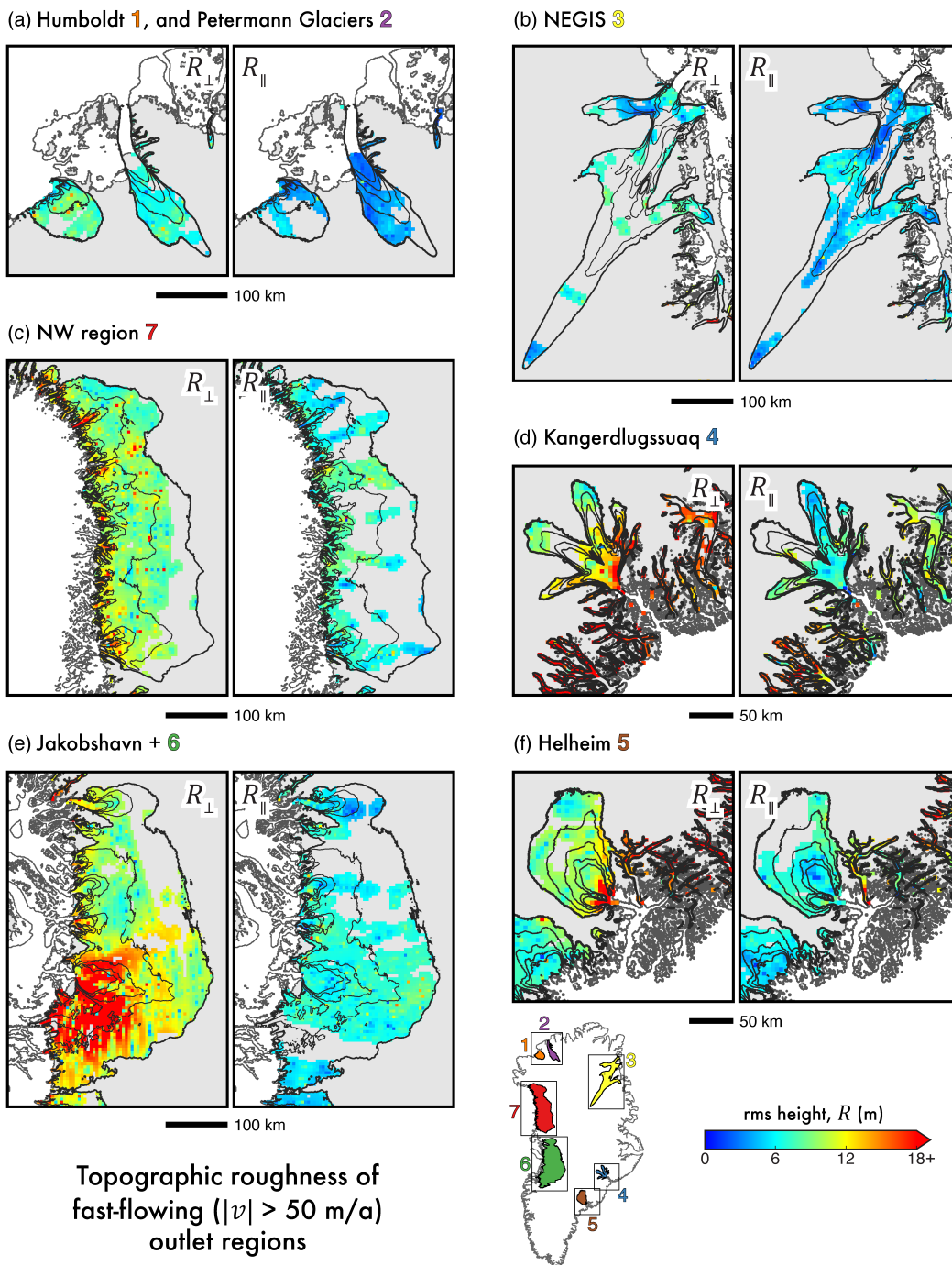
Figure 9. Local subsets of R_{\perp} and R_{\parallel} in fast-flowing outlet glacier regions. Interpolated R_{\perp} and R_{\parallel} (as Fig. 5) is shown for the fast-flowing regions of: (a) Humboldt [1] and Petermann [2] glaciers; (b) the North East Greenland Ice Stream (NEGIS) [3]; (c) the North West (NW) [7] fast-flow region; (d) Kangerdlugssuaq [4]; (e) Jakobshavn Isbrae and surrounding glaciers [6]; and (f) Helheim [5]. The location of these regions is inset, where regions are colour-coded for further analysis (see Figure 10).
