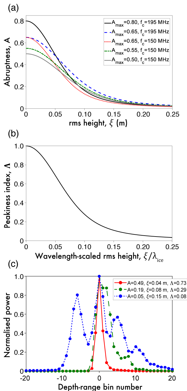
Figure 4. Estimation of scattering-derived roughness and data combination for bed-echo peakiness. (a) Abruptness as a function of rms height for different CRE SIS field seasons: solid black curve, 2010 DC8; long dashed blue curve, 2011 TO, 2011 P3, 2012 P3, 2013 P3 and 2014 P3; dotted red curve, 2006 TO; tray-dashed green curve, 2005 TO; solid grey curve, 2008 TO and 2009 TO. (b) Peakiness Index as a function of wavelength-scaled rms height. (c) Example bed-echo waveforms, their abruptness, A , peakiness-index, \Lambda , and scattering-derived roughness, \xi . The plots are for the 2011 P3 field season which has maximum A \sim 0.65 .
