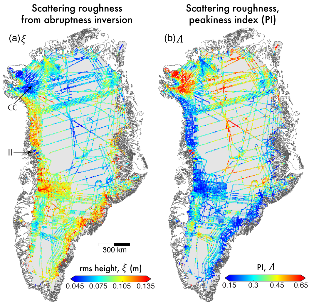
Figure 6. Scattering-derived roughness ( \xi ) across the GrIS. (a) \xi . (b) Non-dimensional \Lambda (peakiness index) determined from the bed-echo waveform. Locations for Inia Isbrae (II) and Camp Century (CC) drilling site are marked.
