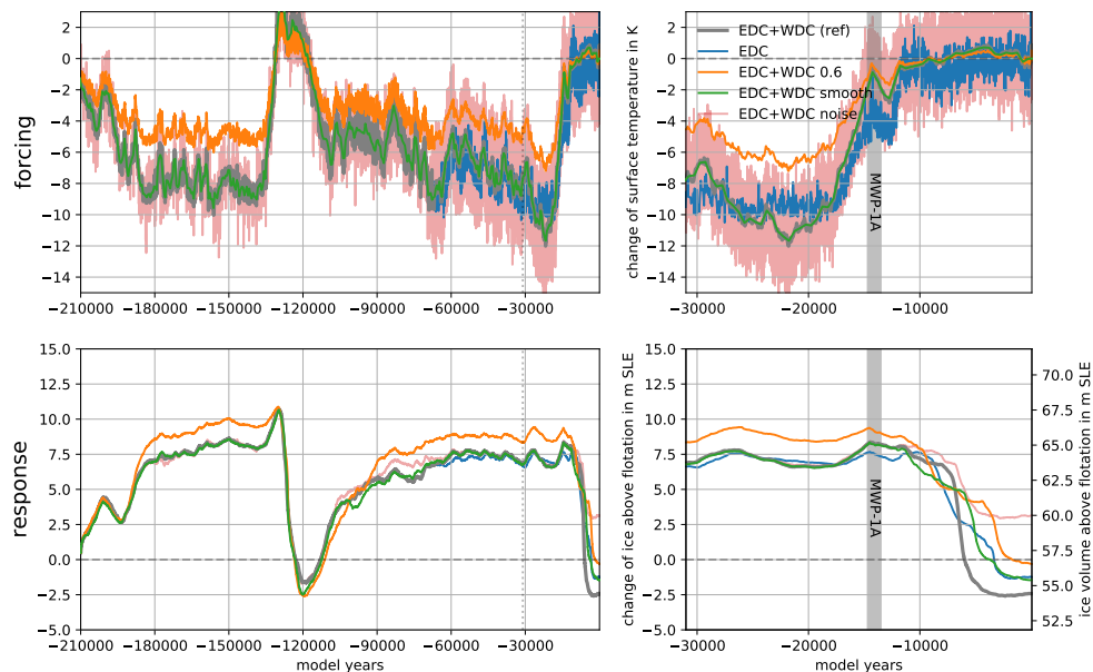
Fig. 1. Timeseries of PISM-simulated ice volume above flotation relative to observations over last 210 kyr forced with five different surface temperature reconstructions (added to Figure 19).
