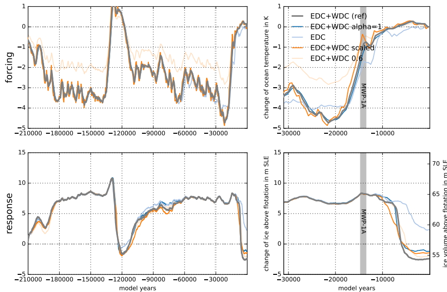
Figure 22: Sensitivity of transient ice volume above flotation to varied ocean temperature forcing. Reference simulation (grey) is based on EDC+WDC surface temperature with fit response function of power \alpha = 2 . The resulting ice volume change is similar for a fit response function with power \alpha = 1 (blue). Even if ocean temperature forcing responds immediately directly to the scaled surface temperature anomalies-anomaly (orange) the resulting effects on ice volume are comparably small. If a different surface temperature reconstructions-are-reconstruction is used, here from EDC with \alpha = 2 (light blue), we find for in response to a later warming signal a delayed deglaciation accordingly . If the amplitude of WDC surface temperature anomalies was 40% lower (light orange), this would have only negligible effect on the modeled ice volume.
