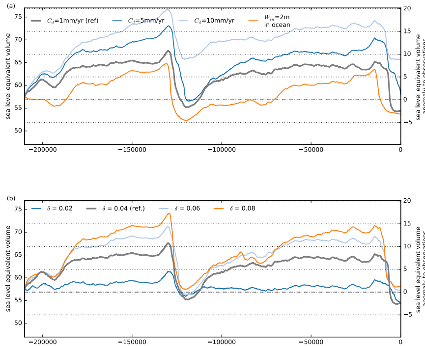
Figure 17: (a) Simulation over two glacial cycles for different till water decay rates (a) and for different fractions of the overburden pressure (b) underneath the grounded ice sheet. (a) Higher values decay rates than the reference value of C_d = 1 \text{ mm/yr} (grey) cause less extended ice streams, less ice discharge and hence thicker ice sheets (blue and light blue). If we assume When assuming maximum till water fraction across ocean beds, grounding line advance of marine glaciers is decelerated. Accordingly, we find a less extended and thinner ice sheet at glacial periods, earlier retreat but similar present-day results (compare grey and orange lines). (b) The critical fraction of the effective overburden pressure \delta in Eq. has strong influence on the reconstructed ice volume, particularly at glacial maximum, with high parameter values leading to more friction and hence thicker ice sheets. For the evaluated range of 2–8% we find up to 12 m SLE difference in the ice volume above flotation.
