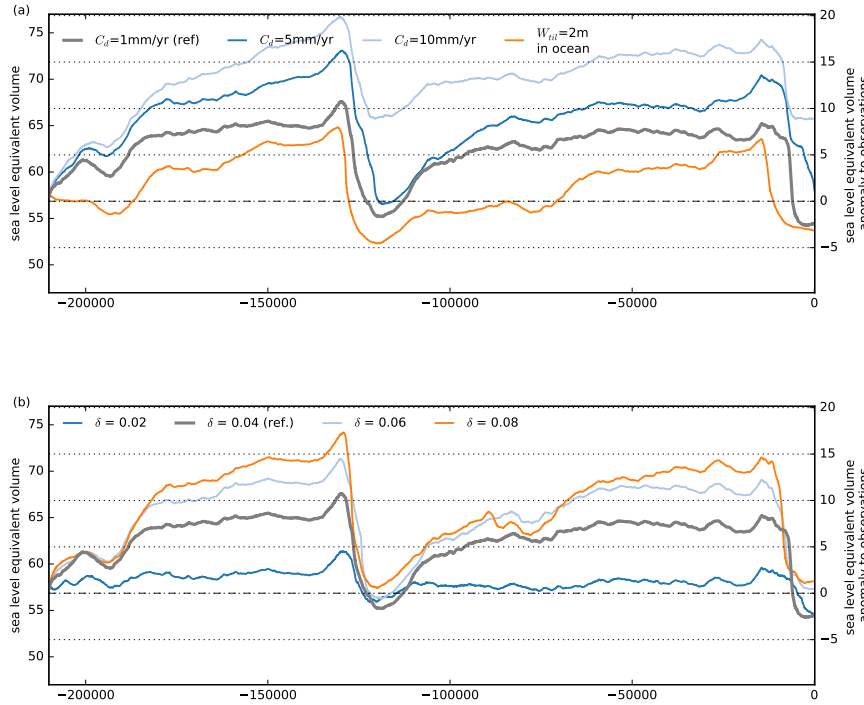
Figure 17: (a) Simulation over two glacial cycles for different till water decay rates (a) and for dif- ferent fractions of the overburden pressure (b) underneath the grounded ice sheet. (a) Higher values decay rates than the reference value of C_d = 1 mm/yr (grey) cause less extended ice streams, less ice discharge and hence thicker ice sheets (blue and light blue). If we assume When assuming maximum till water fraction across ocean beds, grounding line advance of marine glaciers is decelerated. Ac- cordingly, we find a less extended and thinner ice sheet at glacial periods, earlier retreat but similar present-day results (compare grey and orange lines). (b) The critical fraction of the effective over- burden pressure \delta in Eq. has strong influence on the reconstructed ice volume, particularly at glacial maximum, with high parameter values leading to more friction and hence thicker ice sheets. For the evaluated range of 2–8% we find up to 12 m SLE difference in the ice volume above flotation.
