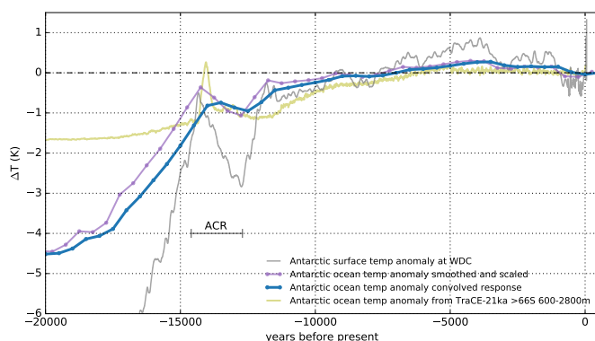
Figure 21: Response of the intermediate ocean temperature (blue) to surface temperature anomaly, as reconstructed from WDC (Cuffey et al., 2016, grey line) assuming a polar amplification factor of 1.8 and an equilibrium ocean scale factor of 0.75, as identified in climate model analysis for a warming scenario. Convolution yields a delayed response (blue) with respect to the forcing, here shown as scaled curve (compare violet and blue curve). Dots indicate, with dots indicating bins of 500 year means. The timeseries includes the Antarctic Cold Reversal (ACR) 14.6-12.7 kyr BP (Fogwill et al., 2017). For comparison, GCM ocean temperature anomaly is shown (in olive), as reconstructed by TraCE-21ka (Liu et al., 2009), for the mid-ocean depth 600-2,800m depth and south of 66°S.
