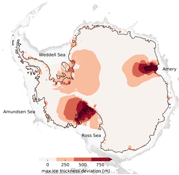
Figure 2: Maximum difference in present-day ice thickness of three simulations of the Antarctic Ice Sheet after three rounds of two-glacial-cycle simulations with identical model settings, but for different initial enthalpy states (cf. final state in Fig. 1). In particular the Siple Coast (Ross) and Amery trough shows more than 1 km difference in ice thickness between the final states.
