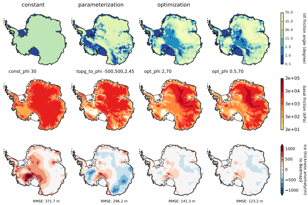
Figure 14: PISM equilibrium simulations for different basal friction fields ( \tau_c in middle row) based on different till friction angle distributions ( \phi in first row). First column with spatially uniform till friction angle of 30^\circ , second column show till friction angle according to PISM parameterization as function of bed topography, last columns using a simple inversion technique with different minimal \phi_{i_{min}} . Last row shows the resulting ice thickness anomaly to Bedmap2 observations (Fretwell et al., 2013) with improvements particularly in East Antarctica and Siple Coast region and overall RMSE reduced to 123 m (with parameters ESIA=1 and C_d = 5 mm/yr).
