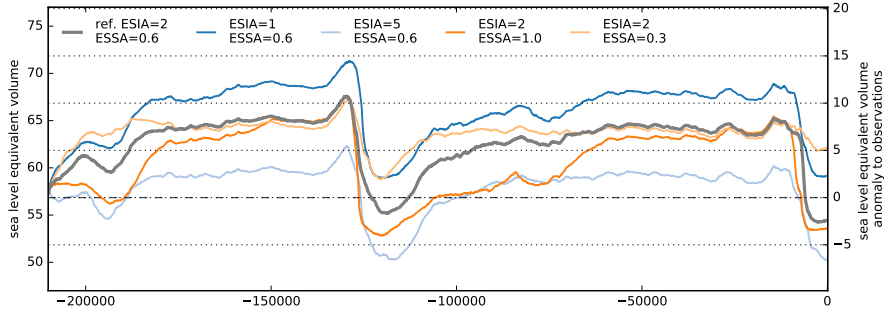
Figure 3: Ice volume above flotation for simulations over the last two glacial cycles with varied enhancement factors for SIA and SSA stress balance. Lower E_{SIA} lead to thicker grounded ice sheets, while larger E_{SSA} cause faster deglaciation and slightly thinner modern ice sheets.
