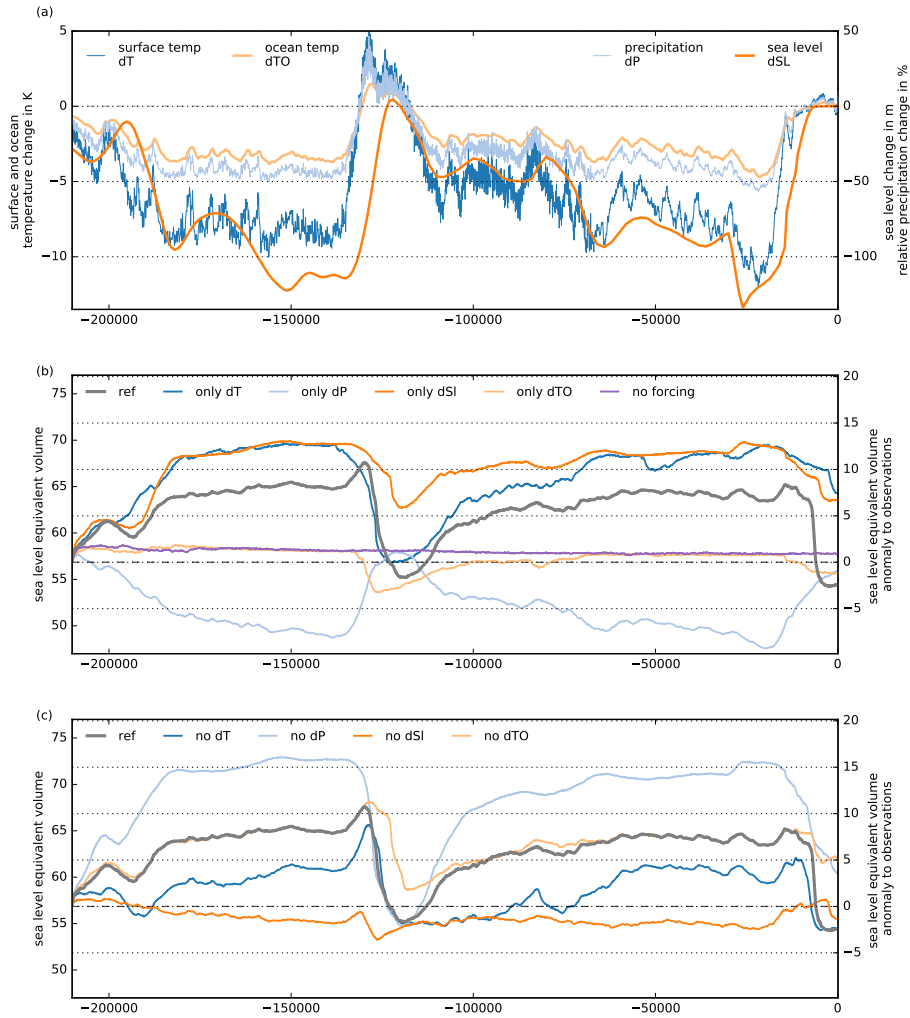
Figure 24: Antarctic Ice Sheet volume above flotation for combination-combinations of surface temperature, ocean temperature, sea-level and precipitation forcings ( upper-panel ), as defined in previous sections. Middle-panel shows the (b) The ice sheet's response to individual forcings (or constant equilibrium conditions in purple) , while-or (c) in lower-panel the absence of one forcing is switched off of the forcings, compared to the reference simulation (with all forcings combined, in grey). Sea-level forcing (orange) and surface temperature forcing (blue) have the strongest effects: each alone can cause larger glacial ice volume than in the reference simulation. Yet, each alone cannot initiate effective glacial retreat during modern climate. In contrast, ocean temperature forcing (light orange) has no effect on glacial volume but it amplifies deglaciation. Precipitation forcing (light blue) counteracts sea-level and temperature forcings at glacial climates.
