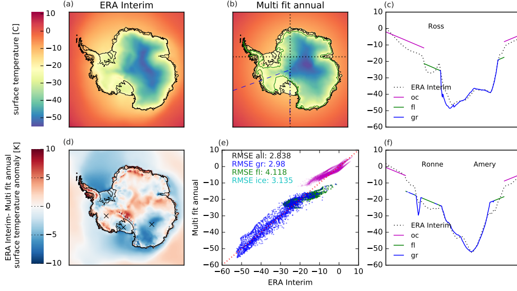
Figure 8: Comparison of ERA Interim annual mean temperatures (a) with multiple regression fit (b) according to Eq. (9), with 110^\circ\text{W} -longitude indicated as blue-dashed line, the 1000 m surface height isoline in green and the black-dotted transects through the large ice shelf regions. Inner parts of the West Antarctic Ice Sheet are less than 1 K too cold (d), while temperatures in the shallow ice shelves of Ross and Ronne are overestimated by up to 5 K (cf. panels (c) and (f)). Root-mean-square-errors of temperatures in grounded and floating ice sheet regions are 3.0 K and 4.1 K respectively (e).
