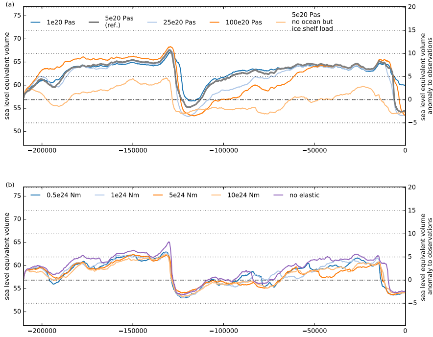
Figure 7: Simulations over two last glacial cycles with varying Earth model parameters for the viscous (a) and the elastic part (b). Mantle viscosities with a range over two orders of magnitude cause slower ice sheet growth but faster decay for increasing viscosity. Tested (b) The tested flexural rigidity over a ranges-range of more than one order of magnitude yields smaller difference in simulated ice volume response, but increased variability. Be aware that for the lower panel a different PISM v1.1 has been used, with a fixed elastic model, but only accounting for changes in grounded ice loads, explaining generally lower glacial volumes than in the reference in the upper panel.
