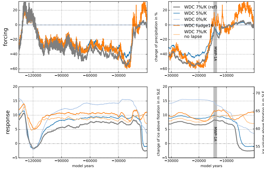
Figure 23: Sensitivity of transient ice volume above flotation to varied precipitation forcing. Grey curve is the reference with an exponential scaling factor of 7\% \text{ K}^{-1} with respect to WDC temperature reconstruction (Cuffey et al., 2016). Ice volume is slightly larger for 5\% \text{ K}^{-1} (blue) and much larger without precipitation forcing (light blue). Deglaciation is prohibited when using WDC accumulation reconstruction (Fudge et al., 2016) with additional accumulation during Holocene (orange). A similar effect reveals is seen when no lapse rate correction is applied for the precipitation (light orange).
