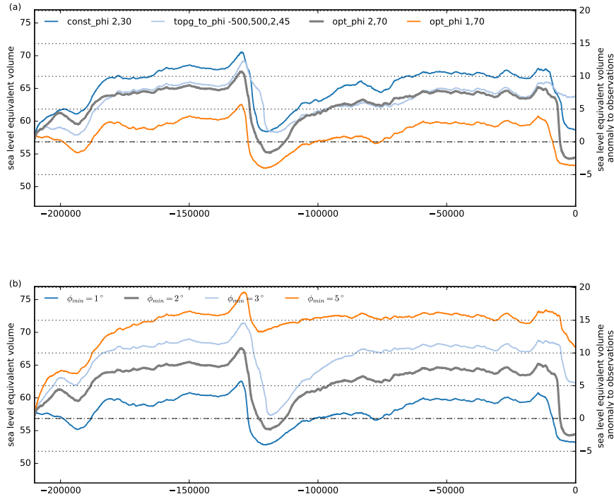
Figure 15: Ice volume histories over two glacial cycles for different parameterizations of till friction angle. (a) For a spatially uniform \phi (with 30^\circ in grounded ice and 2^\circ elsewhere, blue) and \phi according to PISM parameterization a till friction angle that is parameterized as function of the bed topography (light blue), the simulated ice volumes are generally larger than for the reference \phi (grey), as where \phi is a result of the simple inversion technique, all with. In those three cases the same minimal \phi_{\min} was used. For a smaller \phi_{\min} = 1^\circ we find generally smaller ice volumes. (b) The choice of \phi_{\min} has strong influence on the reconstructed ice volume, with high till friction angles leading to more friction and hence thicker ice sheets. Within the plausible range from 1.0^\circ – 5.0^\circ we find up to 18 m SLE difference in ice volume above flotation.
