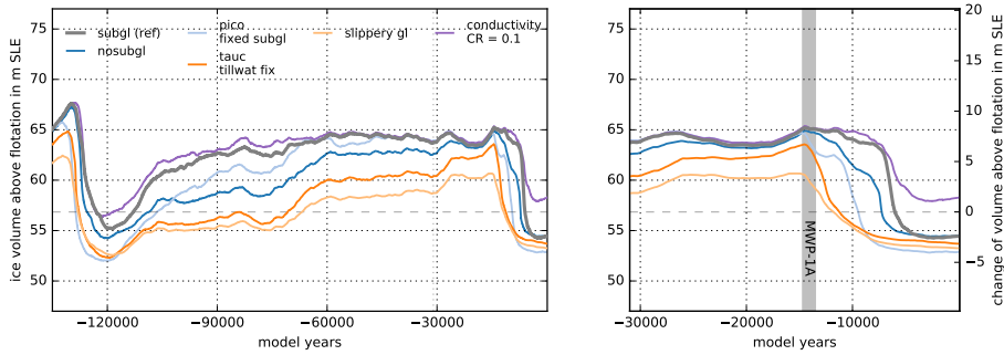
Figure A.2: Sensitivity of transient ice volume above flotation to varied conditions at the grounding line. Grey curve is the reference with applied sub-grid basal shear stress and old basal melt interpolation, which generally underestimates melting at the grounding line. Without basal melt interpolation (blue) or with fixed basal melt interpolation (light blue), deglaciation occurs hence earlier than in the reference, while glacial maximum extent is comparable. Glacial ice sheet growth is even slower for enforced saturated till conditions along the marine sections of the grounding line, landward (orange) or on the ocean side of the grounding line (light orange). The much higher sensitivity of the ice sheet volume to oceanic forcing yields a smaller glacial ice volume and much earlier deglaciation. The effect of variation of the temperate ice conductivity ratio over four orders of magnitude has only little effect, with slightly larger interglacial ice volumes for larger ratios (purple).
