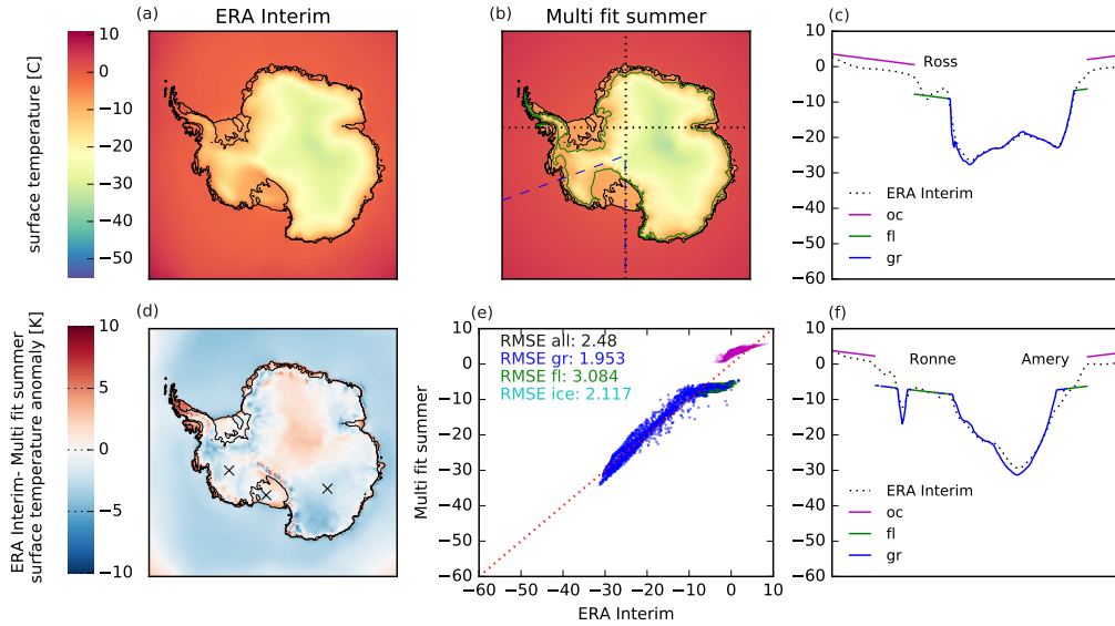
Figure 9: Comparison of ERA Interim summer (January) mean temperatures with parameterization of Eq. (10). Root-mean-square-errors of temperatures in grounded and floating ice sheet regions are 2.0 K and 3.1 K respectively, with temperatures in the large ice shelves close to observations.
