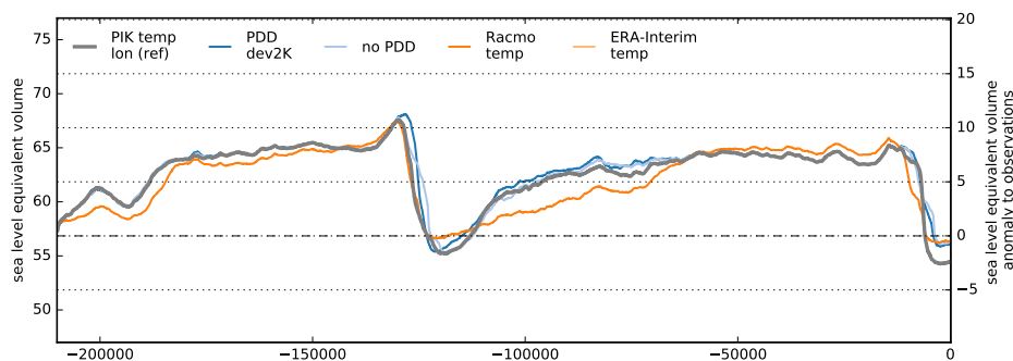
Figure 10: Ice volume above flotation for variation of PDD standard deviation and for different modern mean temperature distributions. The sensitivity is low for different PDD parameters of 5 K (reference in grey), 2 K and when off no surface model with yearly cycle is used (blue and light blue respectively), also for interglacials. For more realistic annual mean surface temperatures from Racmo2.3p2 (Wessem et al., 2018) or ERA-Interim (Dee et al., 2011), but without PDD and yearly cycle applied show slightly more difference in , the simulated volumes show most difference for glacial ice sheet growth and at interglacials (orange and light orange respectively).
