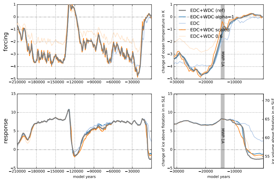
Figure 22: Sensitivity of transient ice volume above flotation to varied ocean temperature forcing. Reference simulation (grey) is based on EDC+WDC surface temperature with fit response function of power \alpha = 2 . The resulting ice volume change is similar for a fit response function with power \alpha = 1 (blue). Even if ocean temperature forcing responds immediately directly to the scaled surface temperature anomalies-anomaly (orange) the resulting effects on ice volume are comparably small. If a different surface temperature reconstructions-are-reconstruction is used, here from EDC with \alpha = 2 (light blue), we find for in response to a later warming signal a delayed deglaciation accordingly . If the amplitude of WDC surface temperature anomalies was 40% lower (light orange), this would have only negligible effect on the modeled ice volume.
