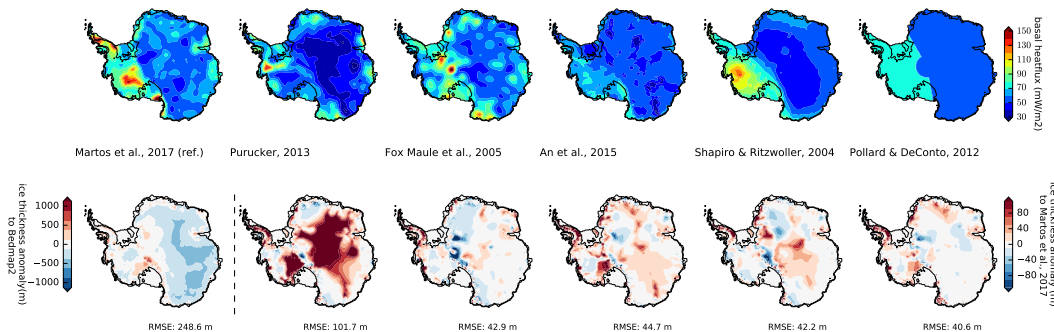
Figure 11: PISM present-day equilibrium results after 50 kyr for different basal heat flux fields (upper row) affecting the near-ground ice temperatures and hence the ice thickness, here shown for the first equilibrium result as anomaly to Bedmap2 (first panel in lower row) or relative to the first PISM -result. First three columns show the results for the magnetic reconstructions by Martos et al. (2017) (as in the reference), Purucker (2013) and Fox Maule et al. (2005). Columns 4 to 5 show the seismic reconstructions by An et al. (2015) and Shapiro and Ritzwoller (2004), and last column for comparison a two-valued field as used in Pollard and DeConto (2012a), separating East and West Antarctica. The overall effect of the choice of geothermal heatflux on present-day equilibrium ice thickness measures up to 100 m RMSE for Purucker (2013), while for the other tested setups it differs only in individual spots with a RMSE of 40–45 m.
