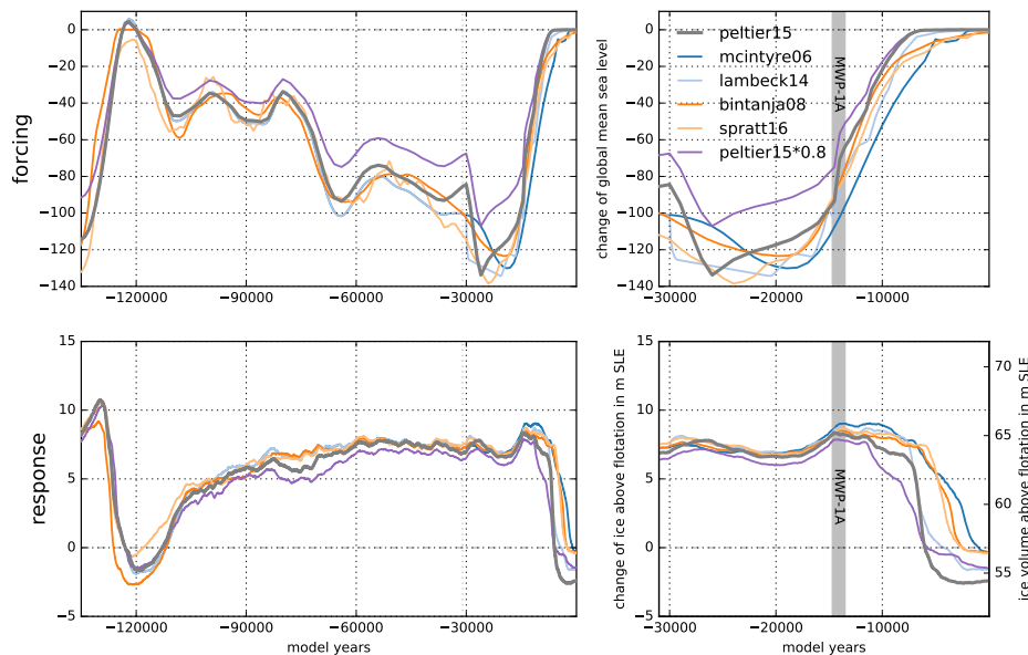
Figure 18: Time series of reconstructed sea-level change over the last 135 kyr (upper left) and the last 30 kyr (upper right) by Stuhne and Peltier (2015); Imbrie and McIntyre (2006); Lambeck et al. (2014); Bintanja and Van de Wal (2008); Spratt and Lisiecki (2016) and corresponding PISM-simulated sea-level relevant ice volume anomaly relative to observations (Fretwell et al., 2013) in lower panels. In order to approximate the effect of self-gravitation we scaled the ICE-6G forcing (Stuhne and Peltier, 2015) by 80%. For about 25 m higher sea-level stand at LGM we find almost the same modeled ice volume, while we find earlier but more gradual deglaciation (violet).
