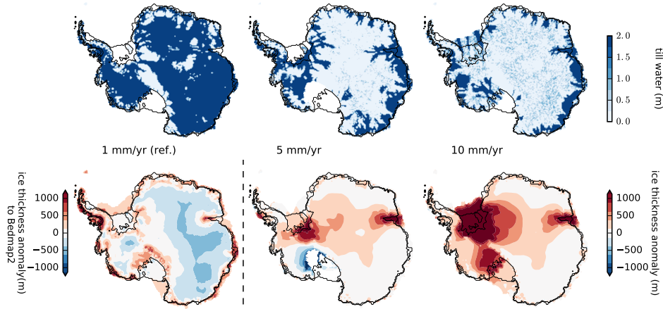
Figure 16: Present-day result of glacial cycle simulation showing ice thickness anomaly to Bedmap2 (lower left) and/or to reference (lower-right) for different till water decay rates (from left to right, 1 mm/yr, 5 mm/yr, and 10 mm/yr) causing different till water distributions underneath the ice sheet (upper row). For a reference decay rate of 1 mm/yr about 90% of ice sheet's bed is saturated, while for 10 mm/yr saturated till is only found in the coastal regions and underneath the fast-flowing ice stream.
