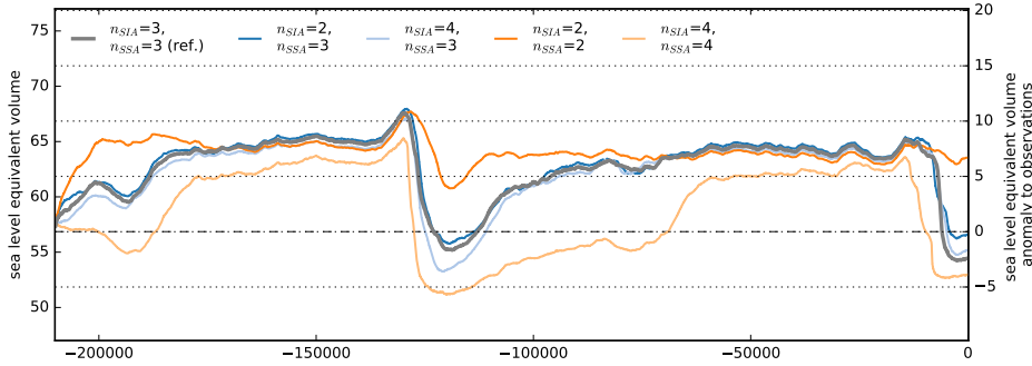
Figure 4: Simulations with different flow law exponents in the SIA and SSA stress balance, varying from 2–4. For variation of the SIA flow law exponent we find only small impact on ice volume (blue, grey, light blue), while for the SSA it strongly affects ice sheet growth and deglaciation (orange and light orange).
