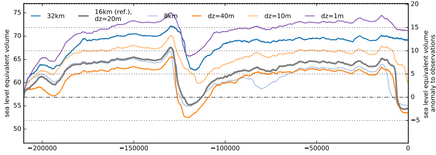
Figure 5: Ice volume above flotation for simulations with horizontal reference resolution of 16 km (grey), fine grid resolution of 8 km (light blue) and relatively coarse resolution of 32 km (blue) resulting in different Antarctic Ice Sheet histories. Refined vertical resolution of 10 m (light orange) and 1 m (violet) at the base yields larger ice volumes than the reference simulation with 20 m (grey) or for coarse resolution of 40 m (orange).
