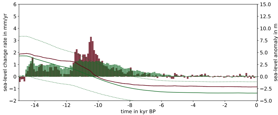
Figure S3: During deglaciation the score-weighted ensemble mean (green) shows most of the sea-level change rates between 14.5 kyr-kyr BP (MWP1a) and 8 kyr-kyr BP with mean rates around 1 mm yr -1 , while the best-score simulation (red) reveals rates of sea-level rise of up to 4 mm yr -1 (100 yr-yr bins) in the same period (cf. Golledge et al., 2014, Fig. 3 d). In contrast to the base ensemble (cf. Fig. 9c) the basal ensemble shows a much earlier deglacial retreat and no regrowth during the late Holocene.
