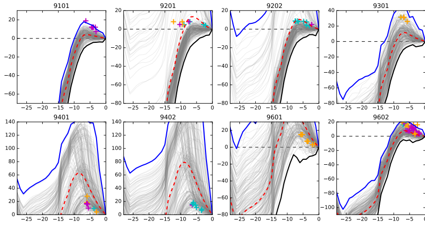
Figure S7: Regional sea level (RSL) data points and ensemble sea level curves for the 8 data sites, analogous to Fig. 5–6 in Briggs et al. (2014), upper panels in EAIS, lower panels in Antarctic Peninsula and Ross sector. Observed RSL data points are colour coded according to the constraint they provide: two-way (light blue, dated past sea level); one-way lower-bounding (mauve, past sea level above or maximum age of beach) or one-way upper-bounding (orange, past sea level below or minimum age beach). For a detailed description of the RSL datasets and its processing, refer to Briggs and Tarasov (2013). RSL has not been used as constraint in this study.
