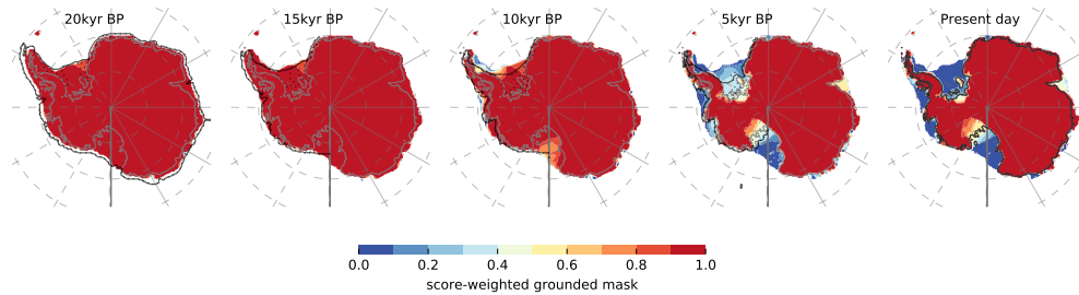
Figure 7: Ensemble-score weighted grounded mask for 5 kyr -kyr snapshots. Mask value 1 (red) indicates grounded area which is covered by all simulations, while blueish colors indicate areas which are covered only by a few simulations with low scores (compare Fig. D4 in Pollard et al. (2016)). For the last two snapshots, grounding line in the Ross Sea and Weddell Sea sector is found in about 50% of score-weighted simulations inland of its present location (Fretwell et al., 2013, grey line) with some grounding line re-advance (Kingslake et al., 2018; Siegert et al., 2019). In contrast less than 10% show no grounding-line grounding-line retreat from glacial maximum extent. Black lines indicate reconstructions by the RAISED Consortium ( Bentley et al., 2014, Scenario B solid and scenario A dashed ) (Bentley et al., 2014, Scenario B solid and scenario A dotted) .
