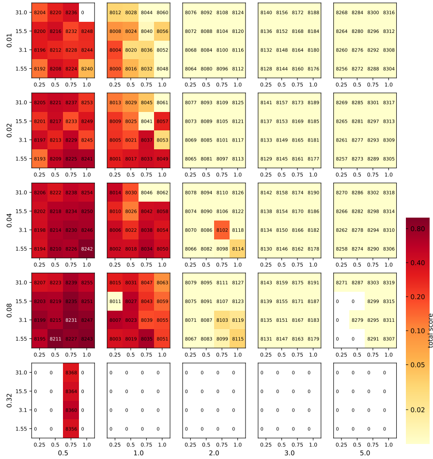
Figure S1: Aggregated score for 318 ensemble members (4 model parameters, 4-5 values each) showing the distribution of the scores over the full range of plausible basal parameter values. The score values are computed versus geologic and modern data sets, normalized by the best score in the ensemble, and range from <0.01 (bright yellow, no skill) to 1 (dark red, best score) (cfs. Pol-lard et al., 2016, Figs. 2 + C1), on a logarithmic color scale. The four parameters are the effective overburden pressure fraction FEOP (outer y-axis), the minimal till friction angle on the continen-tal shelf PHIMIN (outer x-axis), the tillwater decay rate TWDR (inner y-axis) and the power-law sliding pseudoplasticity exponent PPQ (inner x-axis). In the lowest row, only four ensemble scores are shown for 32% of effective overburden pressure fraction, just to ascertain that aggregated scores decline for larger FEOP.
