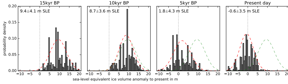
Figure 10: Equivalent-Histogram of ensemble global-mean sea-level contribution-(ESL) contributions relative to modern observation at every 5 kyr-kyr over the last deglaciation period. Grey bars show the score-weighted ensemble distribution (0.5 m-m bins), the red curve indicates the statistically likely range (normal distribution) of the simulated ice volumes with width of 1-sigma standard deviation as for the green envelope in Fig. 9, green gaussian-Gaussian curve from 15k kyr snapshot for comparison (compare to Figs. 6 + C5 in Pollard et al. (2016)).
