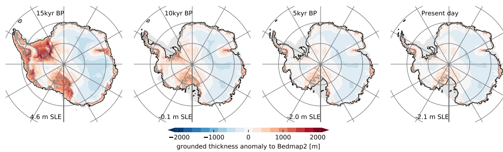
Figure S2: Snapshots of grounded ice thickness anomaly to present-day observations (Bedmap2; Fretwell et al., 2013) over the last 15 kyr kyr for best-fit simulation in the basal ensemble. At LGM state grounded ice extends towards the edge of the continental shelf, with much thicker ice than present mainly in West Antarctica. Retreat of the ice sheet initiates between 12 and 11 kyr kyr BP and halts already latest 8 kyr kyr in all large ice shelf basins of Ross, Weddell Sea, Amery and Amundsen Sea. East Antarctic Ice Sheet thickness is underestimated throughout the deglaciation period (light blue). Compare Fig. 2 in Golledge et al. (2014).
