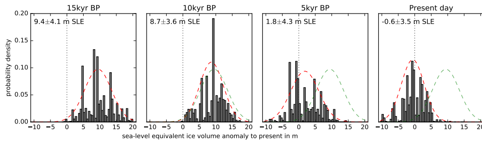
Figure 10: Equivalent-Histogram of ensemble global-mean sea-level contribution-(ESL) contributions relative to modern observation at every 5 kyr over the last deglaciation period. Grey bars show the score-weighted ensemble distribution (0.5 m bins), the red curve indicates the statistically likely range (normal distribution) of the simulated ice volumes with width of 1-sigma standard deviation as for the green envelope in Fig. 9, green gaussian-Gaussian curve from 15k kyr snapshot for comparison (compare to Figs. 6 + C5 in Pollard et al. (2016)).
