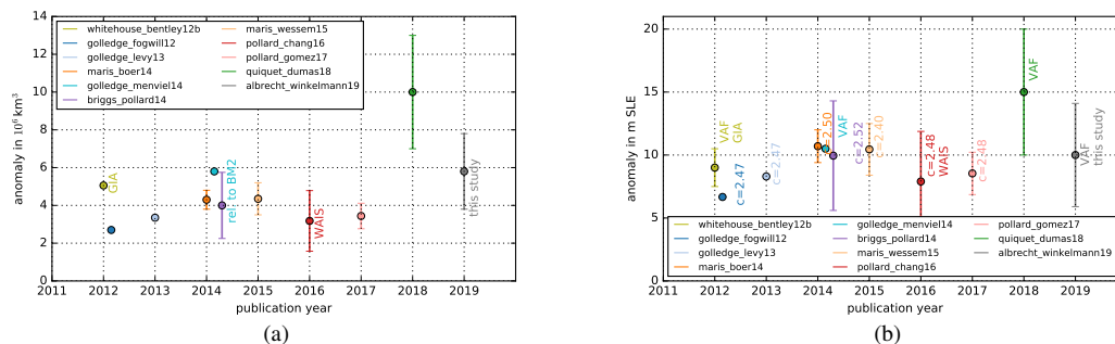
Figure 11: Ice volume anomaly between Last Glacial Maximum as compared to present (not observations) in recent modeling studies in units of 10^6 \text{ km}^3 (a) and in units of meters sea-level equivalents (b). Note that the study by Pollard et al. (2016) only considers the West Antarctic subdomain in their analysis (redish). Golledge and colleagues and this study used PISM (blue and grey), Maris and colleagues used ANICE (orange), Whitehouse and colleagues used GLIMMER simulations (olive), GRISLI simulations by Quiquet and colleagues (green) and Briggs and Pollard and colleagues used PennState3D (or PSU-ISM) as model (blueish) coupled to different Earth models. Be aware, that ice volume estimates are based on different ice densities in the different models and that different conversion factors c have been used. This study, Golledge et al. (2014), as well as the Glimmer and GRISLI model provided the volume above flotation (VAF), which subtracts some portion of the ice volume in panel (b). The provided uncertainty ranges are not necessarily symmetric, e.g. the upper range in Briggs et al. (2014) has less confidence than the lower range.
