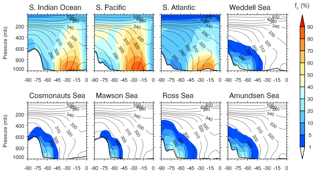
Figure S5: Vertical distribution of fractional contribution (%) to annual and zonal mean water vapor mixing ratio from individual source regions in the “mean” case. Contour lines are zonal mean equivalent potential temperature ( \theta_e ). Zonal mean in each panel is taken along the corresponding longitude band of the source region.
