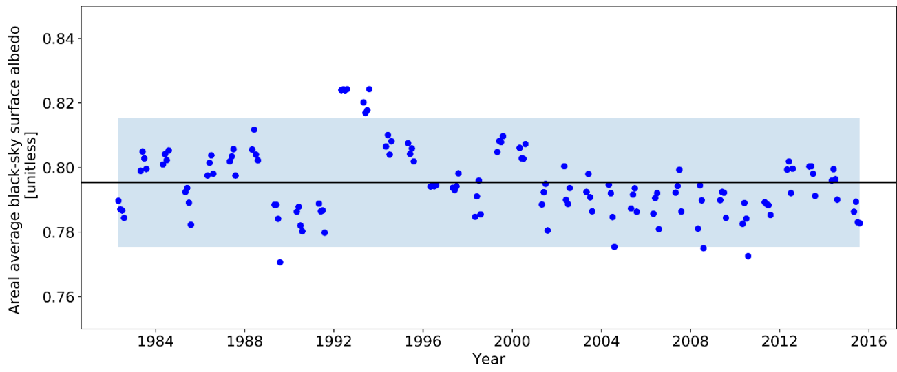
5 Figure 1: Stability of CLARA-A2 SAL over 73-75 °N, 38-42 °W, on the central part of the Greenland ice sheet. Spatially averaged monthly mean albedo retrievals between May and August shown. The black line shows the 34-yr mean albedo of the area. Light blue shading shows \pm 0.02 albedo variability about the interannual mean, corresponding to the reported upper accuracy estimate of 5% relative for CLARA-A2 SAL over snow and ice.
