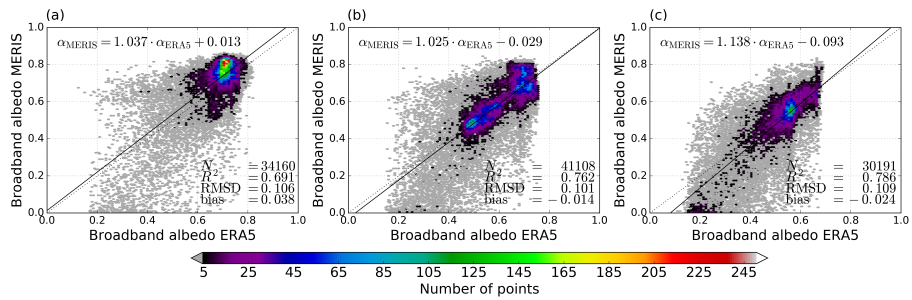
Figure 7. Comparison of ERA5 and MERIS derived grid-cell broadband albedo of Arctic sea ice on selected days of Fig. 6 (a): 2 June 2007, before melt onset; (b): 12 June 2007, at melt onset; (c): 25 June 2007, after melt onset). Regression line and 1-to-1 line are shown in black solid and dotted, respectively.
