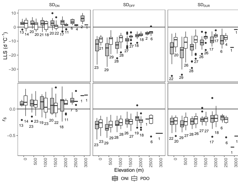
Fig. 3. Linear least squares (LLS; top panel) and Spearman correlation coefficients ( r_S ; bottom panel) per hydrozone for SDON, sdoFF and SDDUR with ONI and PDO in 500 m elevation bins.
