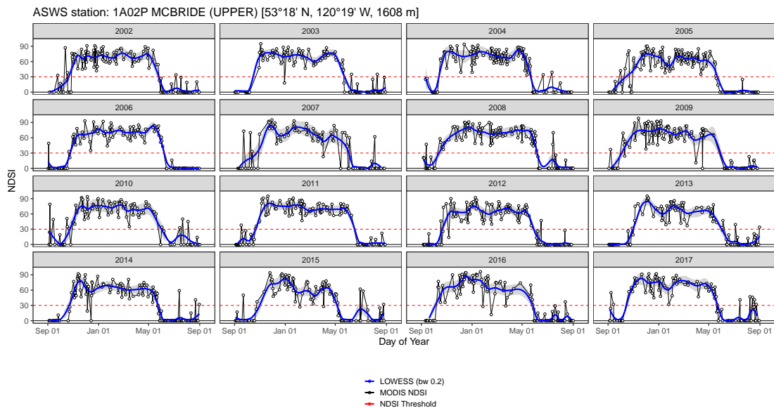
Fig. 1. An example of the LOWESS time series interpolation of MODIS NDSI data at the ASWS station 1A02P McBride (Upper) for the hydrological years 2002-2017.
