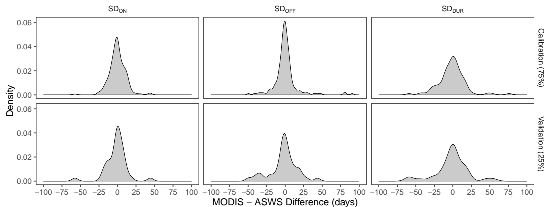
Fig. 2. Distribution of errors calculated from the difference between MODIS and ASWS values for each snow measurement.
