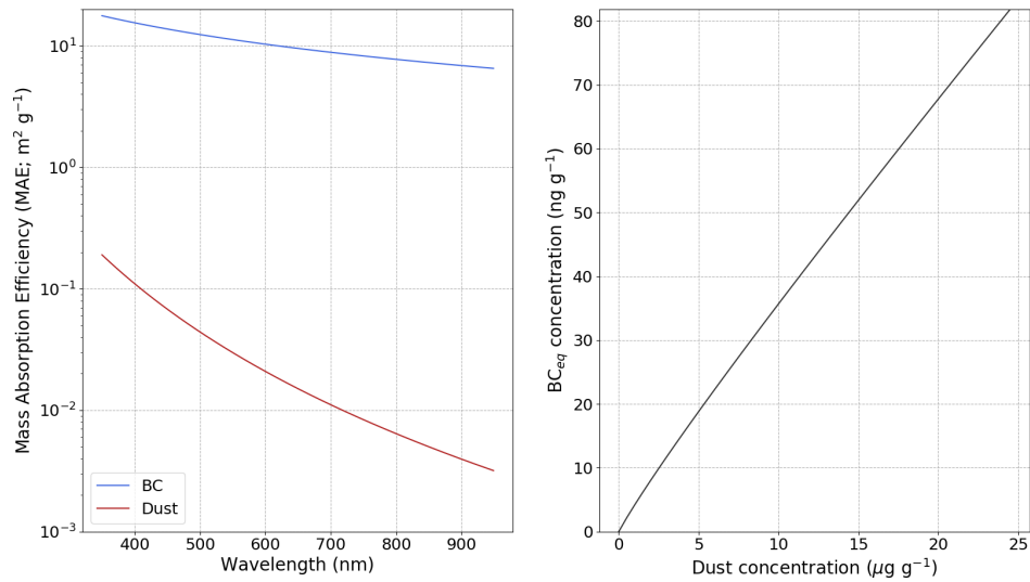
Figure 1. EqBC concentration corresponding to a given dust concentration with the model configuration. a) Mass Absorption Efficiency (e.g.: B g , LAP-MAE) values of BC and dust used in the present study as a function of wavelength. b) EqBC concentration corresponding to a given dust concentration using these MAE values and the methods described in Section 3.1.
