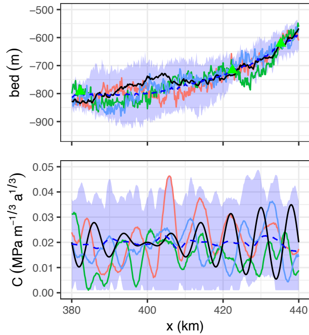
Figure 5. Initial ensemble for the bed and friction coefficient, the reference is shown in black, the synthetic bed measurements are shown as green dots-triangles in the top panel, the ensemble mean is the dashed blue curve and the shading shows the ensemble spread. Coloured solid lines show the first 3 members.
