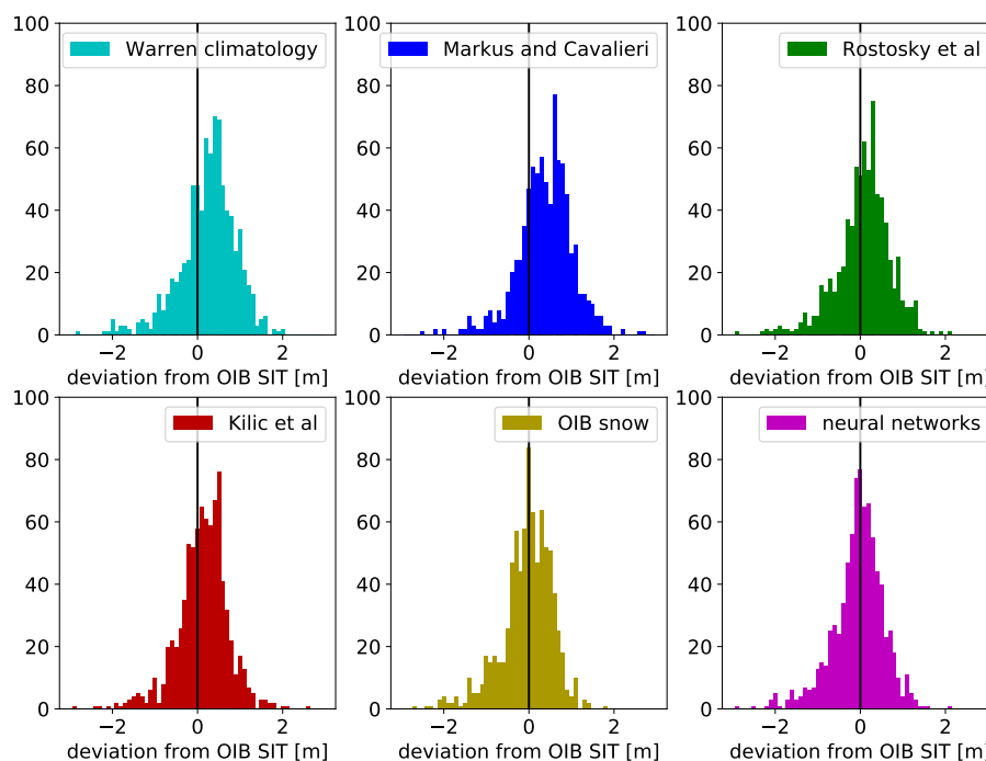
Figure 11. Deviation from OIB (predicted SIT using CryoSat freeboard with different snow depth algorithms minus OIB measured SIT) for all OIB data. The vertical black line indicates a perfect match between OIB and the algorithm, the left half corresponds to an underestimation and the right half to an overestimation of SIT compared to the OIB measurements.
