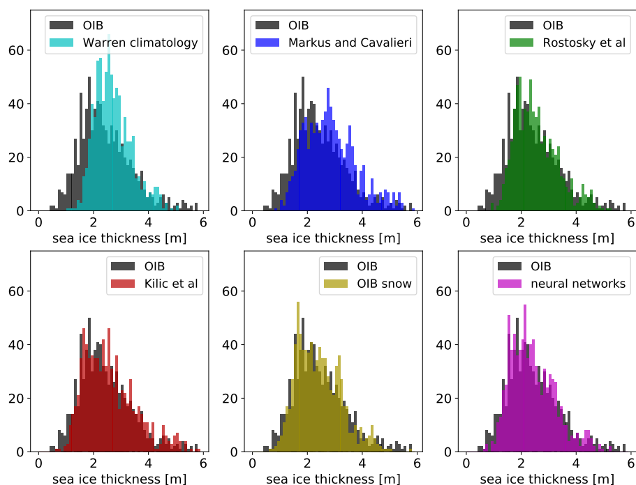
Figure 10. Distribution of OIB measured SIT (all data) in grey versus predicted SIT using CryoSat freeboard with different snow depth algorithms in colour.
