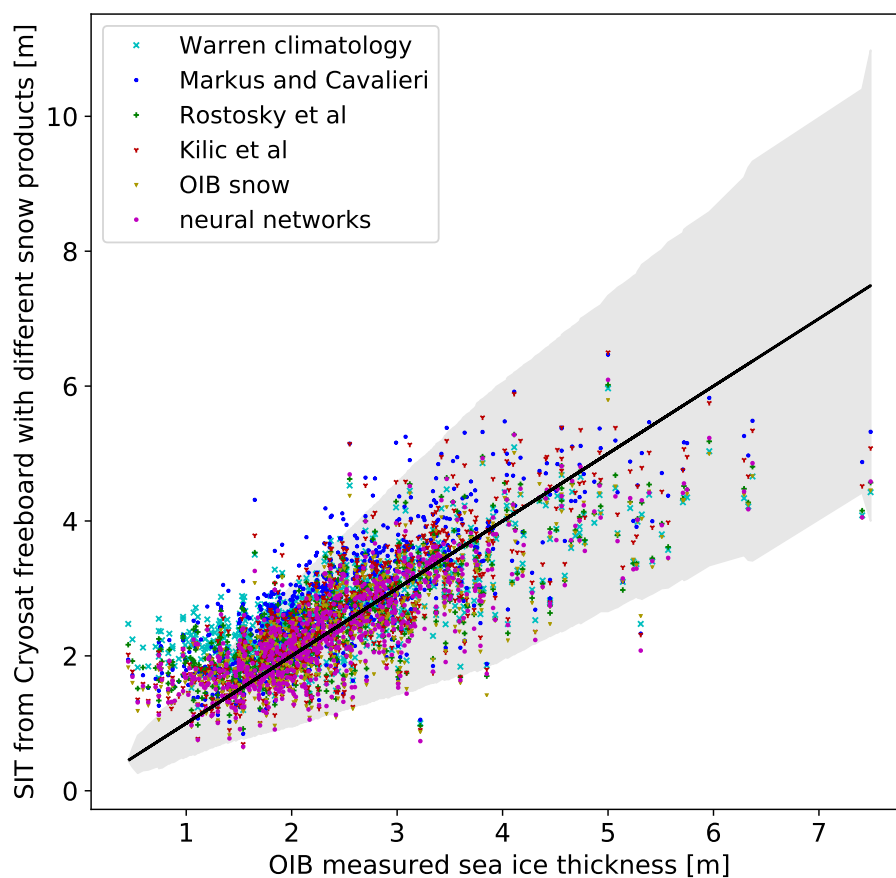
Figure 9. OIB measured SIT (all data) versus predicted SIT using CryoSat freeboard with different snow depth algorithms.
