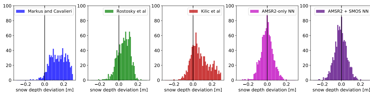
Figure 6. Deviation from OIB (predicted snow depth using different algorithms minus OIB measured snow depth) for all OIB data. The vertical black line indicates a perfect match between OIB and the algorithm, the left half corresponds to an underestimation and the right half to an overestimation of snow depth compared to the OIB measurements.
