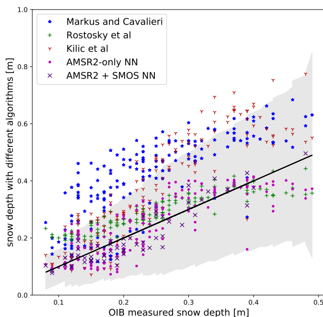
Figure 4. OIB measured snow depth (test data) versus predicted snow depth using different algorithms. Note that Markus and Cavalieri should only be applied over FYI, but this plot includes also MYI.
