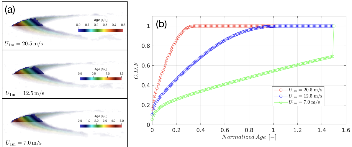
Figure 7. Distribution of age within a mobile barchan (case C24) prior to sintering: (a) Three panels show the distribution of age in the central slice of as well as the arms of the barchan for the three different wind scenarios. (b) Cumulative distribution function of the age of the entire barchan for the three different wind scenarios.
