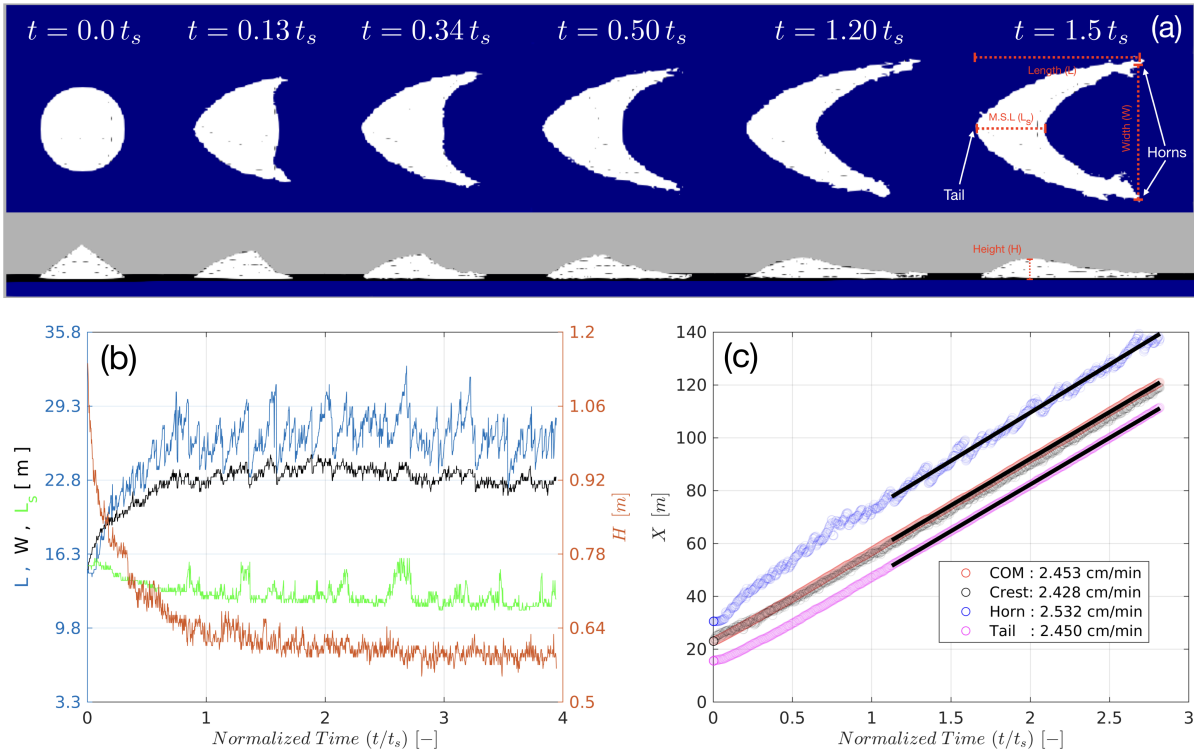
Figure 3. Morphodynamics of a solitary dune (case C20, high-wind scenario U_{1m} = 20.5\text{ms}^{-1} ): (a) Visual representation of evolution from a cone-pile to a barchan. The final image is annotated for identifying different descriptors of a barchan. (b) Evolution of the length (L), width (W) and the maximum streamwise length ( L_s ) of the barchan. (c) Different versions of calculating the dune speed using the displacement of either the center-of-mass (COM), tail, horns or crest of the dune.
