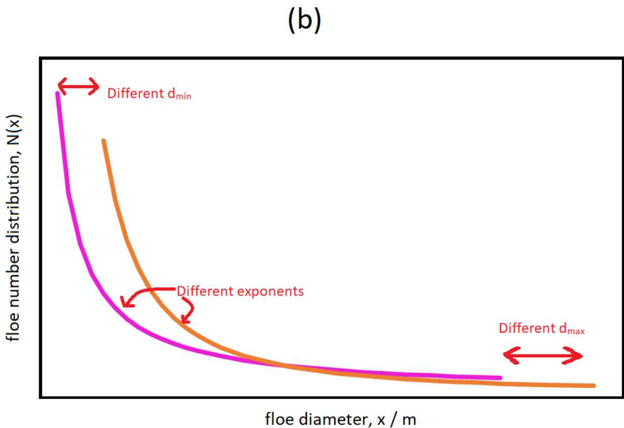
Figure 1: Panel (a) is a schematic of the imposed FSD model. This model is initiated by prescribing a power law with an exponent, \alpha , and between the limits d_{min} and d_{max} . Within individual grid cells the variable FSD tracer, l_{var} , varies between these two limits. l_{var} evolves through lateral melting, wave break-up events, freezing and advection. Not shown is how changes in l_{var} will also impact the floe size number distribution factor, C . Panel (b) shows the how d_{min} , d_{max} and \alpha can all be varied to produce floe size number distributions. All axes within both panels are logarithmic to base 10.
