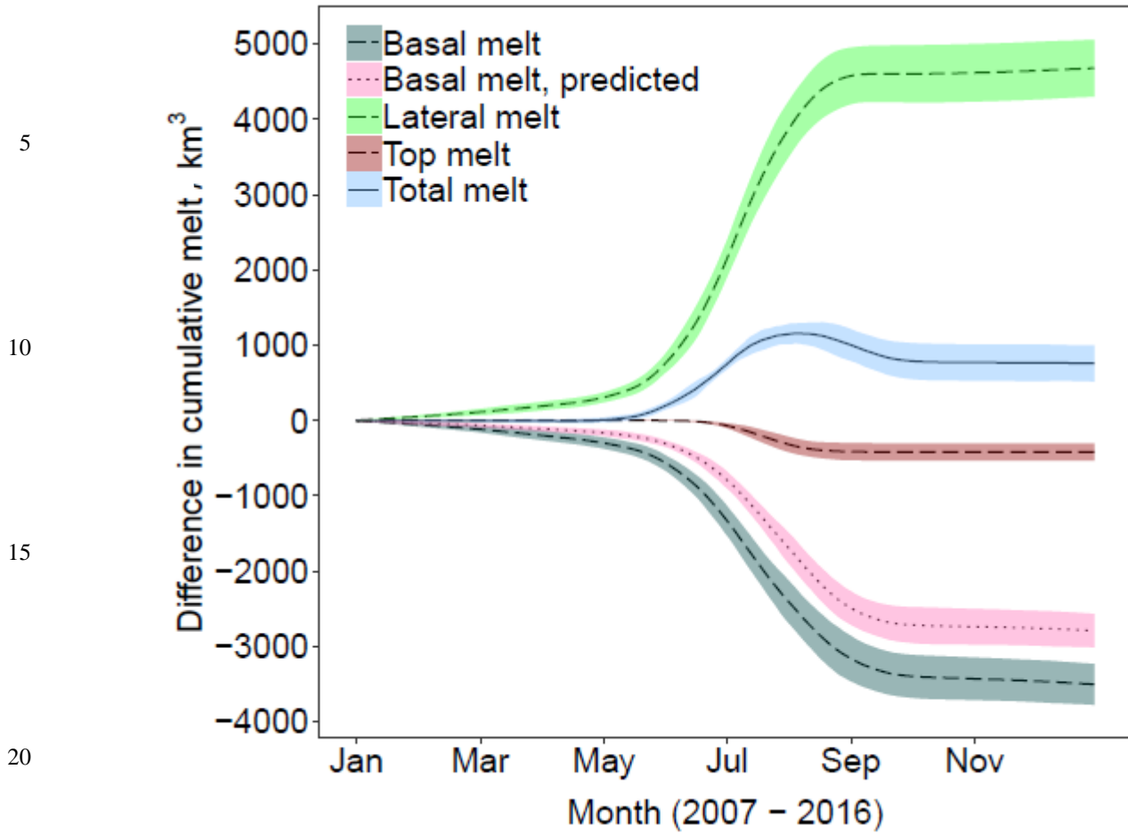
Figure 7: As Fig. 4 but the difference between (A) compared to stan-fsd i.e. the impact of changing \alpha from 2.5 to 3.5 with the other FSD parameters held at standard values. A large increase in lateral melt is partly compensated by a reduction in basal melt, however this time a large increase is seen in the total melt.
