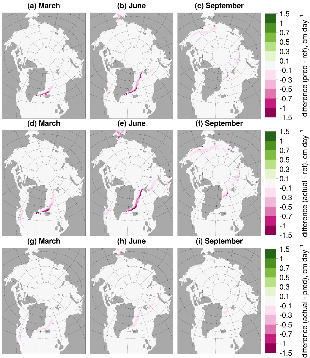
Figure 5: Predicted reduction in basal melt rate from stan-fsd to ref (top row, a-c), actual reduction in basal melt rate from stan-fsd to ref (middle row, d-f), and difference between the actual reduction and predicted reduction in basal melt rate (bottom row, g-i) averaged over 2007 – 2016. Results are presented for March (left column, a, d, g), June (middle column, b, e, h) and September (right column, c, f, i). Values are shown only in locations where the sea ice concentration exceeds 5 %. The predicted reduction in basal melt rate refers to the expected reduction if the change in sea ice area fraction is the only factor driving the change in basal melt rate. This is calculated by multiplying the basal melt rate for ref by the relative percent change in ice area fraction from ref to stan-fsd for each grid cell.
