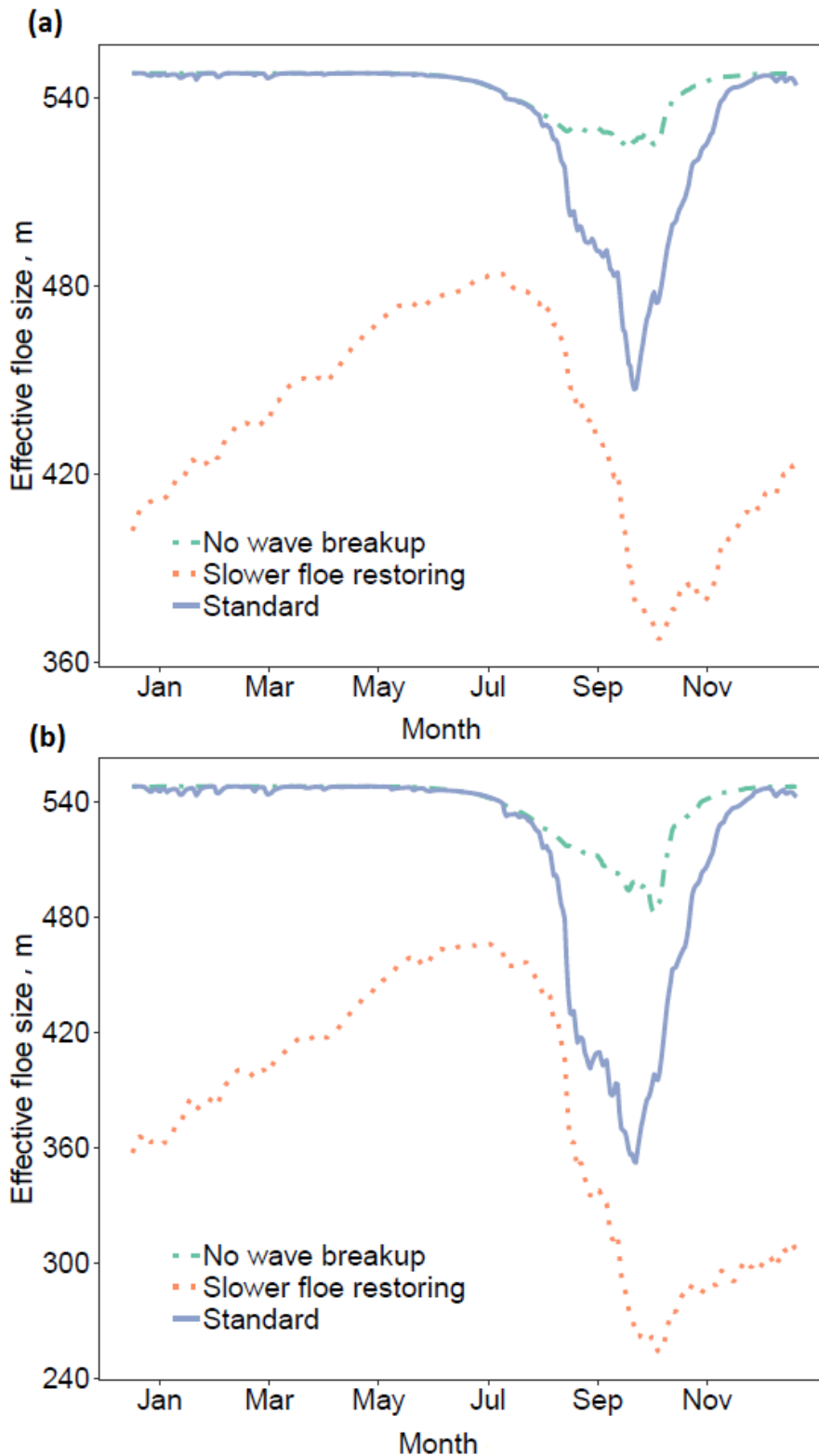
Figure 13: Daily variation in l_{eff} over 2015 averaged over (panel a) regions with between 15 – 80 % sea ice concentration on 31 st August 2015 and (panel b) regions with between 15 – 30 % sea ice concentration of 31 st August 2015. The three simulations demonstrate l_{eff} tendencies with respect to different processes. The plots show the evolution of l_{eff} throughout the year for the standard simulation ( fsd-stan , blue solid), without wave break-up of floes (F, green dot-dashed), and with a reduced floe size restoring rate in freezing conditions (K, orange dotted). Means for l_{eff} and ice perimeter are taken as averages over the selected grid cells with each grid cell equally weighted. The plots show that a strong seasonal cycle in l_{eff} can be observed, particularly in grid cells on the edge of the sea ice cover where waves are expected to have a particularly strong impact.
