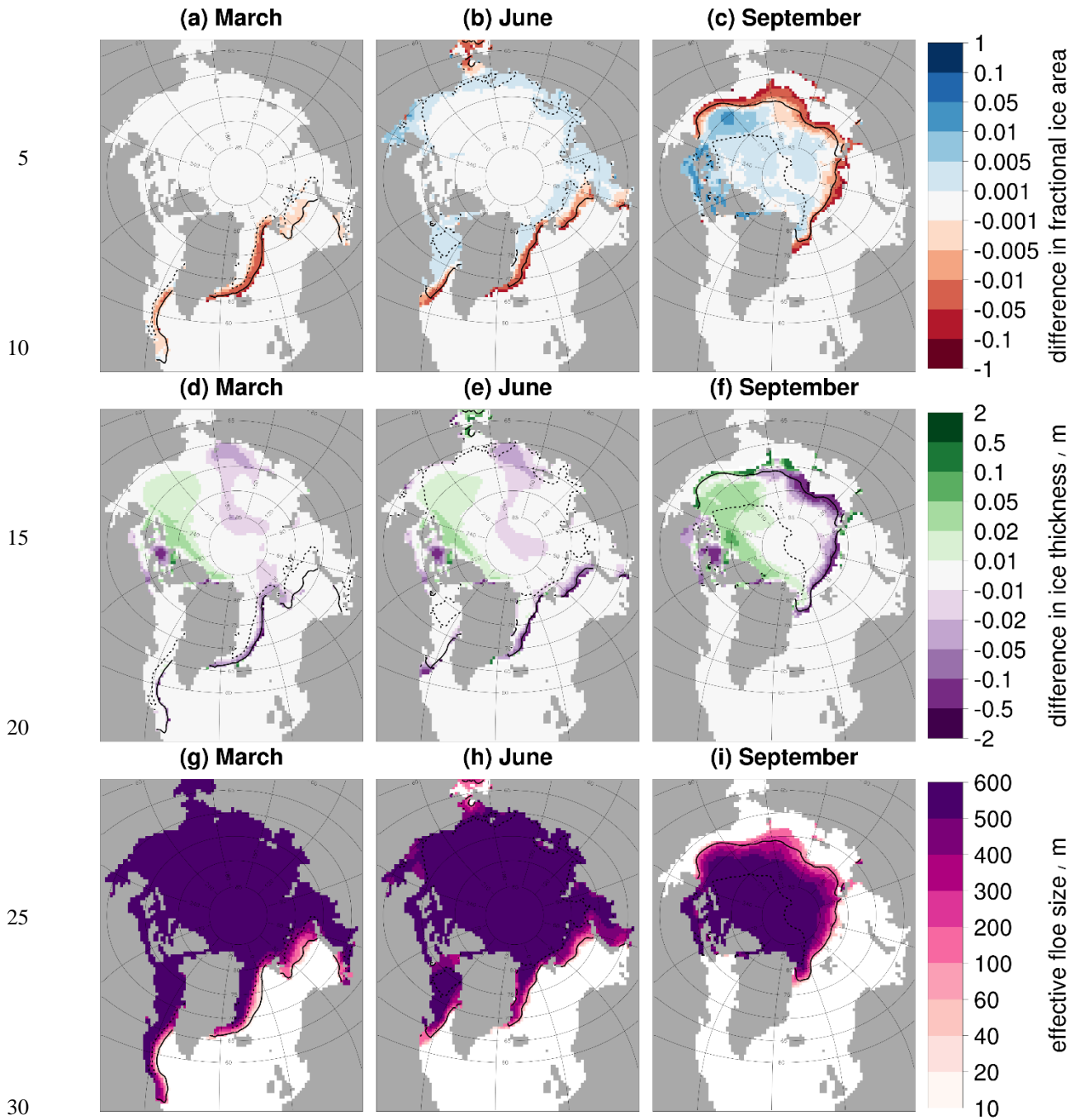
Figure 6: Difference in the sea ice concentration (top row, a-c) and ice thickness (middle row, d-f) between stan-fsd and ref and l_{eff} (bottom row, g-i) for stan-fsd averaged over 2007 – 2016. Results are presented for March (left column, a, d, g), June (middle column, b, e, h) and September (right column, c, f, i). Values are shown only in locations where the sea ice concentration exceeds 5 %. The inner (dashed black) and outer (solid black) extent of the MIZ averaged over the same period is also shown. In general, the plots show an increase in the sea ice concentration and thickness in the pack ice, but a reduction in the MIZ. This corresponds to the behaviour of the l_{eff} , with increases in regions where the l_{eff} is above 300 m and reductions where it is below 300 m.
