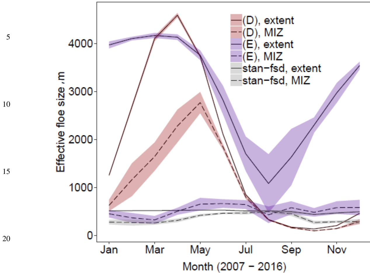
Figure 11: Annual variation in mean l_{eff} averaged over 2007 – 2016 for two simulations with variable \alpha . The plots show the evolution of l_{eff} throughout the year for a simulation with a time-dependent \alpha (D, red ribbon) or a sea ice concentration-dependent \alpha (E, blue ribbon). Also shown is the behaviour of l_{eff} for a simulation with a fixed \alpha of 2.5 ( fsd-stan , grey ribbon). Results are shown for the total sea ice area (solid) and MIZ only (dashed). The mean l_{eff} is taken as the equally weighted average across all grid cells where the sea ice concentration exceeds 5% (total extent) or is between 15% - 80% (MIZ only). The ribbon shows, in each case, the region spanned by the mean value plus or minus two times the standard deviation for each simulation. The results show that introducing a variable \alpha produces much larger intra-annual variations in l_{eff} across the overall sea ice extent than with a fixed \alpha . (D) and (E) show an annual oscillation in the value of l_{eff} averaged over the total sea ice extent. Within the MIZ, only experiment (D) continues to show this strong variation in l_{eff} ; (E) and fsd-stan show variations of around an order less. (D) shows the strongest interannual variation between March and May, whereas for (E) it is strongest in the peak melting season between July and August.
