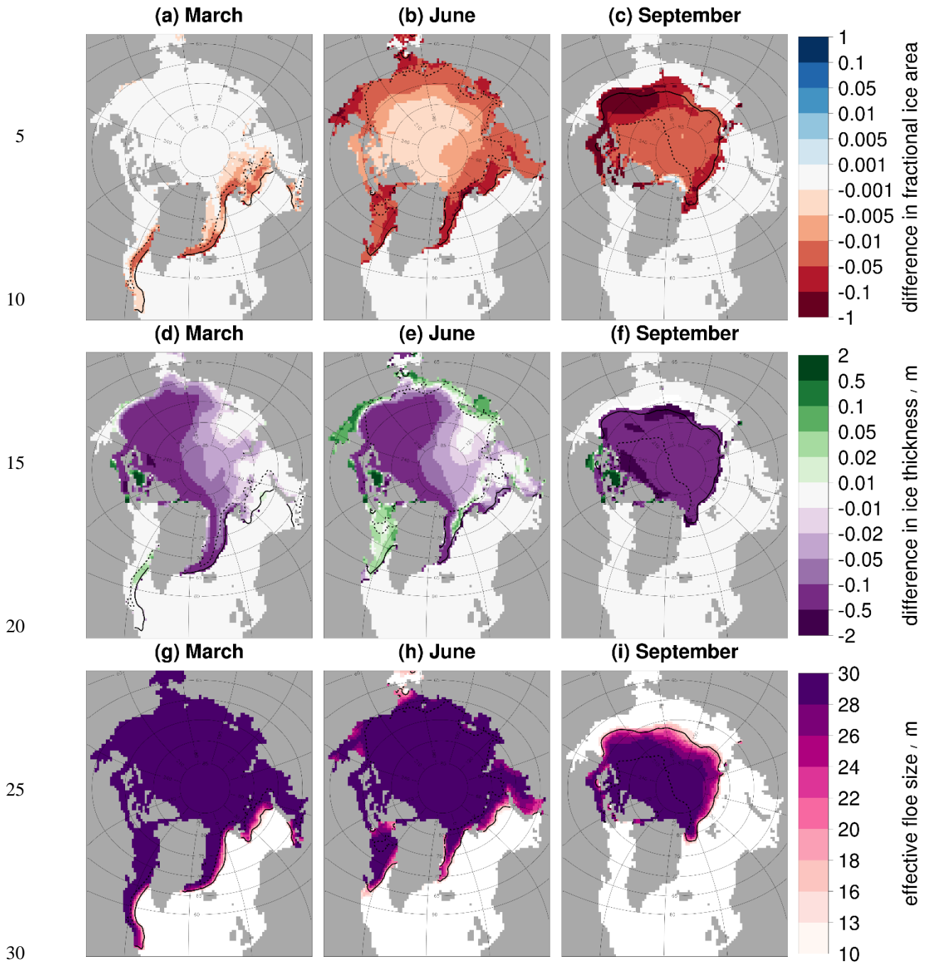
Figure 8: As Fig. 6 except now the difference between (A) compared to stan-fsd is given i.e. the impact of changing \alpha from 2.5 to 3.5 with the other FSD parameters held at standard values. l_{eff} is reported for the simulation with the higher magnitude \alpha . In general, the plots show a reduction in the sea ice concentration and ice thickness across the sea ice cover. This corresponds to the behaviour of the l_{eff} , with the l_{eff} 30 m or below across the sea ice cover.
