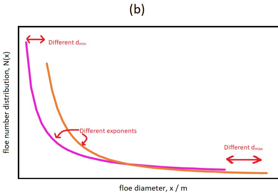
Figure 1: Panel (a) is a schematic of the imposed FSD model. This model is initiated by prescribing a power law with an exponent, \alpha , and between the limits d_{min} and d_{max} . Within individual grid cells the variable FSD tracer, l_{var} , varies between these two limits. l_{var} evolves through lateral melting, wave break-up events, freezing and advection. Not shown is how changes in l_{var} will also impact the floe size number distribution factor, C . Panel (b) shows the how d_{min} , d_{max} and \alpha can all be varied to produce floe size number distributions. All axes within both panels are logarithmic to base 10.
