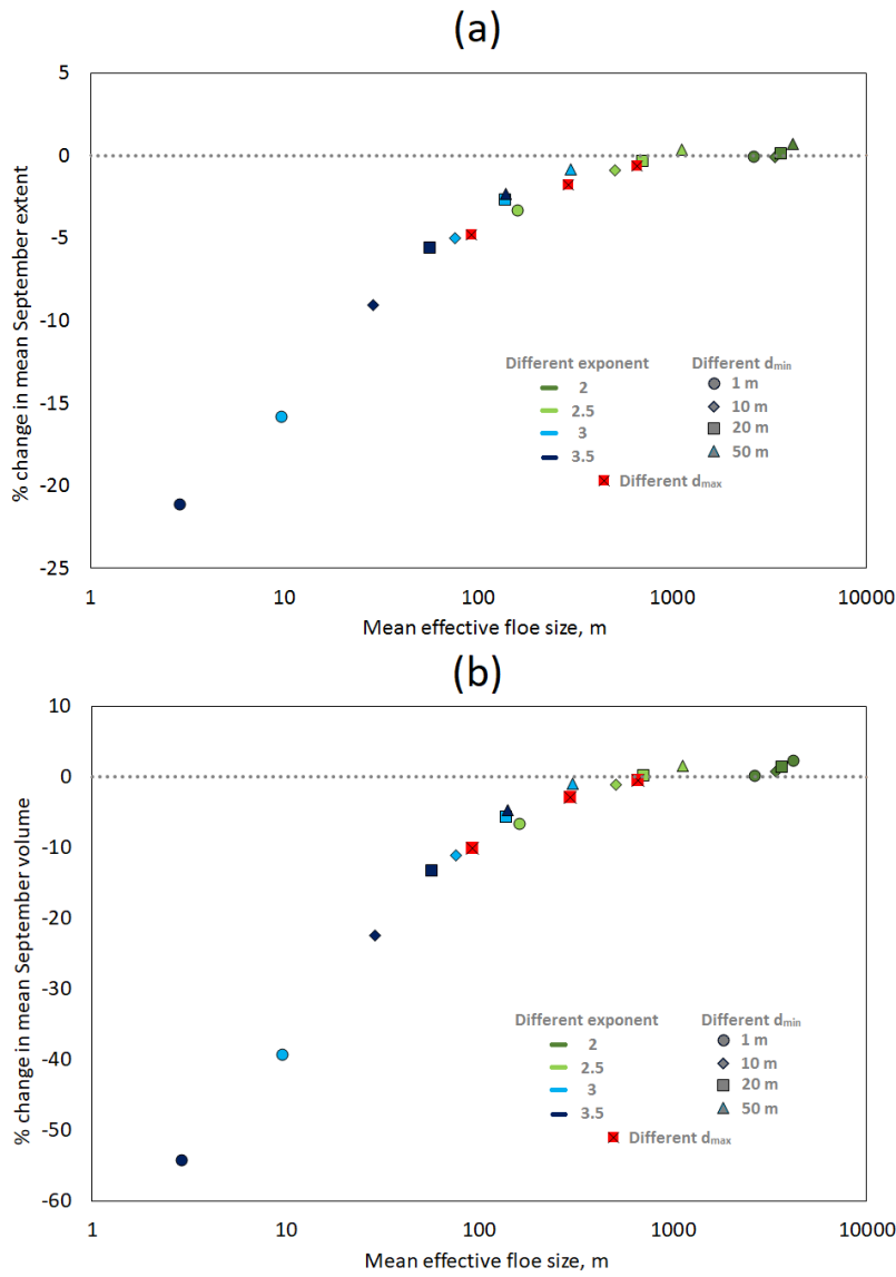
Figure 9: Relative change (%) in mean September sea ice extent (a) and volume (b) from 2007 - 2016 respectively, plotted against mean l_{eff} for simulations with different selections of parameters relative to ref . The mean l_{eff} is taken as the equally weighted average across all grid cells where the sea ice concentration exceeds 15%. The colour of the marker indicates the value of the \alpha , the shape indicates the value of d_{min} , and the three experiments using standard parameters but different d_{max} (1000 m, 10000 m and 50000 m) are indicated by a crossed red square. The parameters are selected to be representative of a parameter space for the WIPoFSD that has been constrained by observations. Model response ranges from small increases in the sea ice extent and volume to reductions of over 20 and 50 % respectively. The mean l_{eff} is shown to be a good predictor of the response of the sea ice extent and volume.
