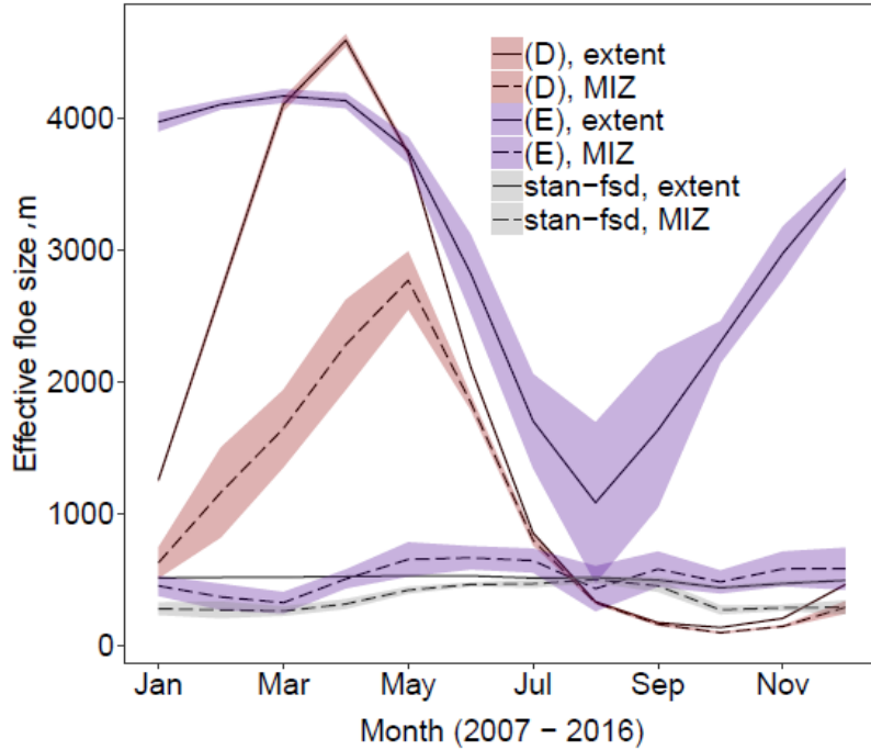
Figure 11: Annual variation in mean l_{eff} averaged over 2007 – 2016 for two simulations with variable \alpha . The plots show the evolution of l_{eff} throughout the year for a simulation with a time-dependent \alpha (D, red ribbon) or a sea ice concentration-dependent \alpha (E, blue ribbon). Also shown is the behaviour of l_{eff} for a simulation with a fixed \alpha of 2.5 ( fsd-stan , grey ribbon). Results are shown for the total sea ice area (solid) and MIZ only (dashed). The mean l_{eff} is taken as the equally weighted average across all grid cells where the sea ice concentration exceeds 5% (total extent) or is between 15% - 80% (MIZ only). The ribbon shows, in each case, the region spanned by the mean value plus or minus two times the standard deviation for each simulation. The results show that introducing a variable \alpha produces much larger intra-annual variations in l_{eff} across the overall sea ice extent than with a fixed \alpha . (D) and (E) show an annual oscillation in the value of l_{eff} averaged over the total sea ice extent. Within the MIZ, only experiment (D) continues to show this strong variation in l_{eff} ; (E) and fsd-stan show variations of around an order less. (D) shows the strongest interannual variation between March and May, whereas for (E) it is strongest in the peak melting season between July and August.
