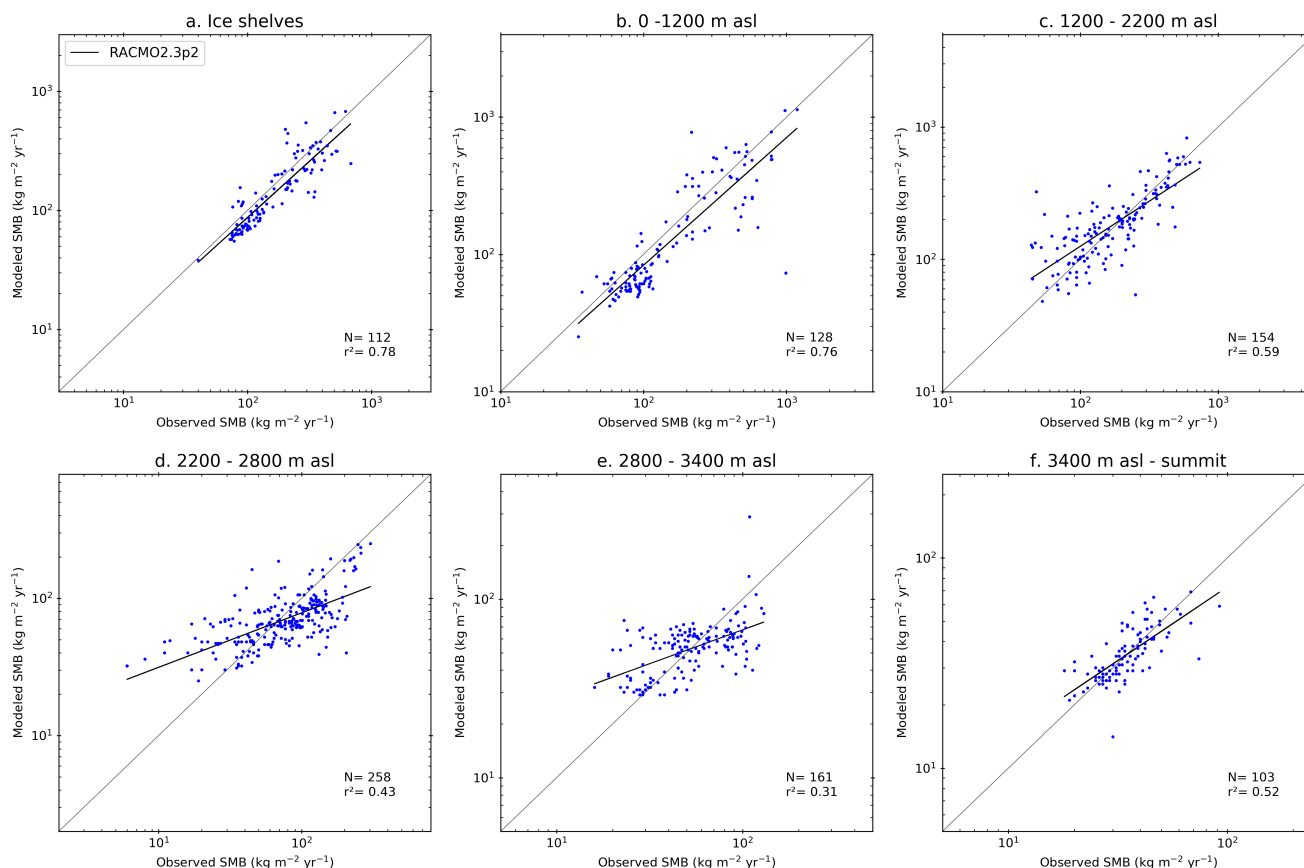
Figure A7. Comparison between RACMO2.3p2 and observed SMB (units= \text{kg m}^{-2} \text{yr}^{-1} ) over the ice shelves (a) and by elevation classes (b-f). Due to the use of logarithmic axes, only positive values for the observed and modelled SMB from all the RCMs in this study are used (number for each bin N). Finally, the regression coefficient of each regression line is also shown ( r^2 ).
