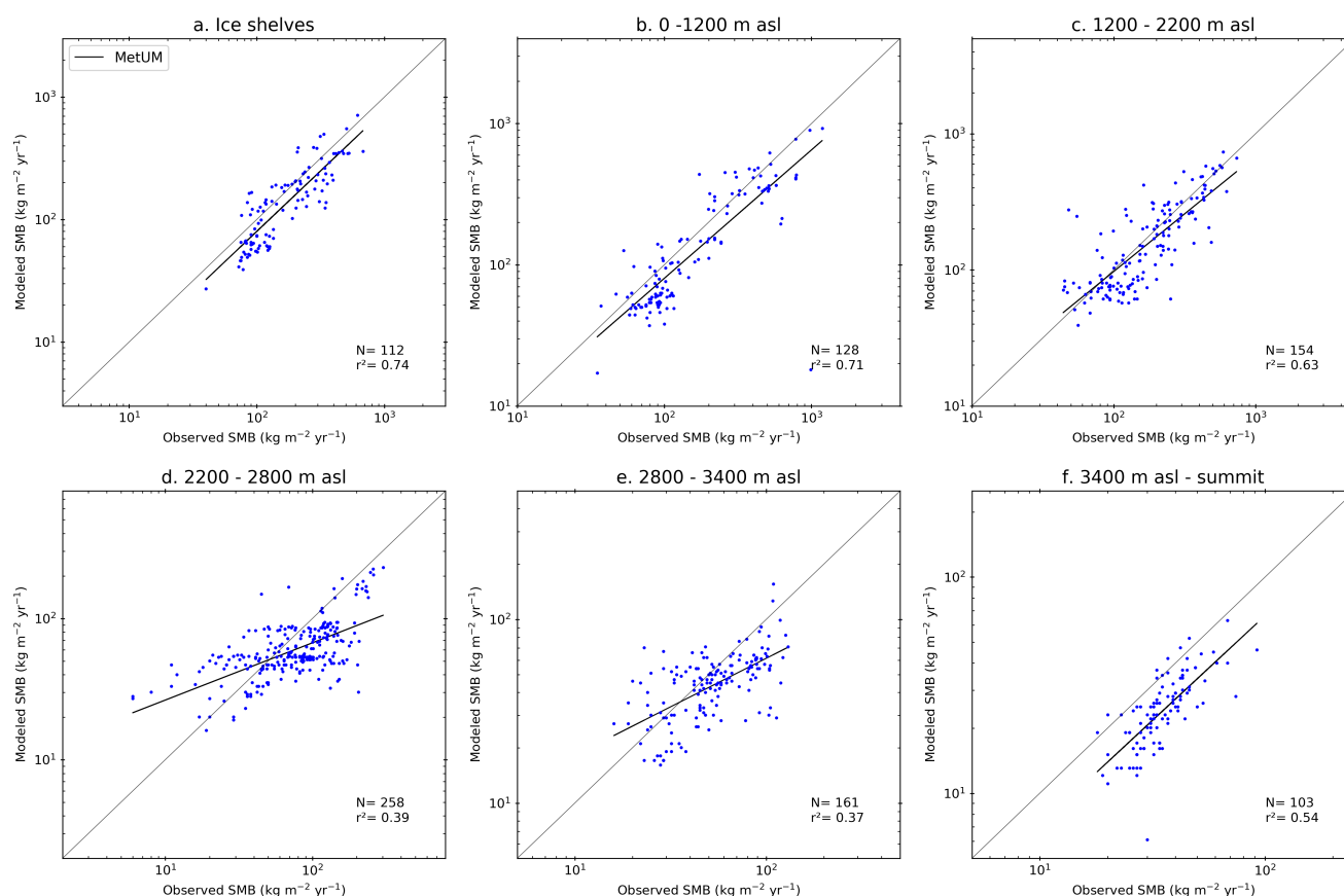
Figure A6. Comparison between MetUM and observed SMB (units= \text{kg m}^{-2} \text{yr}^{-1} ) over the ice shelves (a) and by elevation classes (b-f). Due to the use of logarithmic axes, only positive values for the observed and modelled SMB from all the RCMs in this study are used (number for each bin N). Finally, the regression coefficient of each regression line is also shown ( r^2 ).
