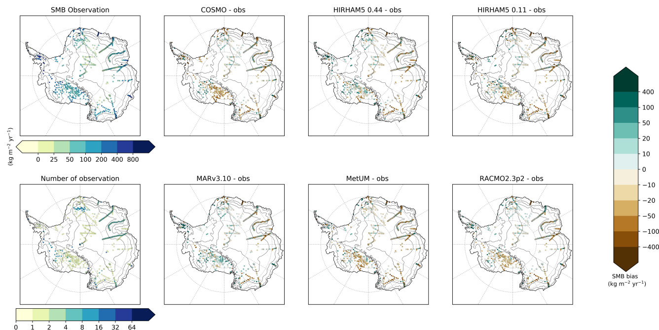
Figure 4. a) Observed SMB values. b) Number of observations per pixel. Difference between observed and modelled SMB from COSMO-CLM 2 (c), HIRHAM5 0.44° (d), HIRHAM5 0.11° (e), MARv 3.10 (f), MetUM (g), RACMO2.3p2 (h).
