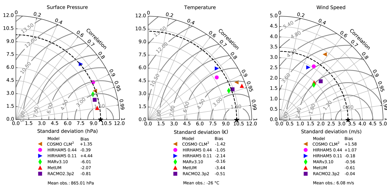
Figure 1. Taylor diagrams showing model performance compared to daily observations of surface pressure, near-surface temperature and observed wind speeds as well as the bias statistics for each model
