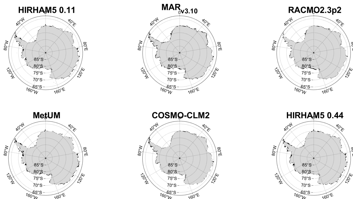
Figure A1. Each sub-figure shows where the common mask and the individual model masks are identical, grey is ice sheet or land in both masks. Black shows variation between model and common masks.
