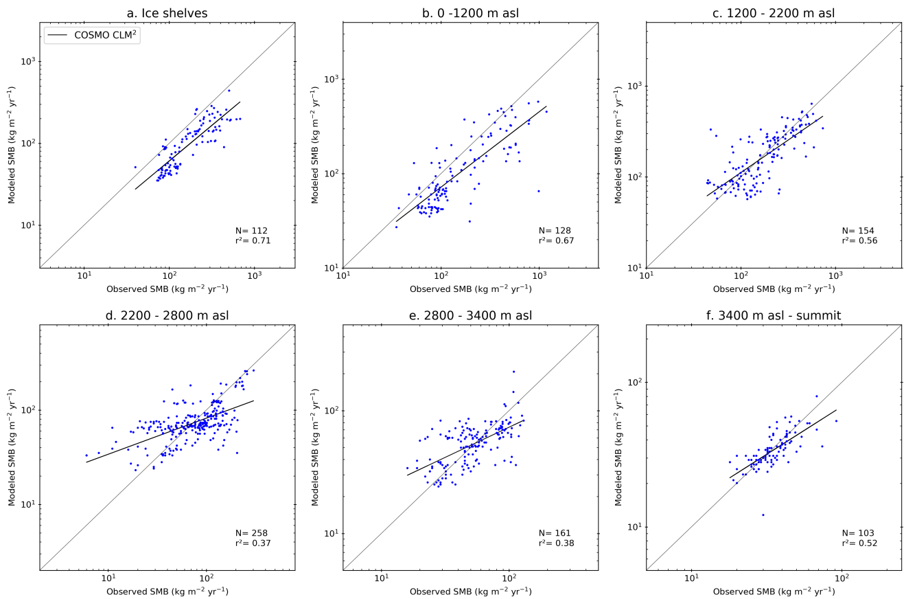
Figure A3. Comparison between COSMO-CLM 2 and observed SMB (units= kg m -2 yr -1 ) over the ice shelves (a) and by elevation classes (b-f). Due to the use of logarithmic axes, only positive values for the observed and modelled SMB from all the RCMs in this study are used (number for each bin N). Finally, the regression coefficient of each regression line is also shown (r 2 ).
