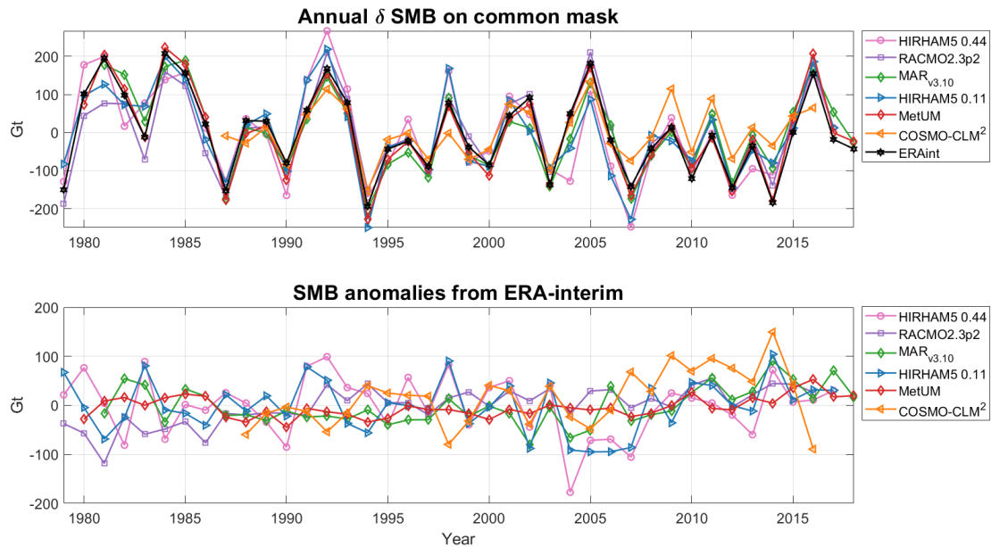
Figure 8. The upper figure shows the annual variability in surface mass balance over the common mask for each of the different RCMs, in the period 1979-2018. It is calculated by subtracting the respective model mean from each RCM's SMB time series. The bottom figure displays how modelled SMB from each RCM deviates from the ERA-interim SMB.
