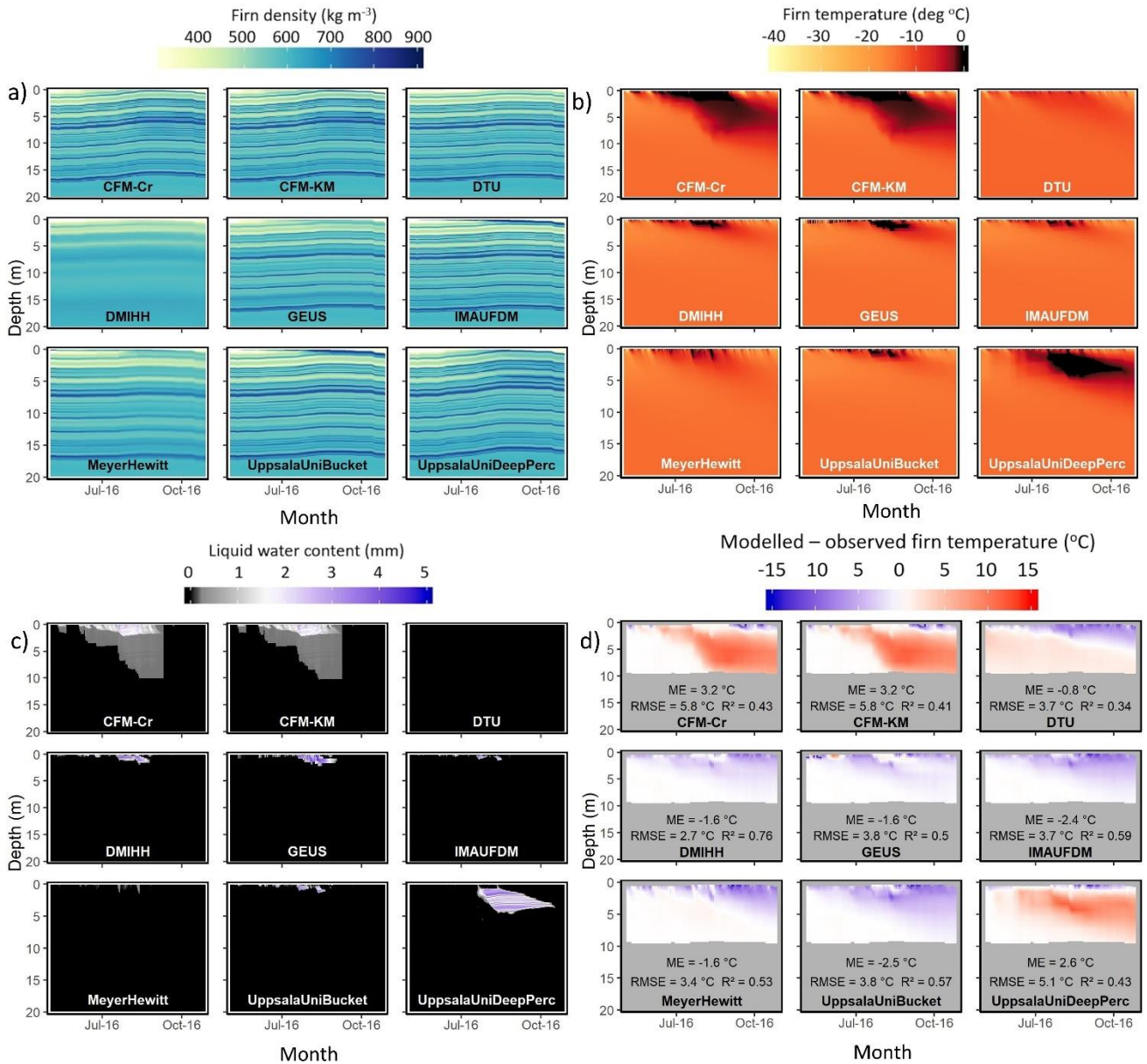
Figure 6: Simulated firn density (a), temperature (b), water content (note different y-axis) (c) and deviation between simulated and observed firn temperature (d) in Dye-2_16.
