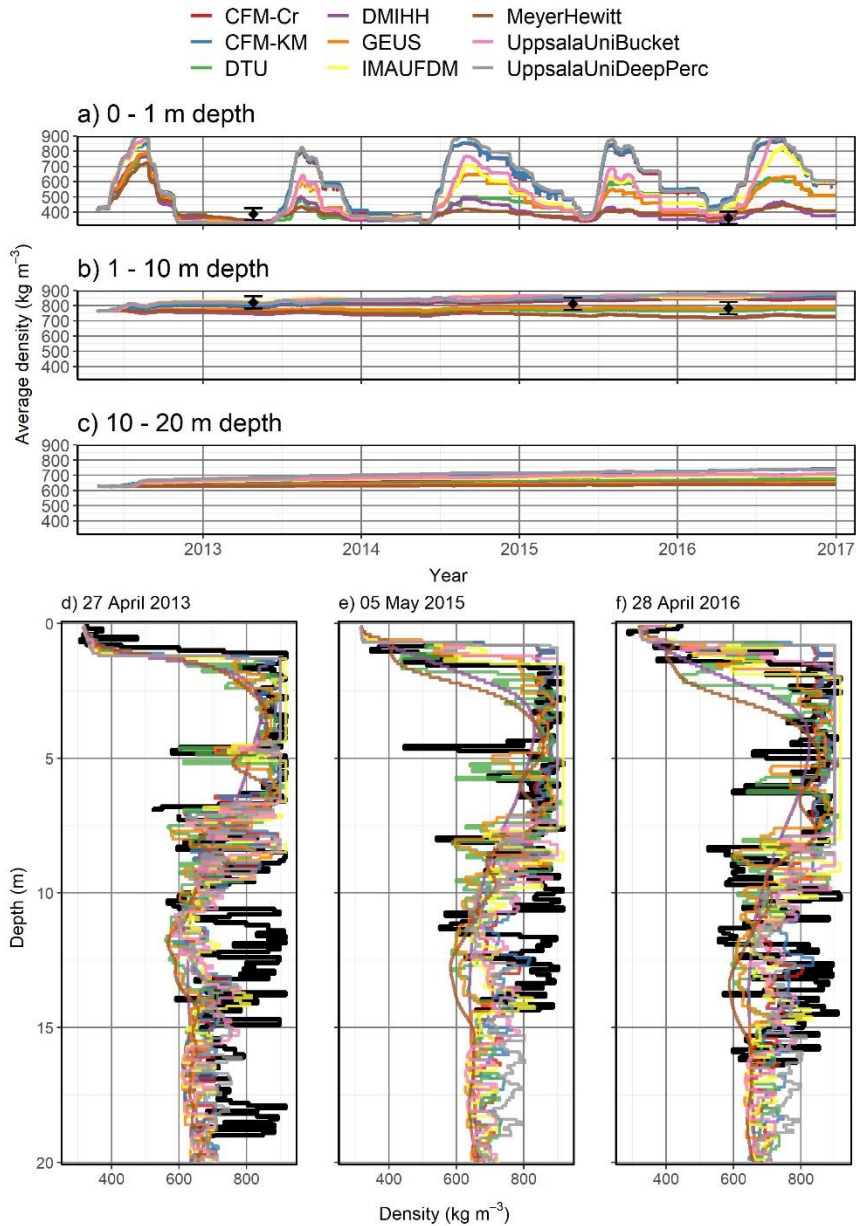
415 Figure 9: Modelled (colored lines) and observed (black dots with 40 kg m -3 uncertainty bars) average firn density for the top 1 m (a), for the 1-10 m depth range (b) and 10-20 depth range (c) at KAN_U. Observed and simulated density at KAN_U (d-f).
