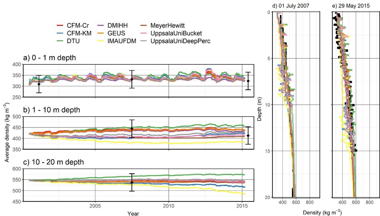
305 Figure 3: Modelled (colored lines) and observed (black dots with \pm 40 \text{ kg m}^{-3} uncertainty bars) average firn density for the 0-1 m (a), 1-10 m (b) and 10-20 m depth range (c) at Summit. Note the different density scales. Comparison of simulated and observed firn density profiles (d, e). In (e) the last modelled density profile, from 8 March 2015, is compared to an observation from 29 May 2015.
