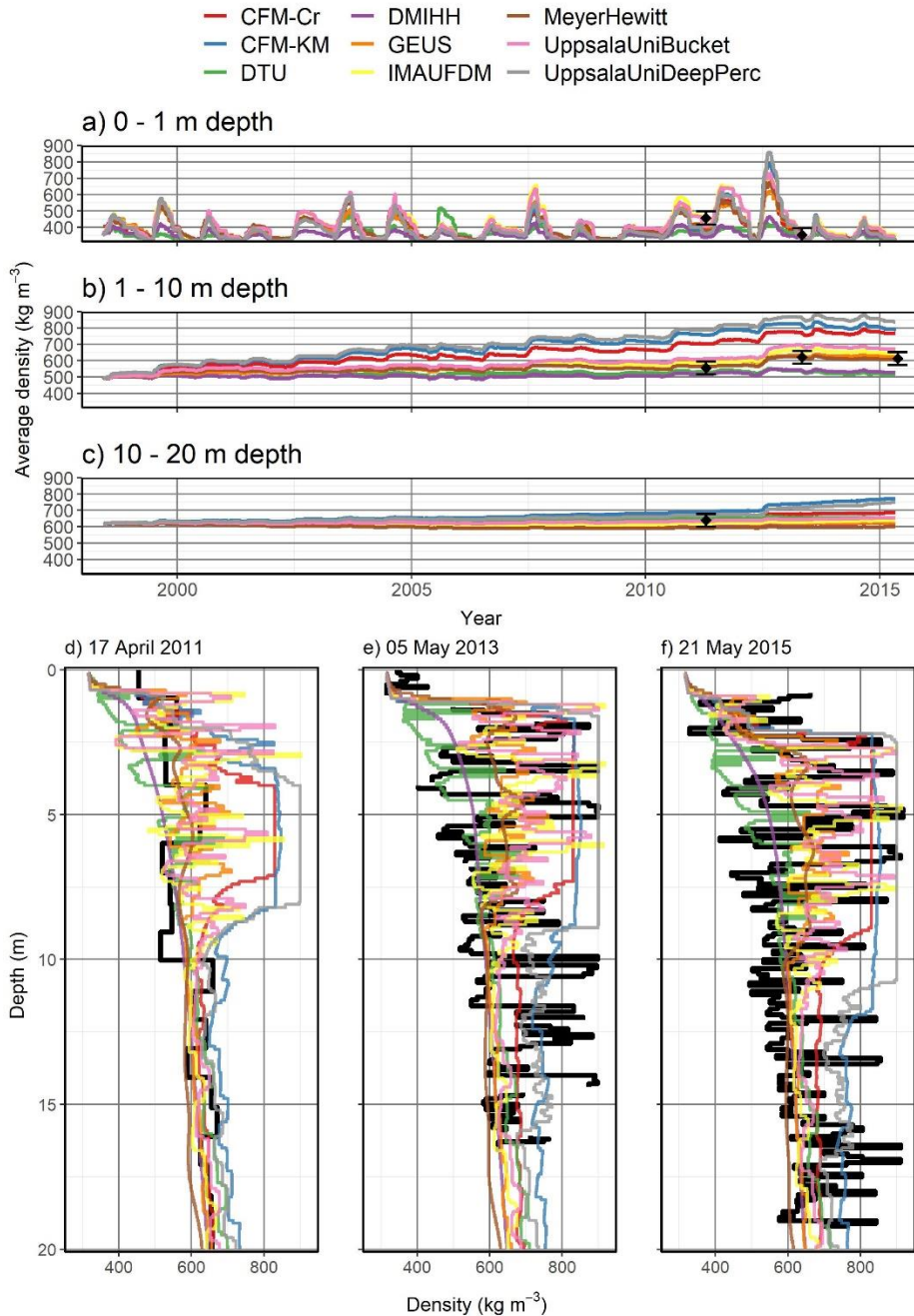
345 Figure 5: Modelled (colored lines) and observed (black dots with 40 \text{ kg m}^{-3} uncertainty bars) average firn density for the top 1 m (a), for the 1-10 m depth range (b) and 10-20 m depth range (c) at Dye-2_long. Observed and simulated vertical variability in density at Dye-2_long (d-f).
