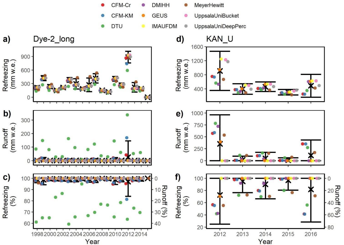
Figure 11. Yearly meltwater refreezing (a,d) or runoff (b,e), as totals (a,b,d,e) or fractions of the total meltwater input (c,f) at Dye-2 (a,b,c) and KAN_U (d,e,f). For each panel, yearly inter-model averages (black cross) and \pm 2\sigma values (error bars) are calculated from all models except the DTU model.
