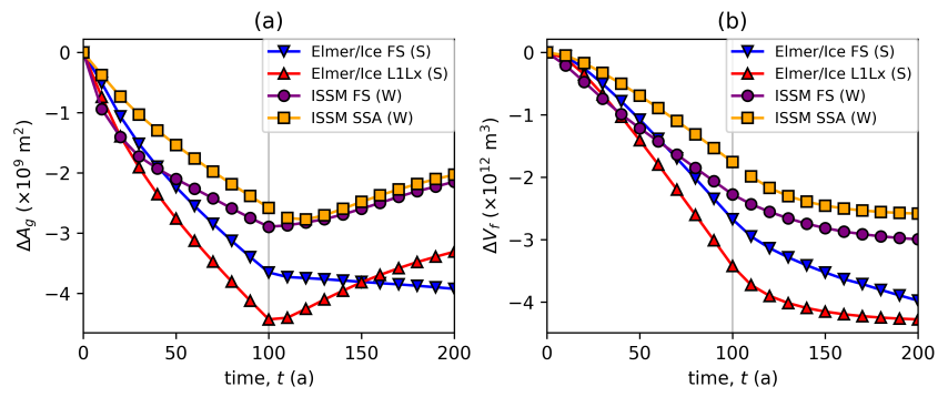
Fig. 1. Comparison of full Stokes and vertically integrated models in the Ice1r and Ice1ra experiments. Panel (a) shows the change in grounded area, panel (b) the change in volume above flotation.
