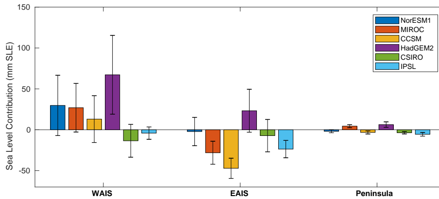
Figure 8. Regional change in volume above floatation (in mm SLE) for 2015–2100 from six CMIP5 model forcing under the RCP 8.5 scenario with median forcing, relative to ctrl_proj. Black lines show standard deviations.
