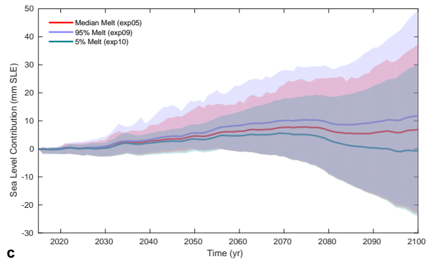
Figure 12. Impact of basal melt parameterization (a and c, 5 th -, 50 th - and 95 th - percentile values of \gamma_0 distribution) and calibration (b and d, “MeanAnt” and “PIGL” calibrations) on basal melt evolution (a and b, in Gt/yr) and ice volume above floatation (c and d, in mm SLE) relative to ctrl_proj over 2015–2100. Lines show the mean values and shaded background the simulations spread. Note that the y-axis differs in all plots.
