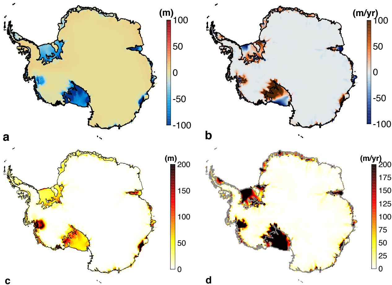
Figure 6. Mean (a and b) and standard deviation (c and d) of simulated thickness change (a and c, in m) and velocity change (b and d, in m/yr) between 2015 and 2100 under medium forcing from NorESM1-M RCP 8.5 scenario (exp01 and exp05) relative to ctrl_proj. .
