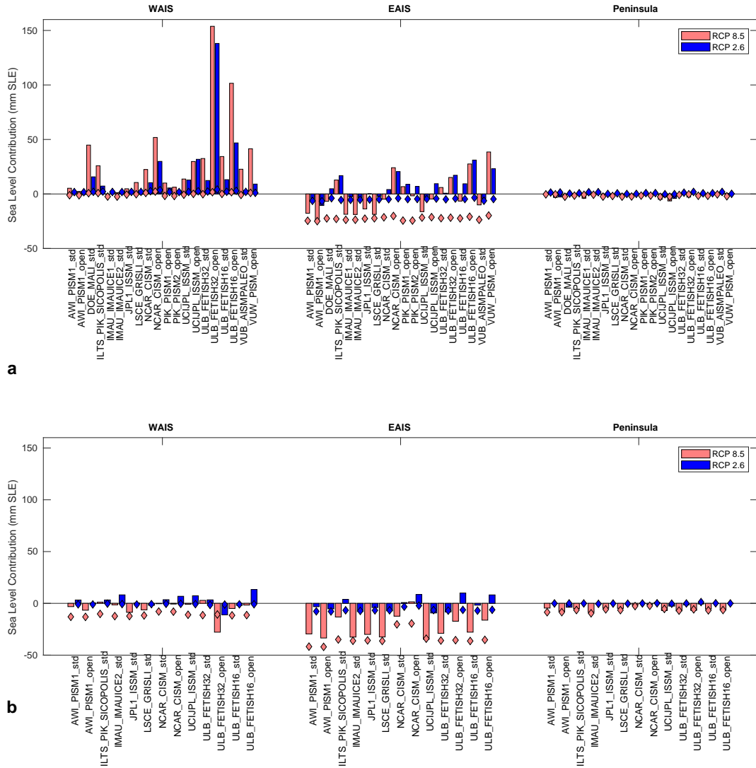
Figure 10. Regional change in volume above floatation (in mm SLE) and integrated SMB changes over the grounded ice (diamond shapes, in mm SLE) for 2015–2100 under RCP 8.5 (red) and RCP 2.6 (blue) scenario forcing from NorESM1-M (a) and IPSL (b) relative to ctrl_proj from individual model simulations.
