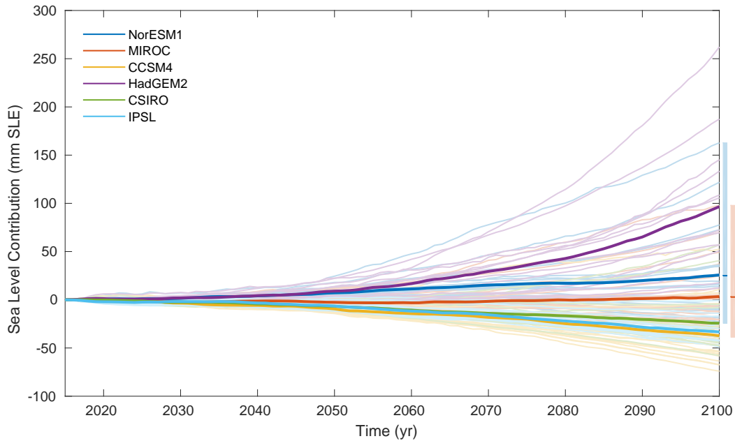
Figure 7. Evolution of ice volume above floatation (in mm SLE) over 2015–2100 period with medium forcing from the six CMIP5 models and RCP 8.5 scenario relative to ctrl_proj. Thin lines show results from individual ice sheet model simulations, and thick lines show mean values averaged for each CMIP5 model forcing. Bars on the right show the spread of results in ice flow models and mean values for the six CMIP5 forcings in 2100.
