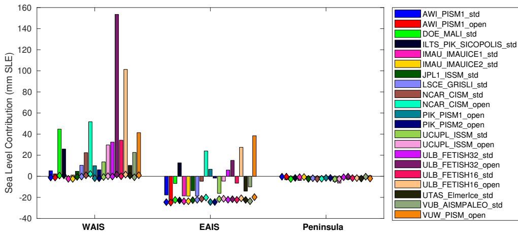
Figure 5. Regional change in volume above floatation (in mm SLE) and integrated SMB changes over the grounded ice (diamond shapes, in mm SLE) for the 2015-2100 period under medium forcing from NorESM1-M RCP 8.5 scenario (exp01 and exp05) relative to ctrl_proj.
