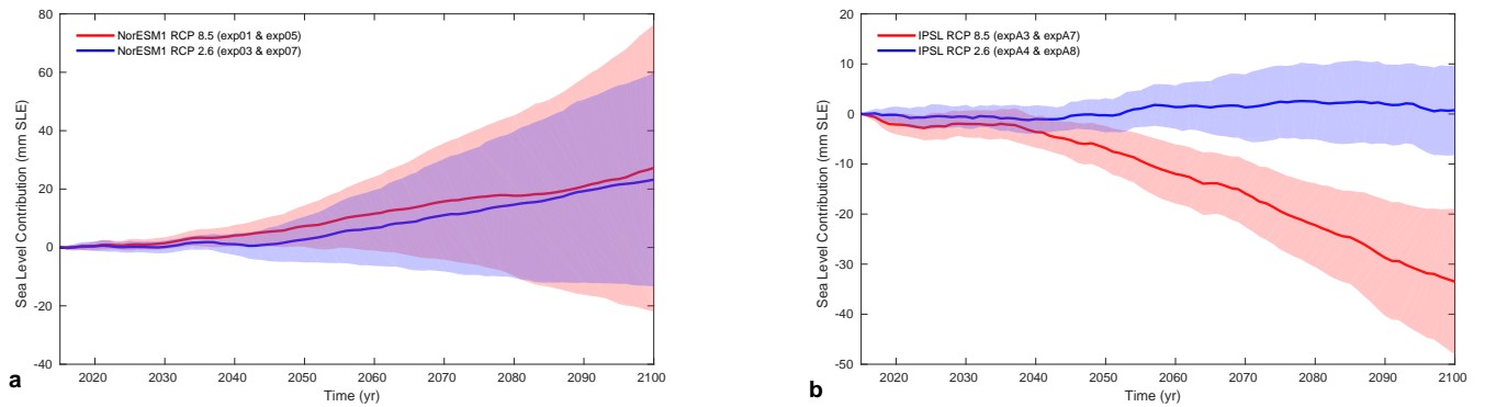
Figure 9. Impact of RCP scenario on projected evolution of ice volume above floatation for the NorESM1-M (a) and IPSL (b) models. Red and blue curves show mean evolution for RCP 8.5 and RCP 2.6, respectively, and shaded background the standard deviation.
