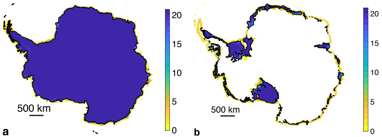
Figure 2. Total (left) and floating (right) ice extent at the beginning of the experiments (January 2015). Colors indicate the number of models simulating total ice (left) and floating ice (right) extent at every point of the 8-km grid. Black lines are observations of the total and floating ice extent, respectively (Morlighem et al., 2020).
