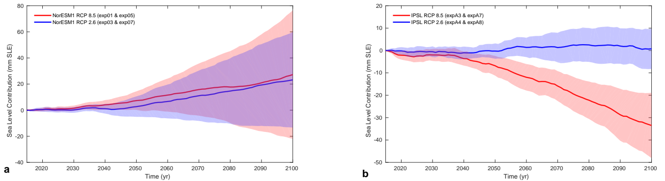
Figure 9. Impact of RCP scenario on projected evolution of ice volume above floatation for the NorESM1-M (a) and IPSL (b) AOGCMs models. Red and blue curves show mean evolution for RCP 8.5 and RCP 2.6, respectively, and shaded background the standard deviation.
