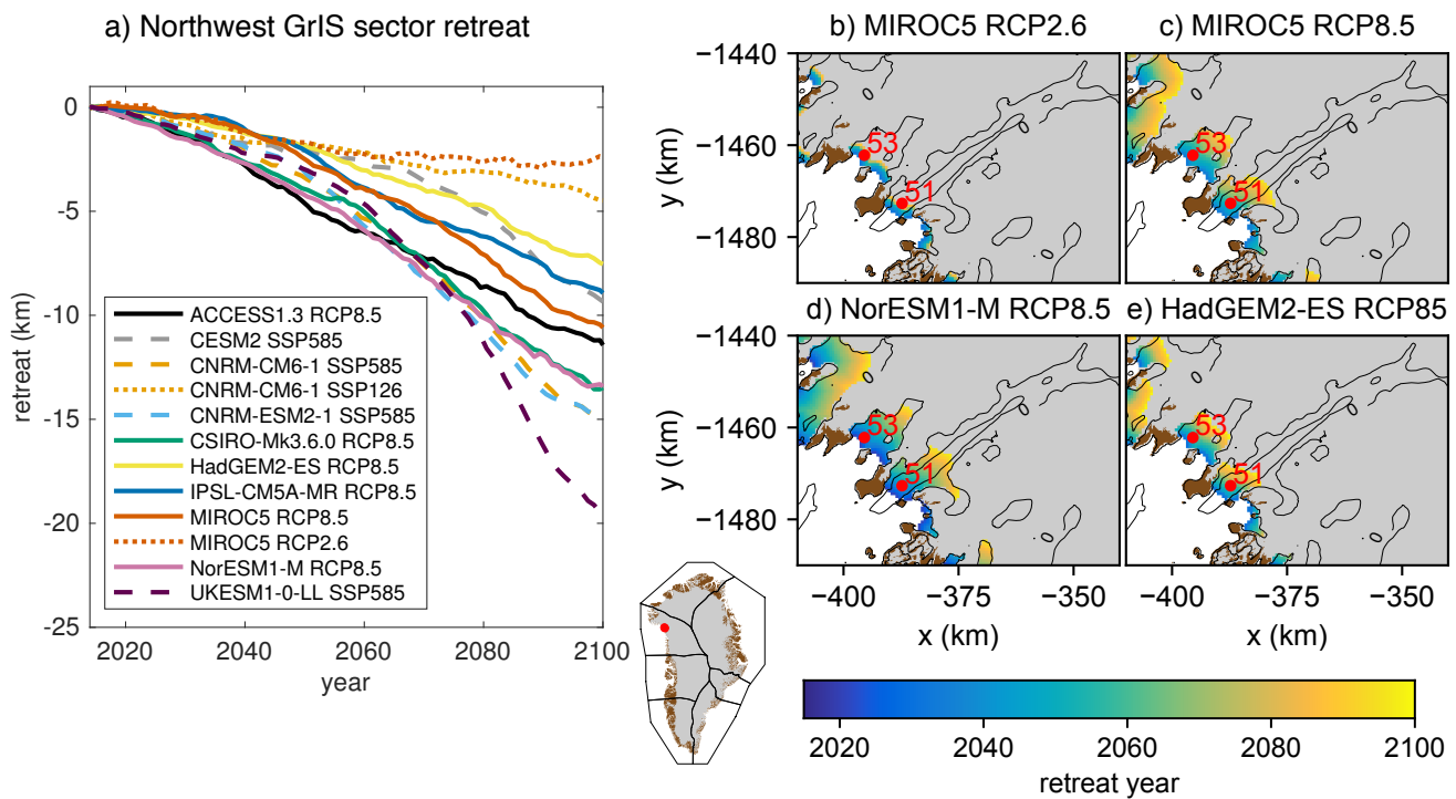
Figure 9: Retreat for selected Greenland ice sheet glaciers under the RCP2.6, RCP8.5, SSP1-2.6 and SSP5-8.5 scenarios. a) Time series of retreat over the 21 st century for the Northwest sector (adapted from Slater et al., 2019) and retreat from 2015 to 2100 for b) MIROC5 under RCP2.6, c) MIROC5 under RCP8.5, d) NorESM1-M under RCP8.5, and e) HadGEM2-ES under RCP8.5. The bedrock contour from Morlighem et al. (2017) is shown as black lines, gray indicates ice sheet mask. Red numbers indicate Kong Oscar Gletsjer (51) and unnamed glacier (53) discussed in the text.
