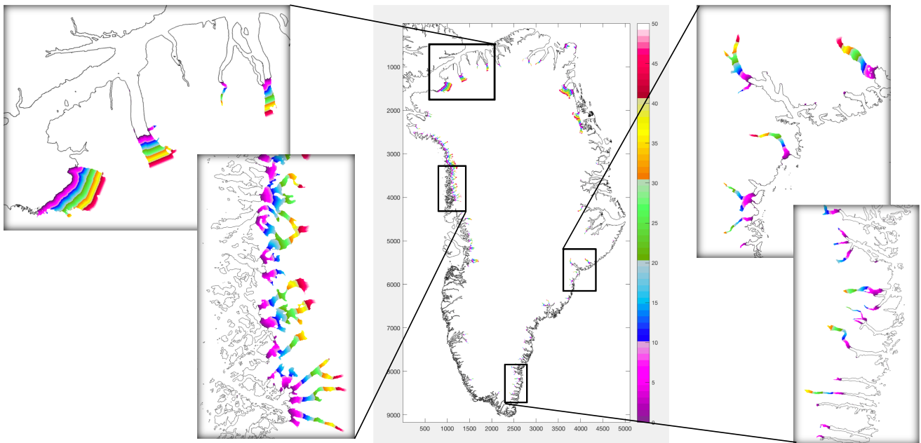
Figure D1. Distances from the ocean for all points identified as ice grounded on bed below sea-level in potential contact with the ocean. The data are masked to areas less than 50 km from the nearest grounding line.
