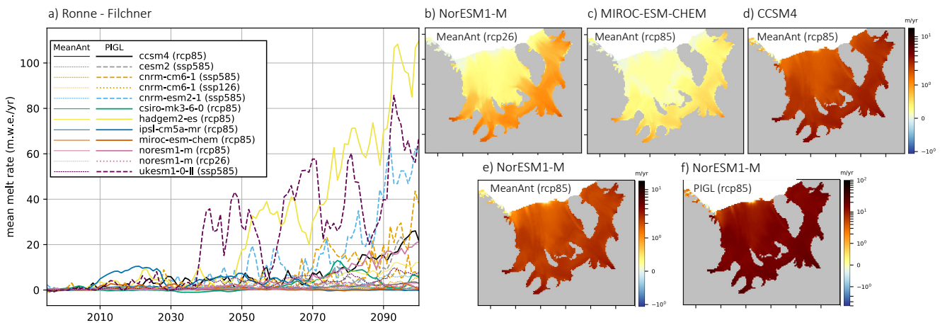
Figure 8. Mean cavity basal melt rates (m w.e./yr) under the RCP2.6, RCP8.5, SSP1-2.6 and SSP5-8.5 scenarios over the 21 st century for MeanAnt and PIGL calibrations and non-local parameterizations in the Weddell Sea Sector. a) Time series for Ronne-Filchner ice shelves obtained with MeanAnt (thin lines) and PIGL (thick lines) calibrations (adapted from Jourdain et al. (under review)). Spatial patterns of mean sub-shelf basal melt rate from 2081-2100 for the Tier 1 models assuming MeanAnt calibration for b) NorESM1-M under RCP2.6, c) MIROC-ESM-CHEM under RCP8.5, d) CCSM4 under RCP8.5., e) NorESM1-M under RCP8.5, and PIGL calibration for f) NorESM1-M under RCP8.5. The projections from the MeanAnt and PIGL calibrations assume that the ice shelf cavities have not evolved and are set to present day.
