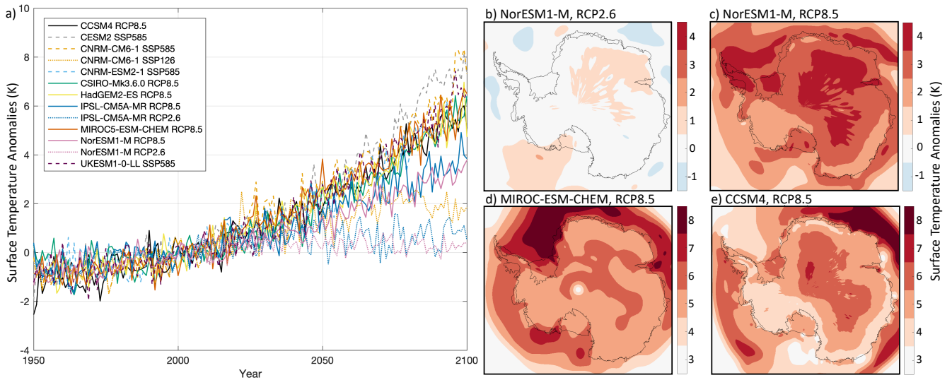
Figure 2: Surface temperature anomalies (K) over the Antarctic ice sheet under the RCP2.6, RCP8.5, SSP1-2.6 and SSP5-8.5 scenarios. a) Time series of mean surface temperature anomaly from 1950 to 2100 for all AOGCMs and scenarios selected, and (b-e) surface temperature anomaly over the time period 2081-2100 for b) NorESM1-M under RCP2.6, c) NorESM1-M under RCP8.5, d) MIROC-ESM-CHEM under RCP8.5, and e) CCSM4 under RCP8.5.
