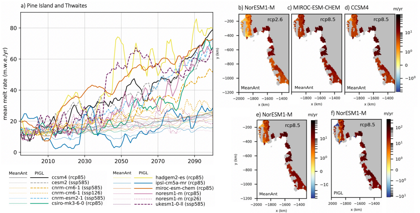
Figure 7. Mean cavity basal melt rates (m w.e./yr) under the RCP2.6, RCP8.5, SSP1-2.6 and SSP5-8.5 scenarios over the 21 st century for MeanAnt and PIGL calibrations and non-local parameterizations in the Amundsen Sea Sector. a) Time series for Pine Island and Thwaites ice shelves obtained with MeanAnt (thin lines) and PIGL (thick lines) calibrations (adapted from Jourdain et al. (under review)). Spatial patterns of mean sub-shelf basal melt rate from 2081-2100 for the Tier 1 models assuming MeanAnt calibration for b) NorESM1-M under RCP2.6, c) MIROC-ESM-CHEM under RCP8.5, d) CCSM4 under RCP8.5, e) NorESM1-M under RCP8.5, and PIGL calibration for f) NorESM1-M under RCP8.5. The projections from the MeanAnt and PIGL calibrations assume that the ice shelf cavities have not evolved and are set to present day.
