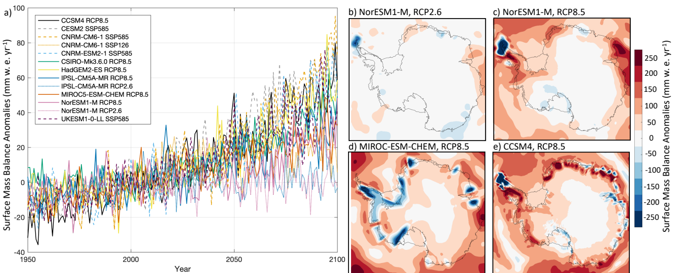
Figure 3: Surface mass balance anomalies (mm w. e. yr -1 ) over the Antarctic ice sheet under the RCP2.6, RCP8.5, SSP1-2.6 and SSP5-8.5 scenarios. a) Time series of mean surface mass balance anomaly from 1950 to 2100 for all AOGCMs and scenarios selected, and (b-e) mean surface mass balance anomaly over the time period 2081-2100 for b) NorESM1-M under RCP2.6, c) NorESM1-M under RCP8.5, d) MIROC-ESM-CHEM under RCP8.5, and e) CCSM4 under RCP8.5.
