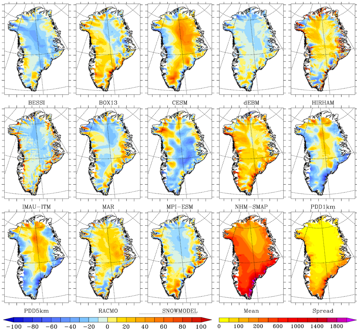
Fig. 4: Same as Fig 2 but for the modelled snowfall (linearly interpolated on the 1 km common grid but without any elevation correction) vs the ensemble model mean over 1980-2012 as a percentage of the ensemble model mean of snowfall accumulation. The ensemble mean and models spread around the mean are also shown in mmWE/yr in the two last plots.
