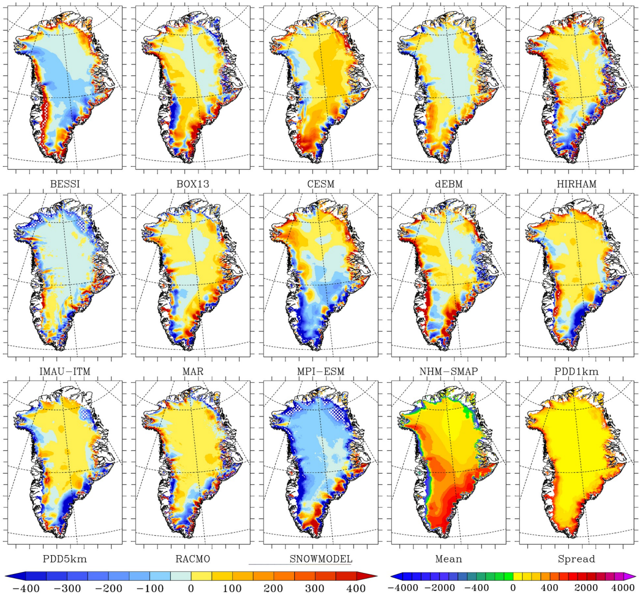
1160 | Fig. 2: Same as Fig 1 but for the modelled SMB vs the ensemble model mean over 1980-2012 (shown in the 2 last plots). As Fig. 1, the areas listed in Table 4 where SMB disagrees with the MODIS-derived bare ice area are shown in hatch.
