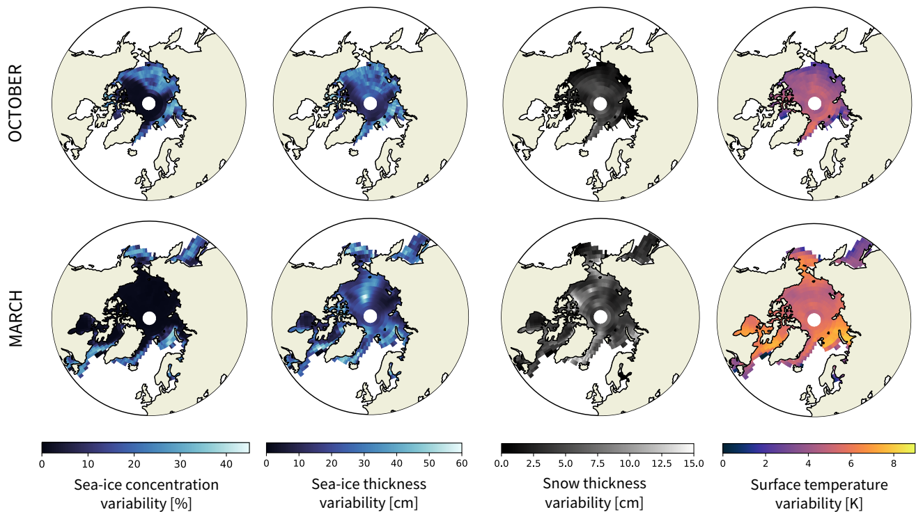
Figure B1. Time mean of the standard deviation for each date over a sample of five years (2003 to 2008), for each variable and each grid cell. This standard deviation was the variability estimate used to modulate the input variables in the sensitivity studies of Sec. 4.3.2. These values are inferred from the SICCI2 assimilation run.
