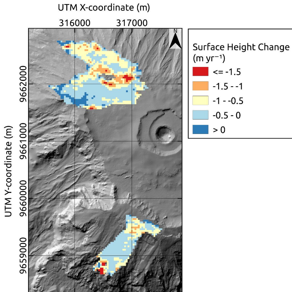
Supplementary Figure 2: Spatial distribution of mean annual surface height change (m) from 2000-2011. The mean annual surface height change was generated from the difference between the SRTM DEM (2000) and the TanDEM-X DEM (2011). Background: hillshade of the KILISoSDM (Sirguy and Cullen 2013).
