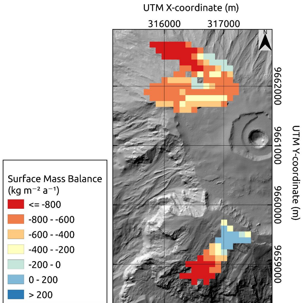
Supplementary Figure 1: Spatial distribution of the mean annual surface mass balance ( \text{kg m}^{-2} ) from 2005-2013 generated with the distributed, physically-based MB model by Mölg et al. (2008, 2009a). Background: hillshade of the KILISoSDM (Sirguy and Cullen 2013).
