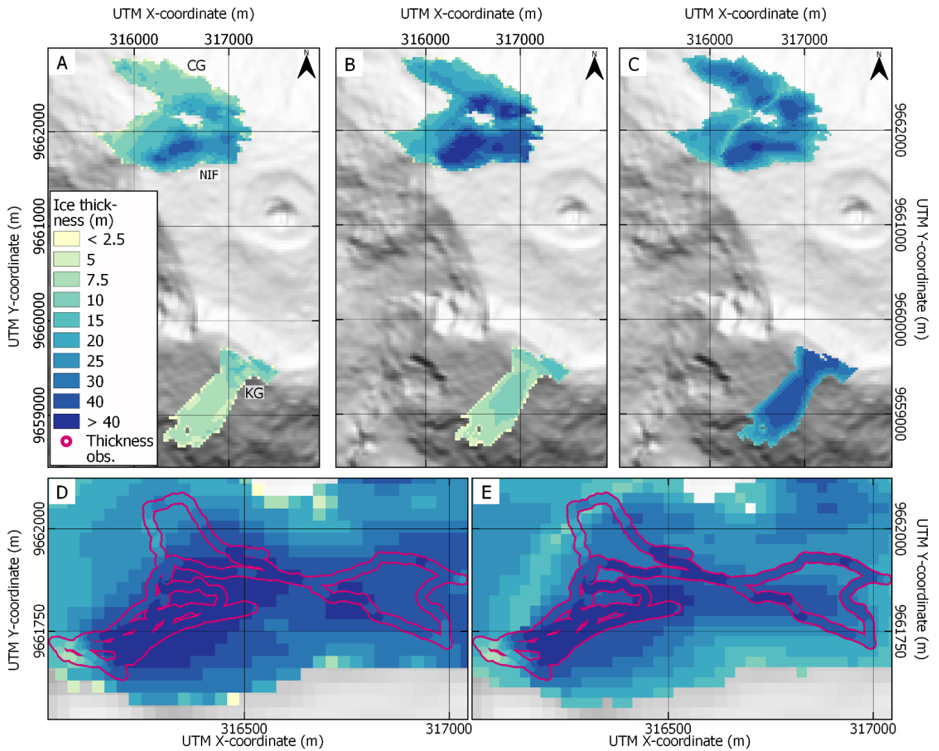
295 Figure 2: Reconstructed ice thickness (m) for Northern Icefield (NIF) and Kersten Glacier (KG) for the year 2000. Panel (A) shows results for Experiment 1 making exclusive use of past thickness information in nowadays ice-free areas. Panel (B) presents results from Experiment 2, which uses a bulk viscosity inferred from the retreat information on KG, whereas for NIF, the reconstruction is only calibrated by in-situ GPR measurements (see Table 1). As comparison panel (C) depicts the composite ice thickness from Farinotti et al 2019. Panel (D) shows a closeup of NIF, overlying the thickness map of Experiment 2 with the GPR thickness measurements (magenta contour, showing measured values in the same colourbar) by Bohleber et al. (2017). Panel (E): same as Panel (D) but showing the consensus thickness map (Farinotti et al., 2019; cf. Panel C). Background: SRTM DEM hillshade.
