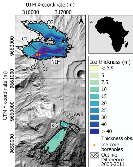
380 Figure 1: Reconstructed ice thickness (m) for Northern Icefield (NIF) and Kersten Glacier (KG) for the year 2011, based on thickness observations (NIF) and mean viscosity (KG) with a model resolution of 2 m (Experiment 3). The magenta path on NIF represent the GPR ice thickness measurements by Bohleber et al. (2017). The orange dots (C1-C3) indicate the drill locations of the ice cores from Thompson et al. (2002). The AWS location from Mölg et al. (2009) is marked by the white triangle. Background: KiliSoSDEM hillshade. The overview map depicts the location of Mt. Kilimanjaro (white cross) on the African continent.
