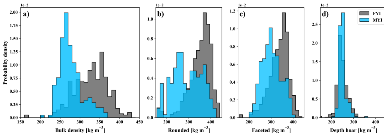
710 Figure 7: Bulk density (vertically integrated) derived from SMP profiles on first year (FYI, n = 402 ) and multiyear (MYI, n = 211 ) sea ice (a). Automated profile classification was used to separate the high vertical resolution (2.5 mm) estimates of snow density and produce layer-type distributions for rounded (b), faceted (c) and depth hoar (d) classes.
