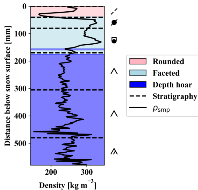
Figure 6: Automated layer-type classification of a SMP profile collected on sea ice where colours indicate classification result. Horizontal dashed lines indicate heights of snow pit observed stratigraphic layers at the same location. Snow layer classification follows standardized colours and symbols described in Fierz et al., (2009).
