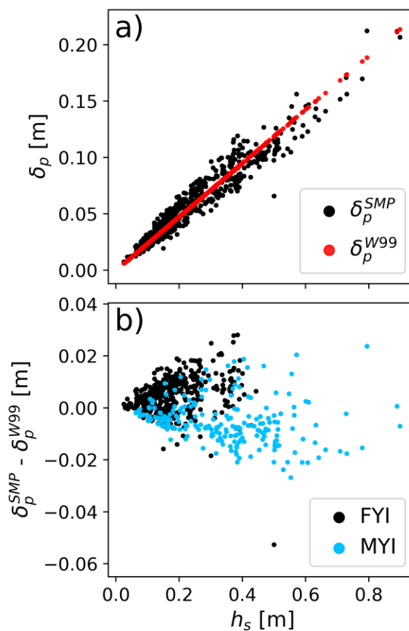
730 Figure 11: Changes in estimated radar propagation bias ( \delta_p ; a) relative to snow thickness ( h_s ) based on density estimated from climatology ( \delta_p^{W99} ) and measured from SMP profiles ( \delta_p^{SMP} ). The two sets of estimates were subtracted to show potential errors associated with the use of climatology over known snow densities (b).
