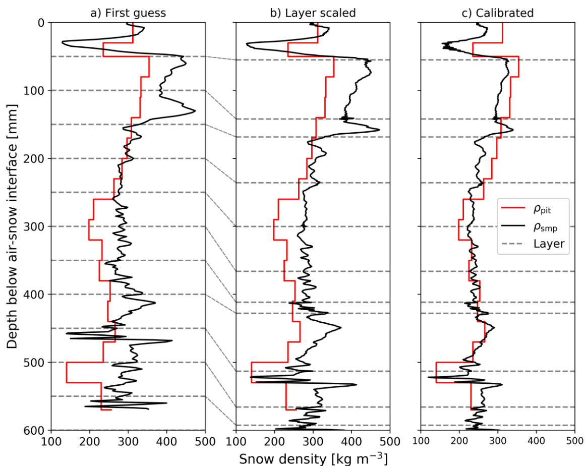
Figure 3: SMP processing steps where first guess estimates of \rho_{smp} (a; black lines) are used to improve alignment with snow pit measurements of density (b; red lines) prior to recalibration and computation of final estimates (c). To begin alignment SMP profiles are divided into arbitrary 5 cm layers (dotted lines) and scaled randomly in thickness. Best fit alignment is selected where RMSE between the SMP estimates and snow pit measurements are minimized. The matching process accounts for differences in the target snowpack due to the 10 cm separation between profiles. The example shown is for Eureka site 5 on MYI.
