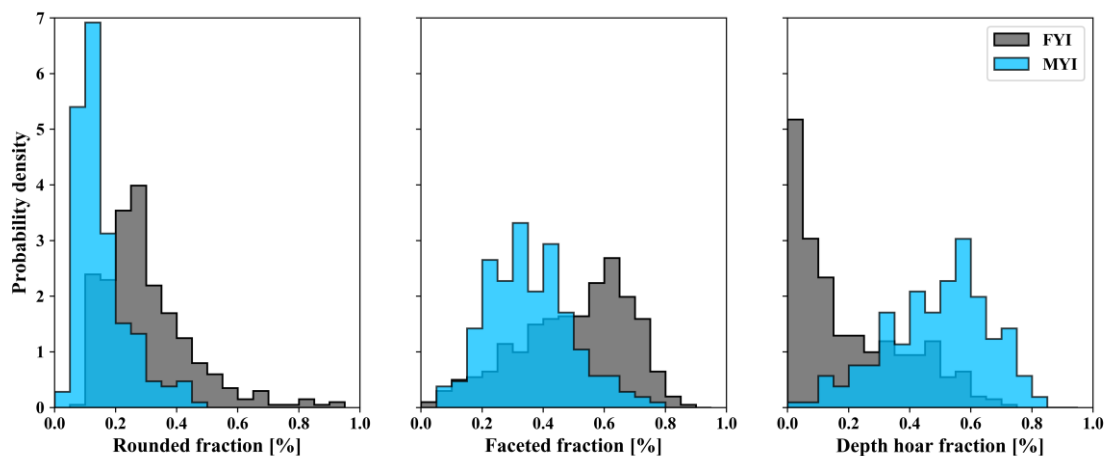
715 Figure 8: Fractional snowpack composition by rounded, faceted, and depth hoar layers from the SMP profiles on first year (FYI) and multiyear (MYI) sea ice. Classification methods for the SMP are described in Sect. 3.4.
