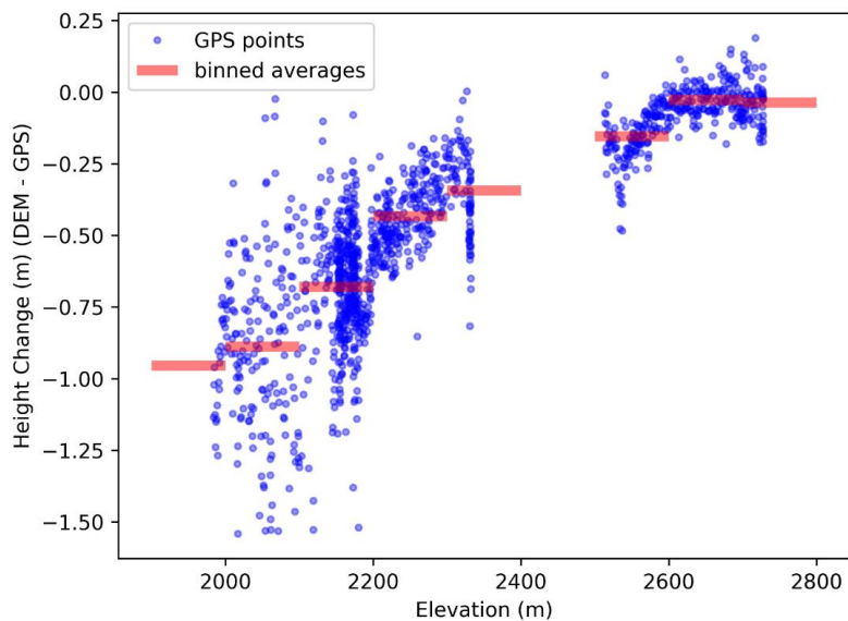
110 Figure S5: Zillmer Glacier kinematic GPS survey points subtracted from the subsequent ALS survey. The survey points were collected on August 12, 14 and 16, 2016 while the ALS survey was conducted on September 14, 2016. Height change points are averaged over 100 m elevation bands, and then assigned a density based upon surface classification from satellite observations to convert height change to water equivalent. Glaciological data are then corrected with this data. Data between 2300-2500 m not shown as the base-station unit failed during this portion of surveying. Typically, time between GPS surveys and LiDAR acquisition was between 0-21 days.
