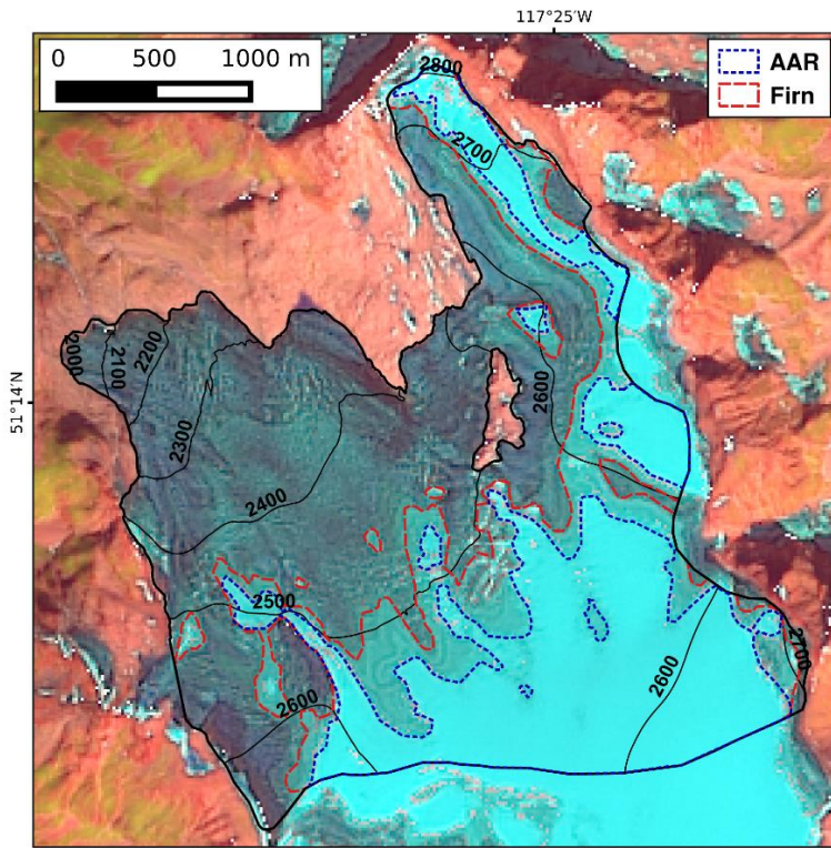
90 Figure S1: Surface classification of the Illecillewaet Glacier with a pan-sharpened Landsat 8 image from August 12, 2015. Firn area, and accumulation area are shown, with the remainder of the glacier (black outline), classified as ice.
