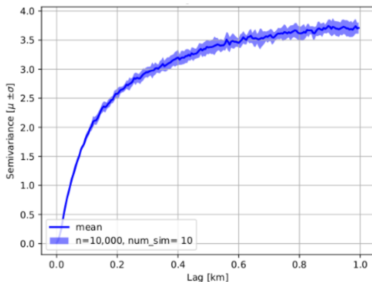
Figure S3: Example semi-variogram for Conrad Glacier, winter 2018. The variogram was constructed using 10,000 random samples over 10 simulations. Decorrelation length was defined as the distance at which semivariance becomes asymptotic (5% change threshold), 900 m in this example.
