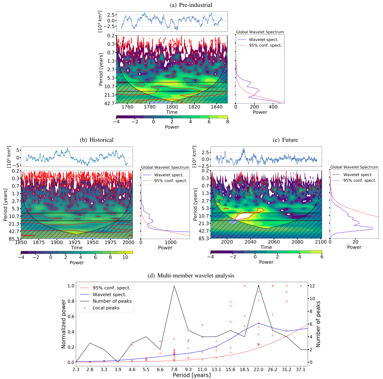
Figure 1. Wavelet analysis applied to the Arctic sea ice volume anomaly over the pre-industrial (200 years preceding the historical integration) (a), historical (1850-2005) (b) and future (2006-2100) (c) periods. Each subfigure (a-c) presents the sea ice volume anomaly time series (top), wavelet power spectrum (bottom-left), and time-integrated power spectrum from the wavelet analysis (bottom-right). Morlet is used as a wavelet mother. The red lines denote the 95% significance levels above a red noise background spectrum, while the crosshatched areas indicate the cone of influence where edge effects become important. White areas in the wavelet power spectrum are representing values out of the range defined by the color bar. Horizontal black lines depict the 8 and 16-year periods. Multi-members wavelet analysis (d). The red dots depict wavelet spectrum local maxima for all members. The blue and dashed red lines show the mean normalised wavelet spectrum and 95% confidence spectrum for all members, respectively. The black line represent the number of wavelet spectrum local maxima at each period.
