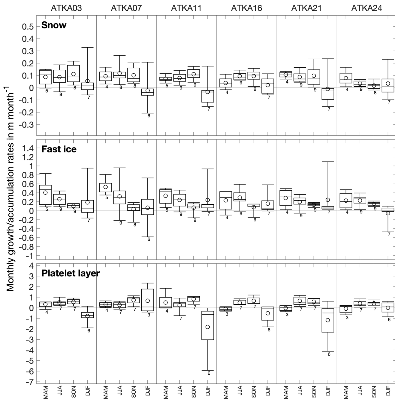
26 Figure 6: Seasonal snow, sea-ice and platelet-layer accumulation/growth and melt rates separated for austral fall (March, 27 April, May; MAM), winter (June, July, August; JJA), spring (September, October, November; SON), and summer (December, 28 January, February; DJF) for each ATKA sampling point for the study period from 2010 to 2018. Boxes are the first and third
