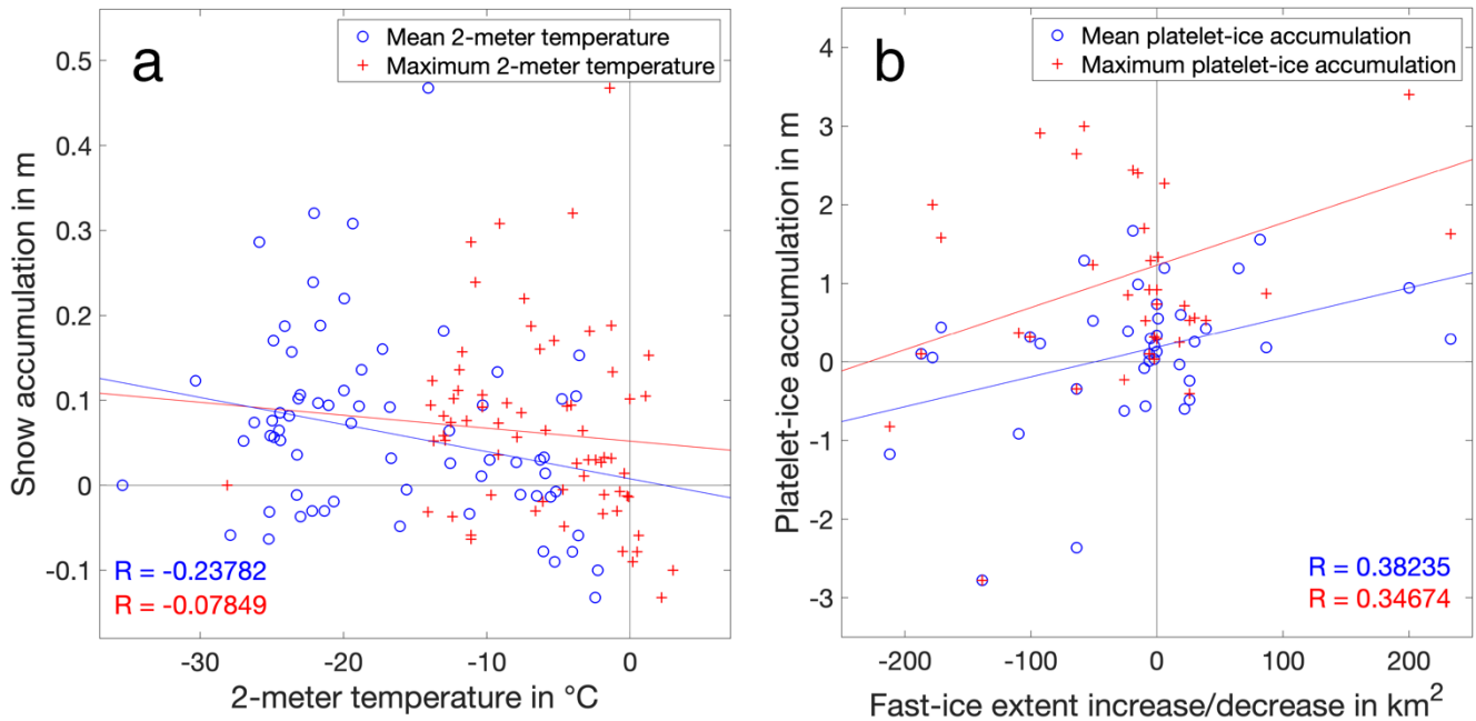
22 23 Figure 8: Scatter plot comparing (a) the average 2-meter air temperature (see Section 2.4) and the snow accumulation between 24 two consecutive surveys, and (b) increasing (positive values) and decreasing (negative values) fast-ice extent and platelet- 25 layer thickness between two consecutive surveys. The analysis includes all measurements at all sampling sites throughout the 26 study period from 2010 to 2018. Blue circles and red crossed denote the respective mean and maximum values within the time 27 frame between the consecutive measurements. Colored solid lines in Figure (b) show the linear regression between both 28 parameters with the respective correlation coefficients R. 29
