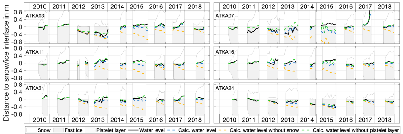
89 Figure 5: Close-up of Figure 4 which highlights the location of the water level with respect to the snow/ice interface (which 90 has the opposite sign of the freeboard) as measured in the field (black solid line) and as calculated according to Equation 1.1 91 and 1.2 including snow and platelet-layer thickness (blue dashed line), neglecting the snow cover (dashed yellow line) and 92 platelet layer (dashed green line), respectively. Please note that, for the purpose of better illustration, we depict here the actual 93 location of the water level rather than the freeboard (the only difference being the opposite sign). This means that, if the water 94 level is above the snow/ice interface, this is depicted in the figure accordingly, while the actual freeboard carries a negative 95 sign, and vice versa. The reference depth of 0 represents the snow/ice interface.
