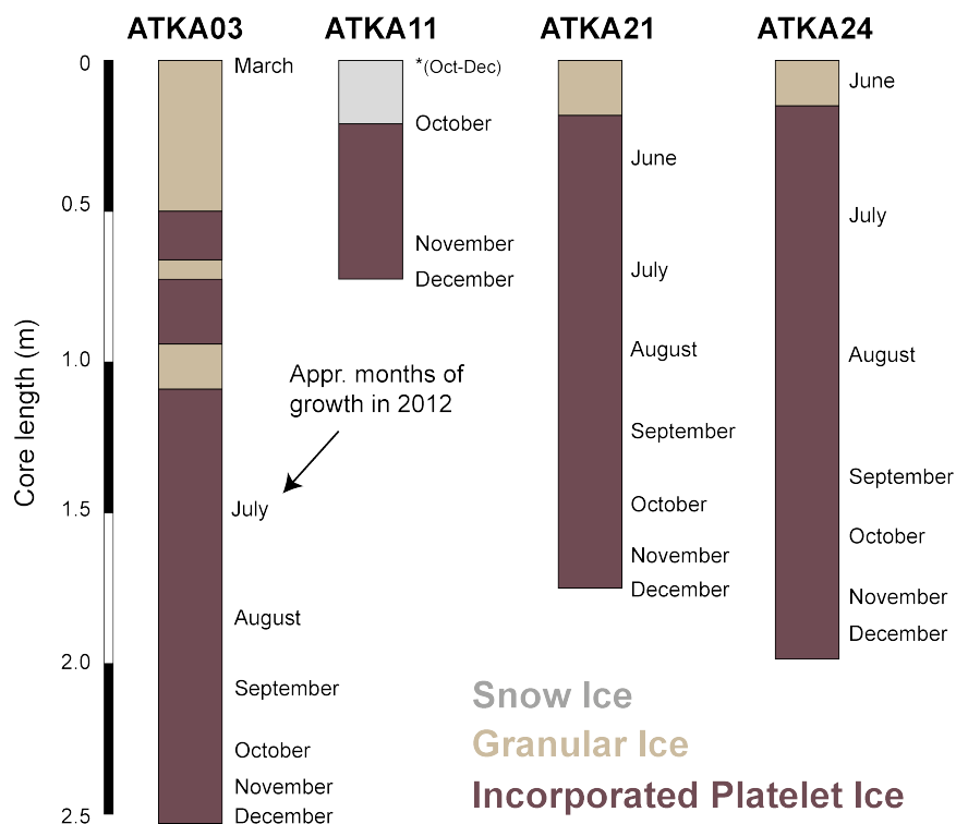
60 61 Figure 9: Sea-ice crystal fabric from ice cores obtained at four different fast ice sampling sites in December 2012, derived 62 from vertical and horizontal thin sections (0.1m spacing) along the full core length (see also Hoppmann et al., 2015a; 63 Hoppmann et al., 2015b; Hoppmann, 2015).
