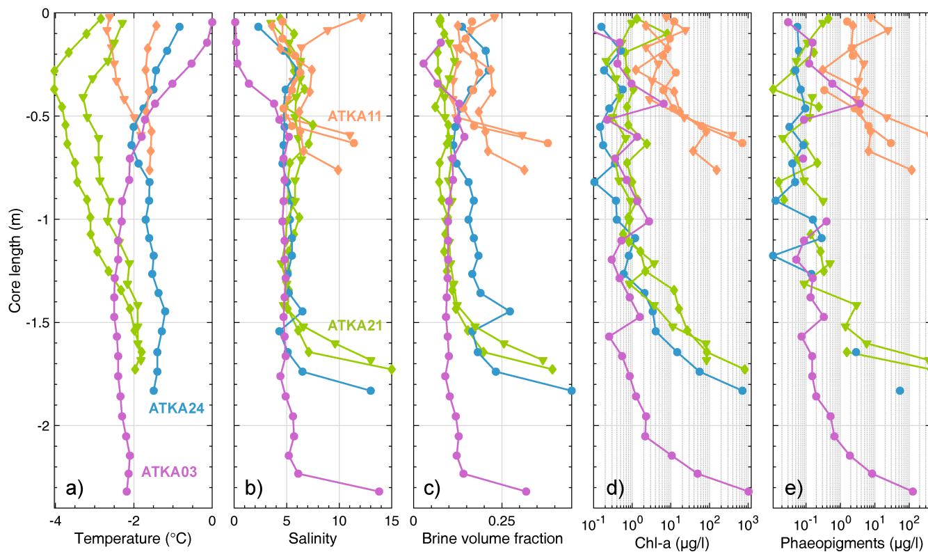
78 Figure 10: Sea-ice physical and biological properties from cores obtained at different fast ice sampling sites in Nov/Dec 2012 79 (after Hoppmann et al., 2013).
