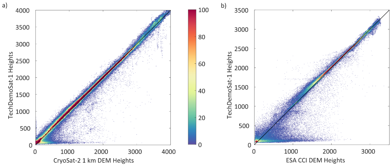
Figure 3: Density plot comparing height estimations from TechDemoSat-1 over a) Antarctica and b) Greenland and co-located data from the CryoSat-2 v1 1 km DEM (Slater et al., 2018) and GL-CCI respectively. With 1:1 reference line (black)
