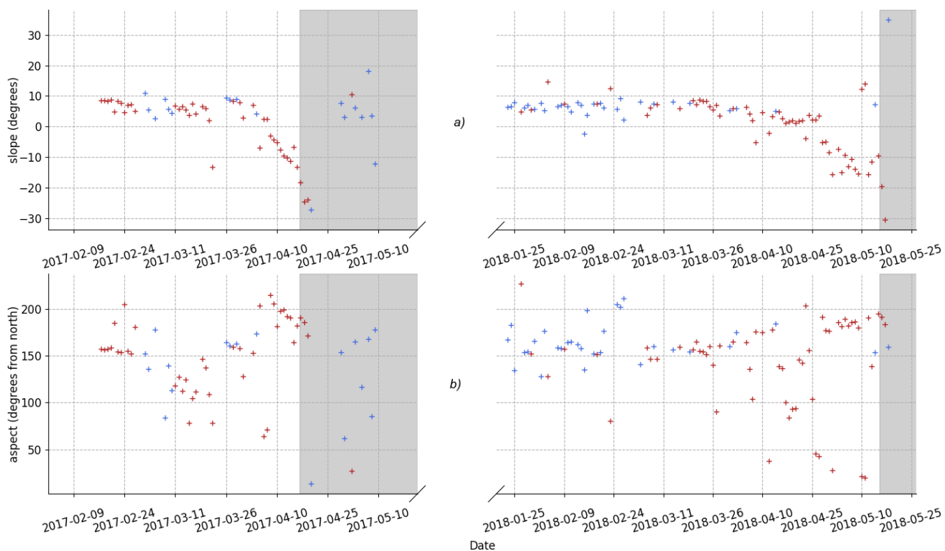
Figure A2. Estimation of the slope (a) and aspect (b) of the snow surface under Autosolexs sensor. The estimation is more robust for low solar elevations and low near-surface AEC. Grey shading corresponds to areas with less than 20 cms of measured snow depth.
