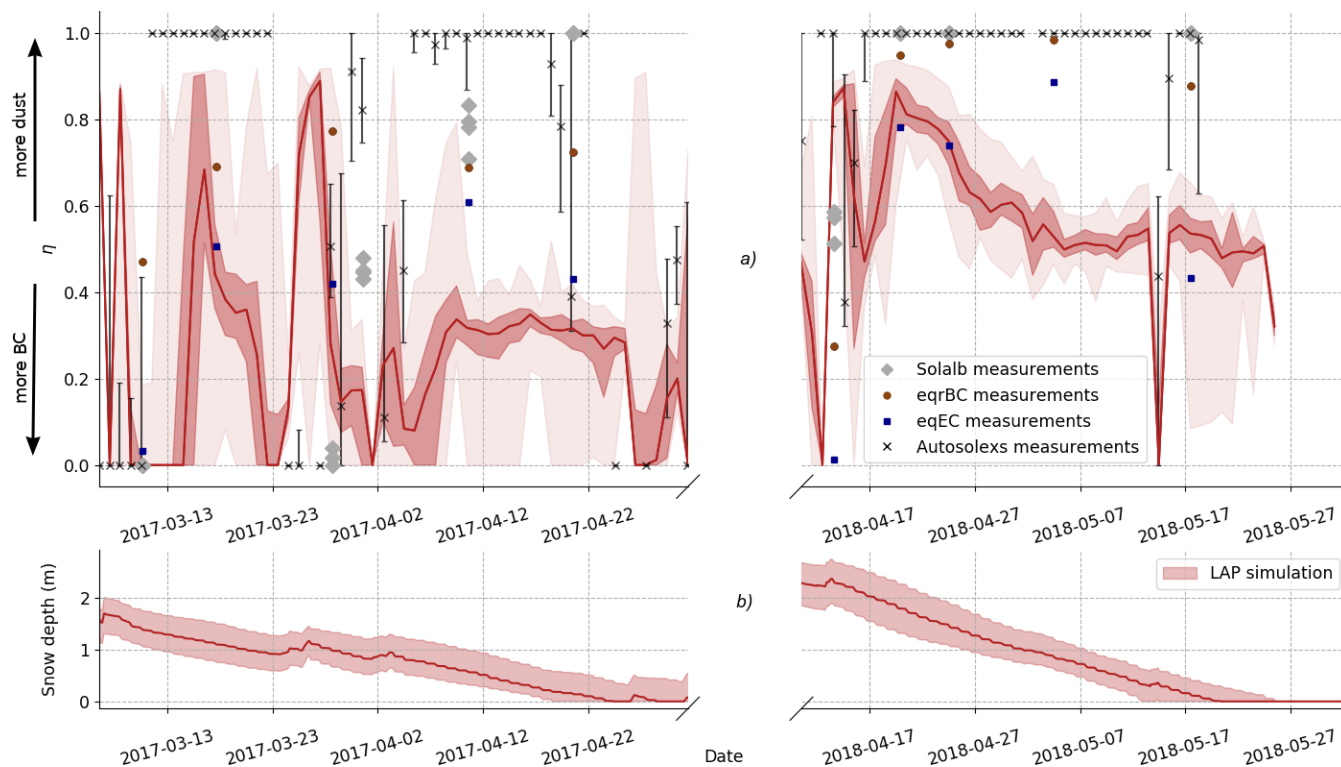
Figure 8. a) Evolution of measured and simulated \eta – i.e. the portion of LAP radiative impact caused by dust during the final ablation period. \eta values estimated from the LAP simulation is represented in red, with light shading corresponding to the full ensemble and darker shading corresponding to the first and third quartiles of the ensemble. Information retrieved from automatic spectral albedo are represented by black crosses with error bars corresponding to the 25 and 75 % quartiles of all the measurements of the day. Information retrieved from manual spectral albedo are represented by grey diamonds. Chemical measurements of eqEC (EC+dust) and eqrBC (rBC+dust) are represented in dark blue and brown respectively. The results are put in comparison to the snow depth (b). The major dust deposition event of the second year is represented by brown shading.
