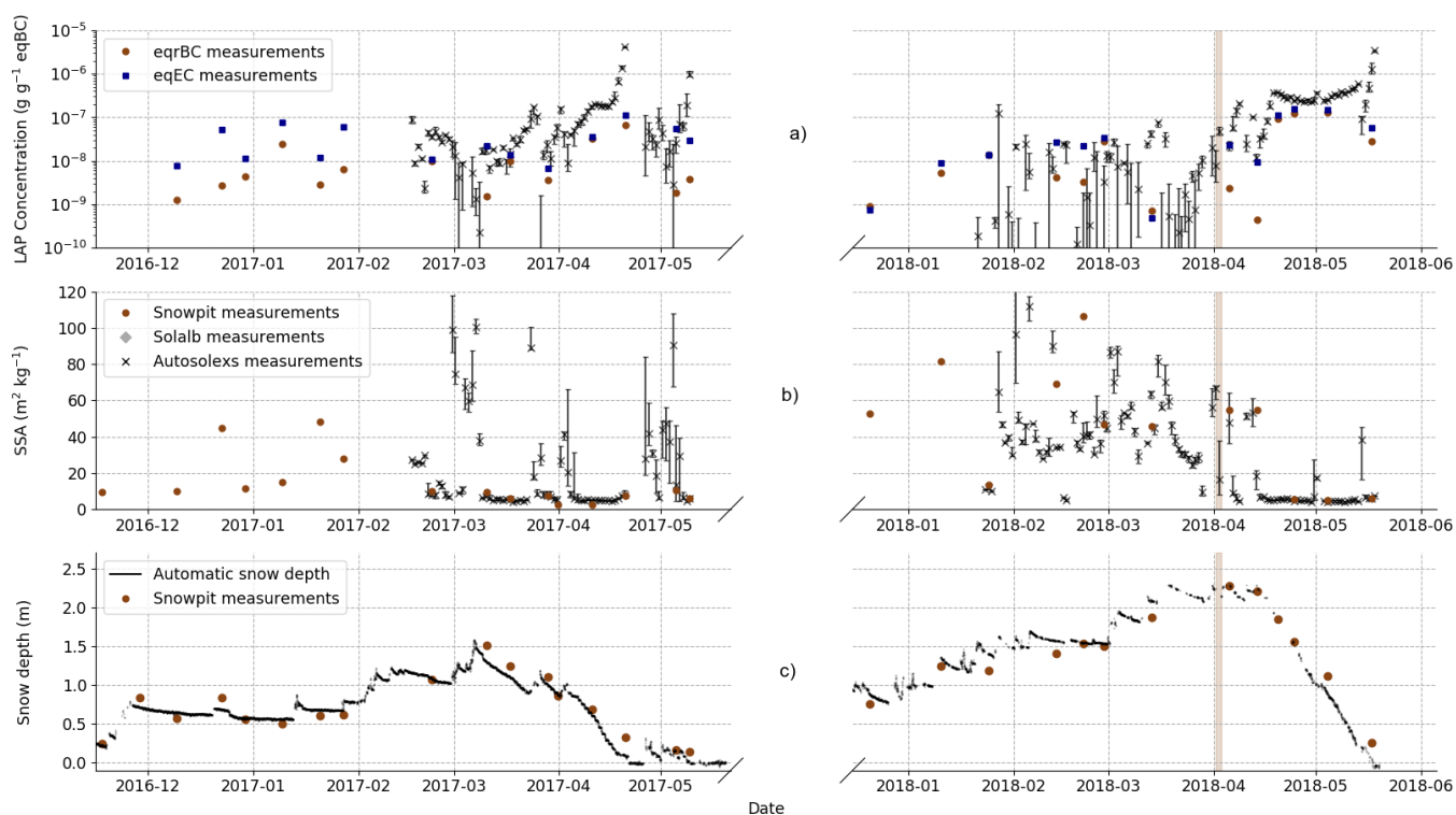
Figure 3. Evolution of measured near-surface LAP concentration (a), near-surface SSA (b) and snow depth (c). Information retrieved from automatic spectral albedo (Autosolexs) are represented by black crosses with error bars corresponding to the 25 and 75% quantile of all the measurements of the day. Information retrieved from manual spectral albedo (Solalb) are represented by grey diamonds. Snowpits SSA and eqrBC concentrations are represented by brown dot and eqEC concentrations are represented by blue squares. The major dust deposition event of the second year is represented by the vertical brown shading.
