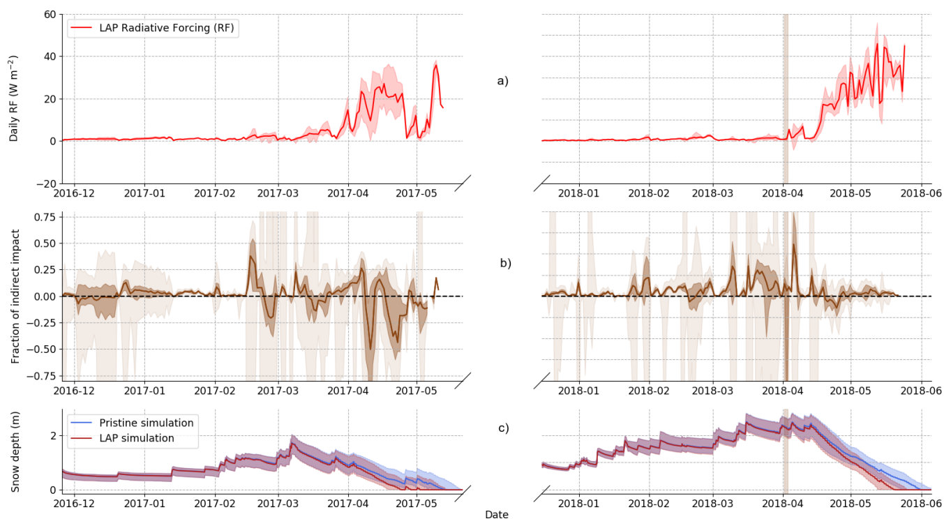
Figure 6. a) Evolution of daily radiative forcing (RF) due to LAPs. This RF is computed as the difference of energy absorbed by the snowpack between the LAP and pristine simulations. b) Evolution of the daily fraction of the indirect impact ( r_{ind} ), the opaque shadowing corresponds to the ensemble members between the first and third quantile whilst the light shadowing is the full ensemble spread. c) Simulated snow depth for the pristine and the LAP simulations. The major dust deposition event of the second year is represented by brown shading.
