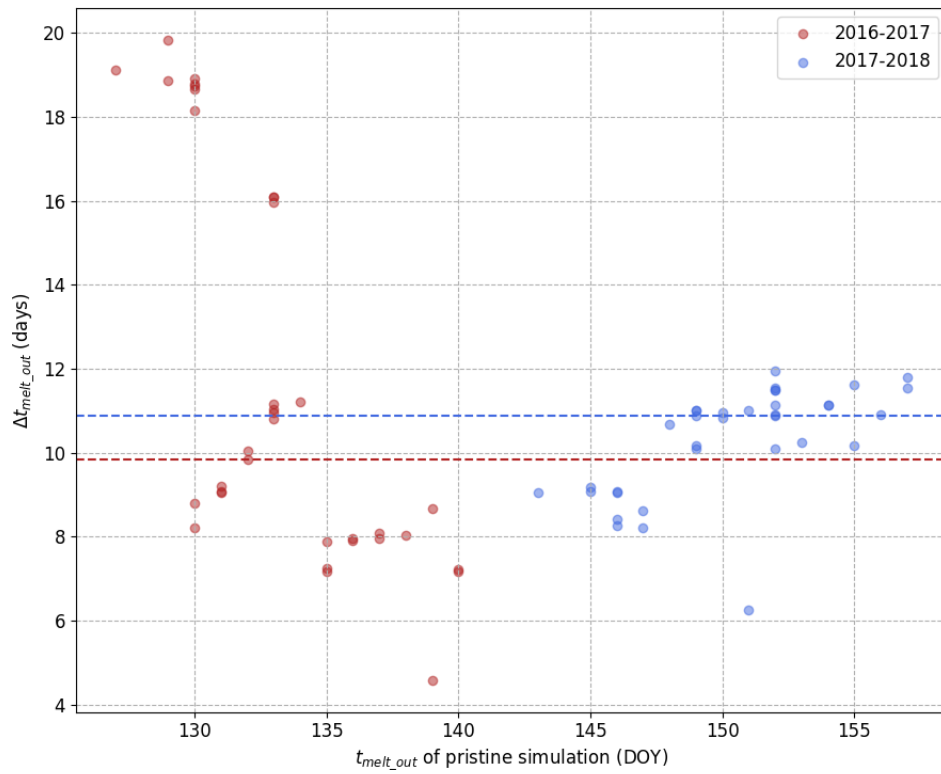
Figure 7. \Delta t_{melt-out} as a function of the date of melt of the pristine simulation for each of the 35 members and each year.
