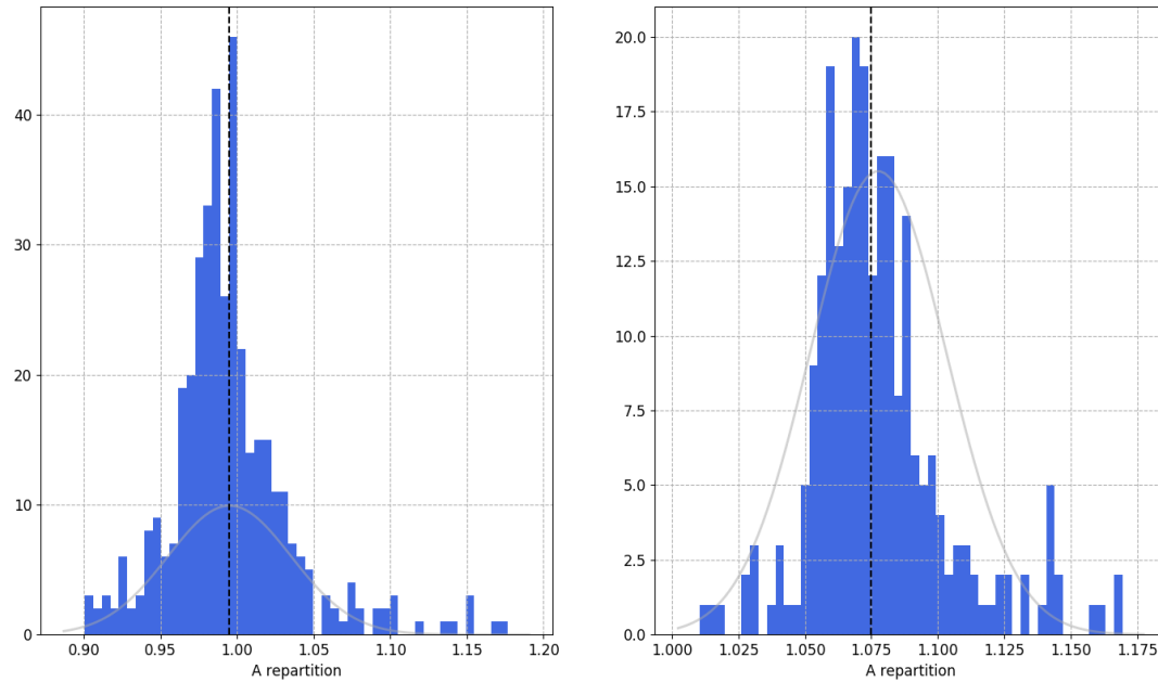
Figure A1. Repartition of the scaling factor of Autosolexs measurements for cloudy days. The difference between both years comes from a change in the instrument setup of Autosolexs for the second year; the lower glass protective shield of the light collector was removed.
