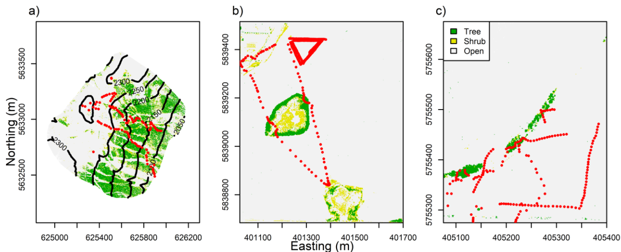
Figure 4: Fortress a), Rosthern b), and Clavet c) study sites classified by vegetation height derived from snow-free (ground) UAV-lidar into open (<0.5 m), shrub (>0.5 m and <2 m) and tree (>2 m) domains. Red points identify locations of manual snow depth survey observations sampled over the course of the data collection campaign. Black lines in Fortress map are 50 m elevation contours.
